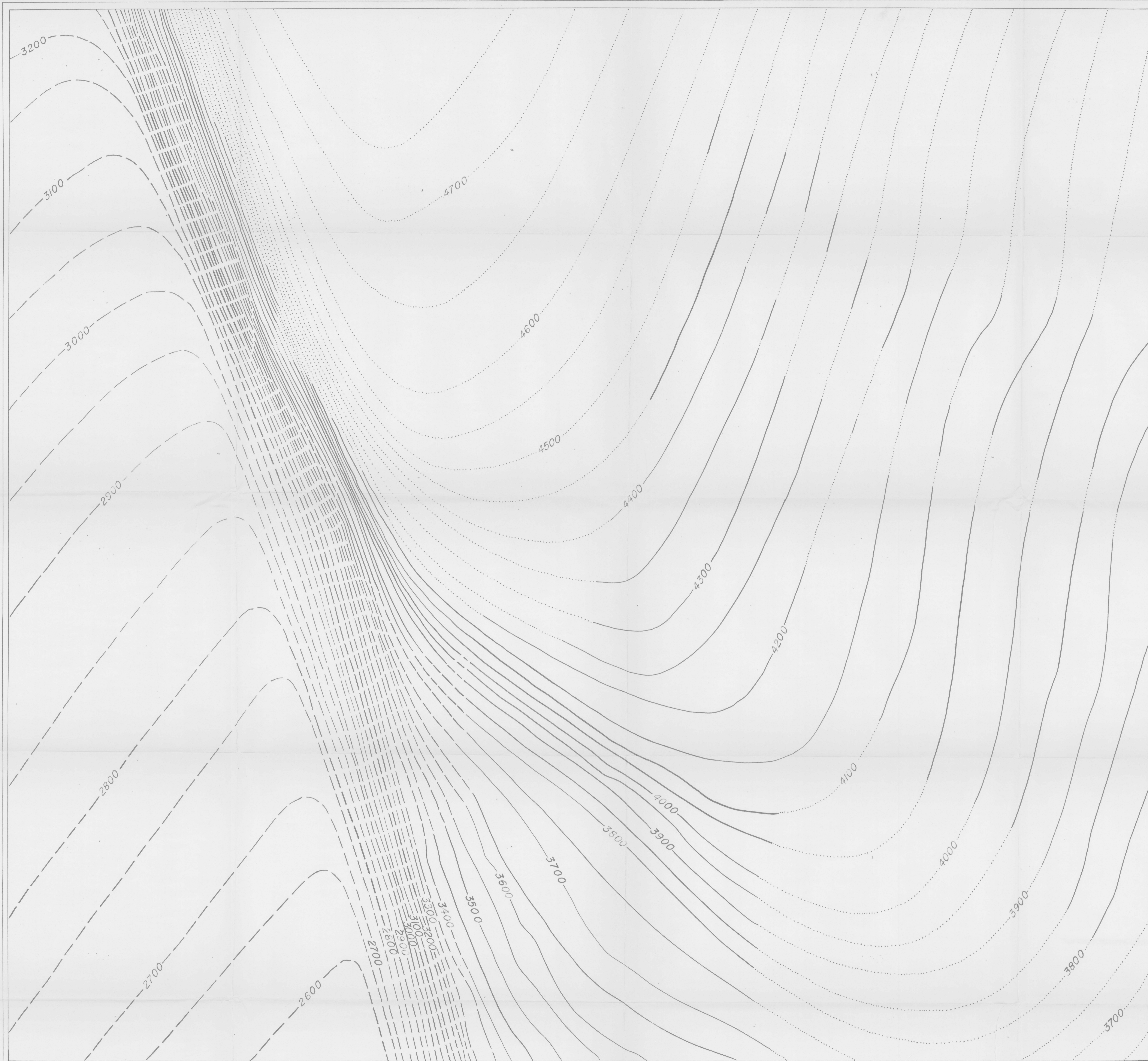
PRELIMINARY STRUCTURE CONTOUR MAP OF THE EAST-CENTRAL PART OF THE CASCADE SPRINGS QUADRANGLE
