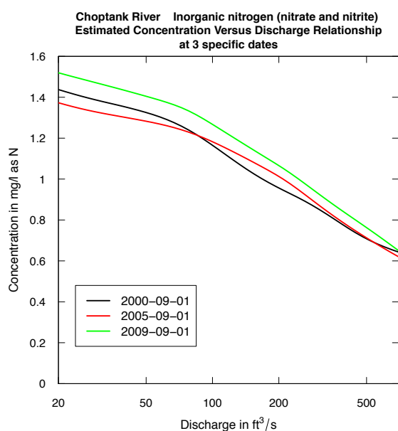
(a) plotConcQSmooth
