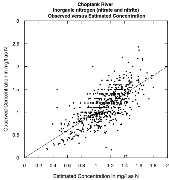
(a) plotConcPred(eList)
