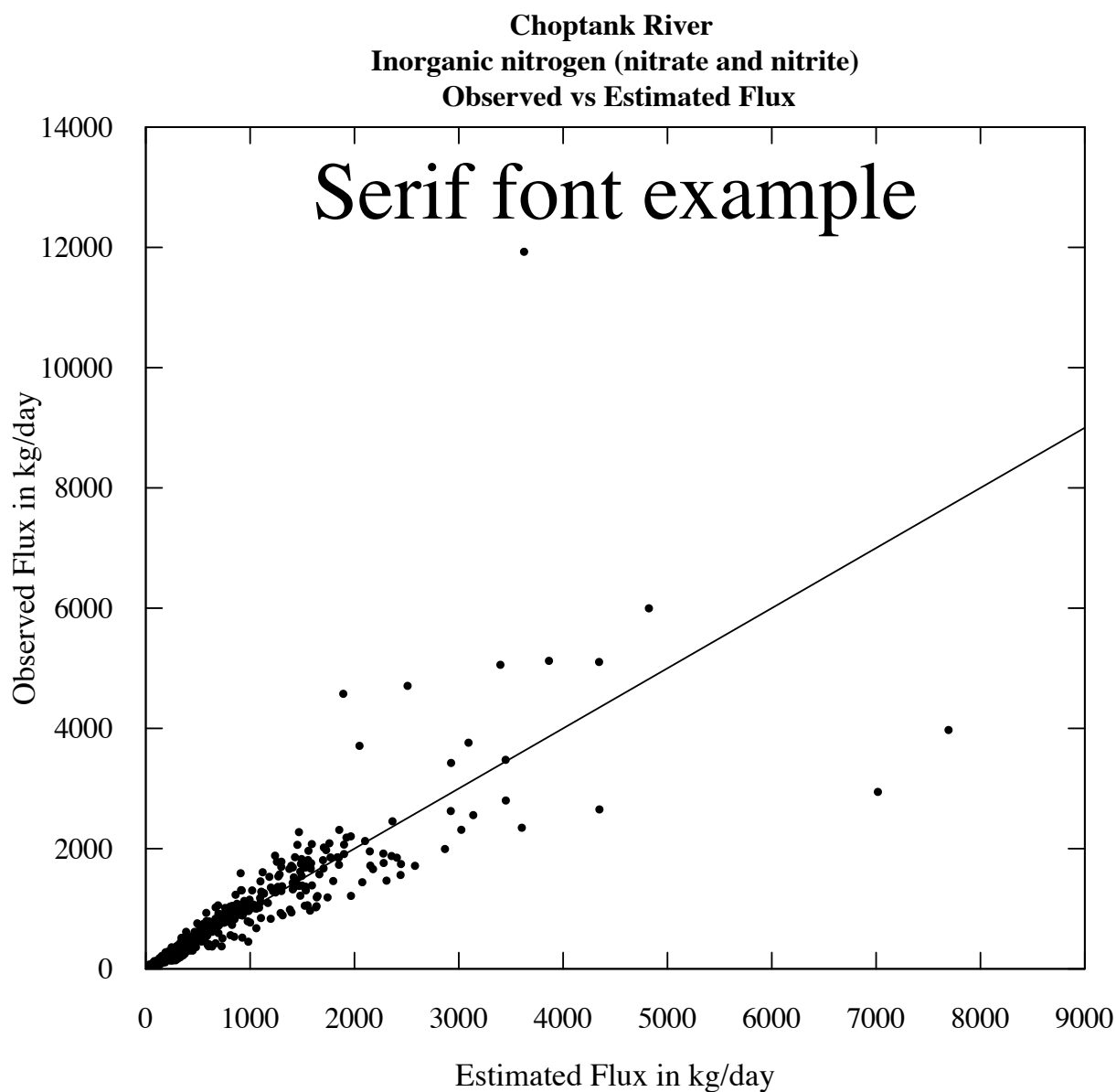
Figure 23. Serif font
