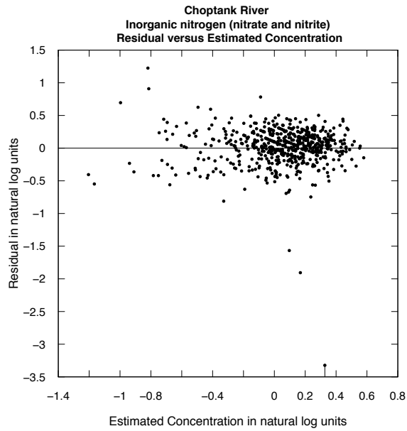
(a) plotResidPred(eList)
