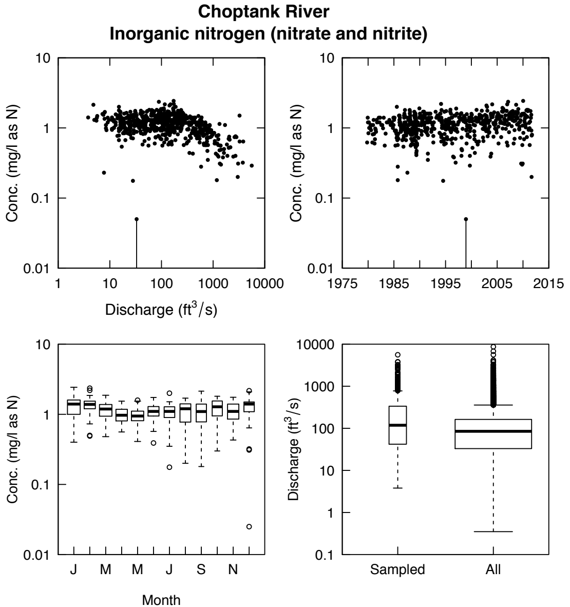
Figure 9. multiPlotDataOverview(eList, qUnit=1)
