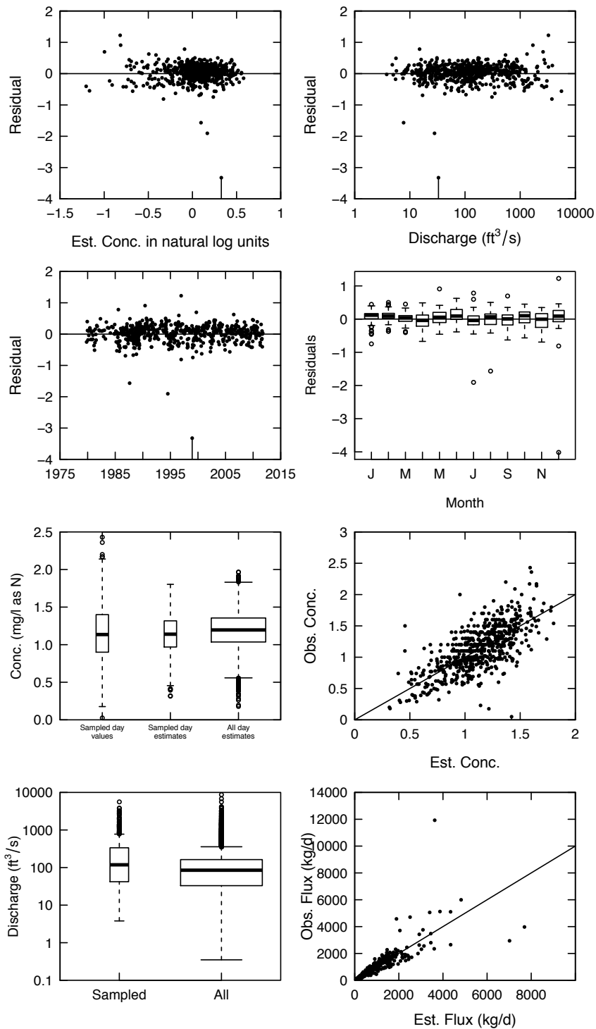
Figure 18. fluxBiasMulti(eList, qUnit=1)
