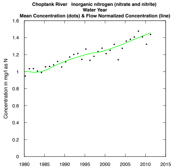
(a) plotConcHist (eList)
