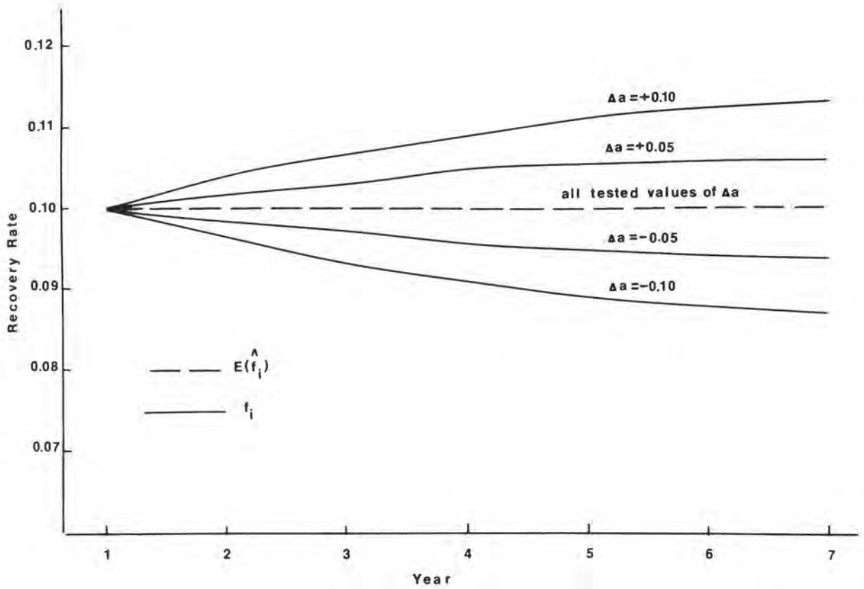
Fig. C-1. E(\hat{f}_i) and true f_i for selected \Delta a .
