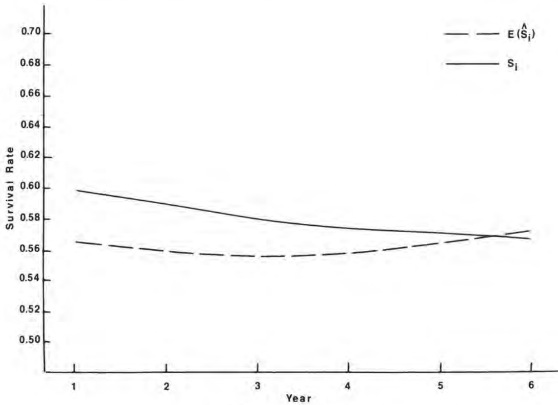
Fig. C-8. E(\hat{S}_i) and true S_i for \Delta b = -0.05 .
