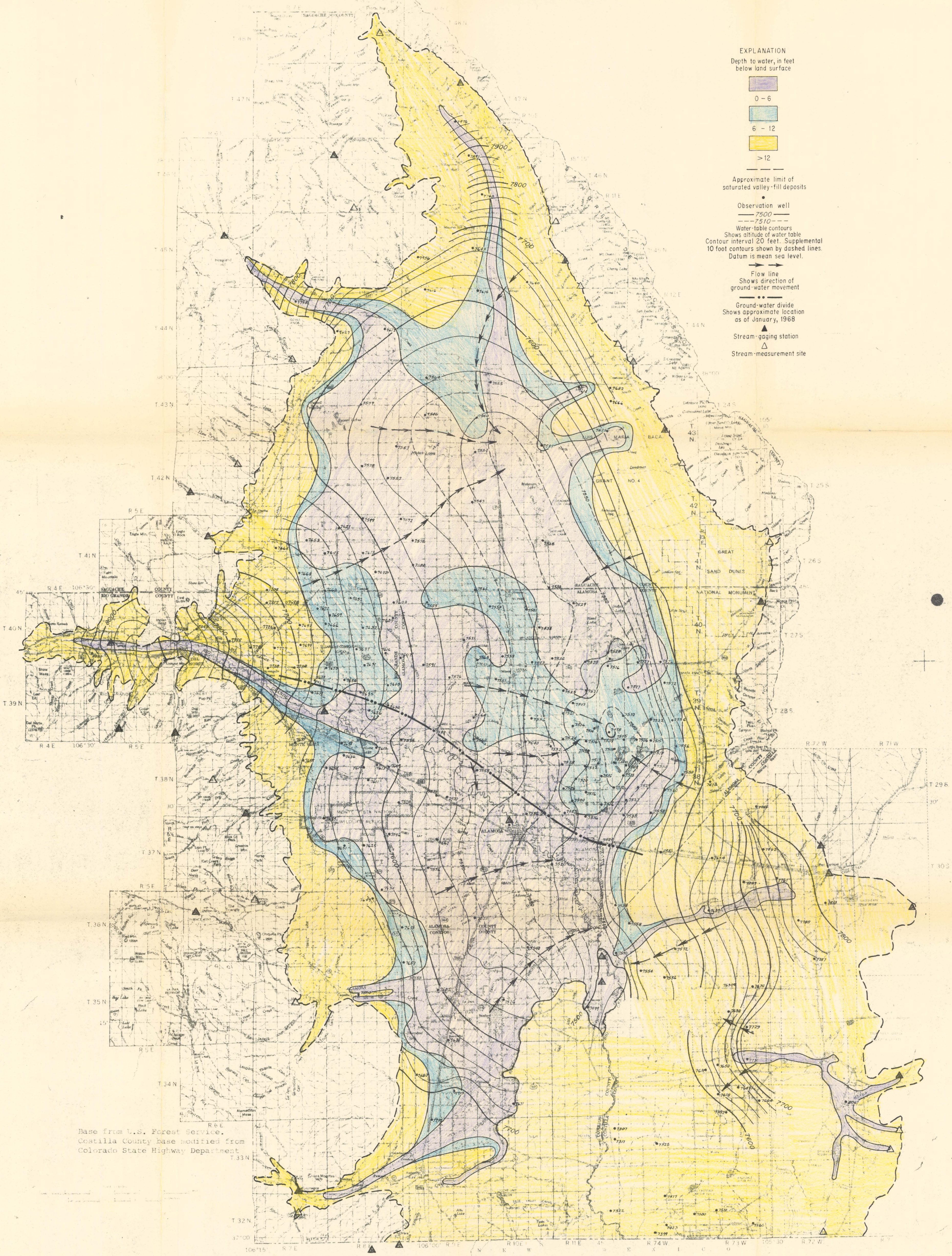
Figure 4. Configuration of water table and depth to water, January 1968.
