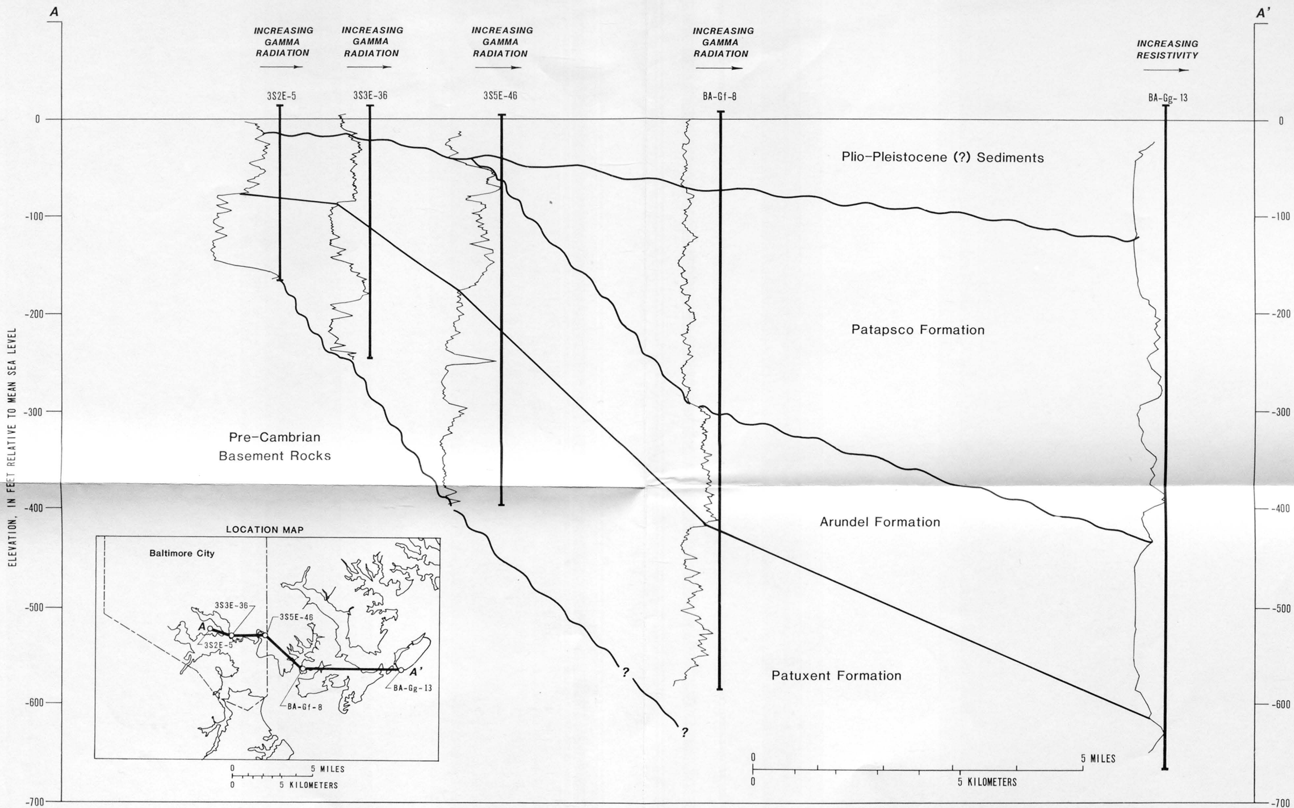
Plate 2.—Cross-section A-A' showing major hydrologic units in the Baltimore, Md., area.
