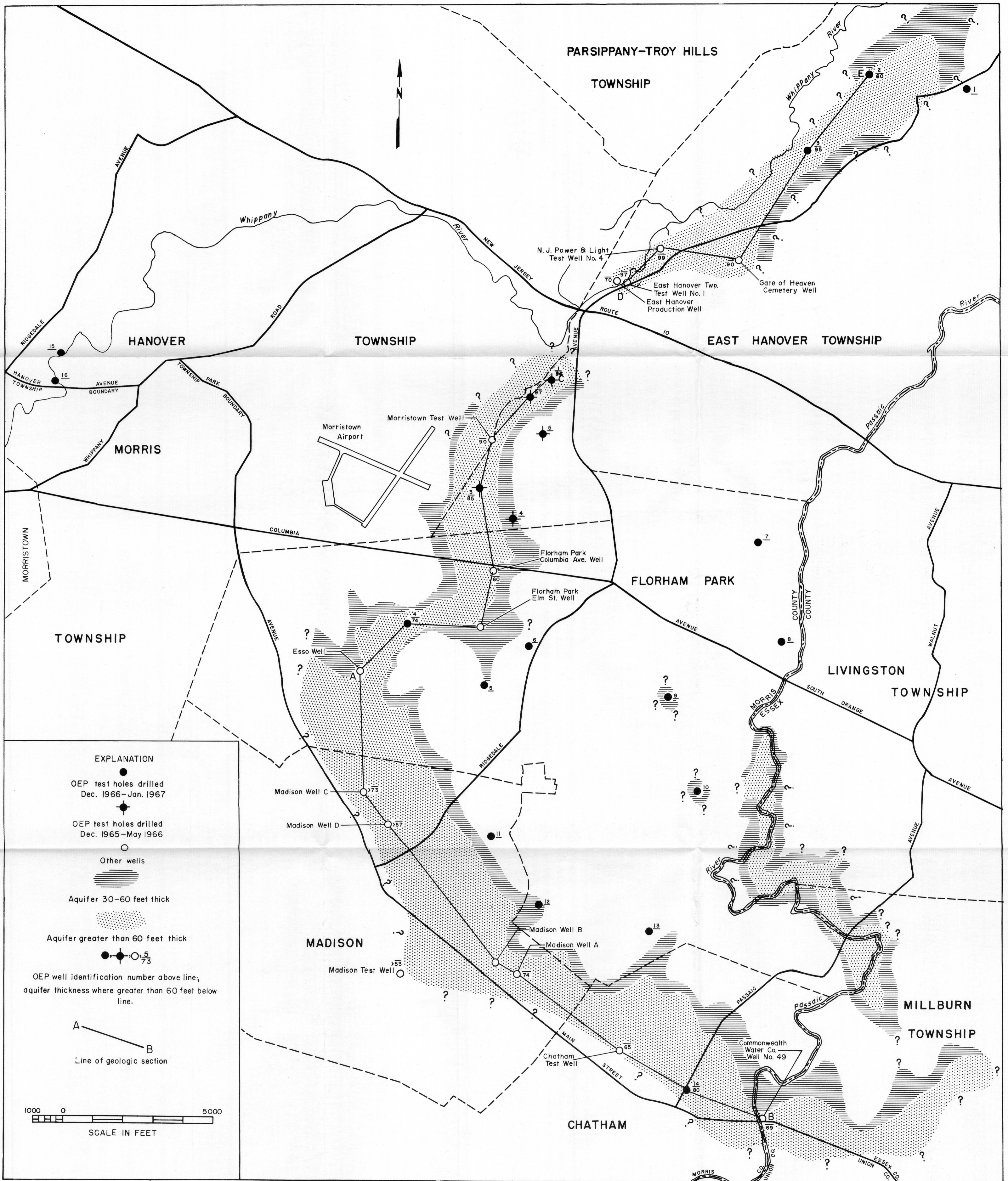
Figure 2.—Location map of OEP test holes showing distribution of valley-fill aquifers where they exceed 30 feet in thickness.
