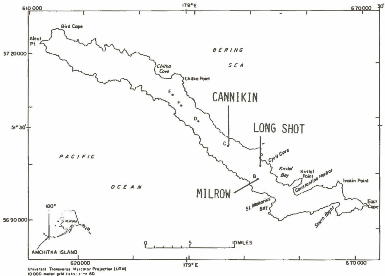
Figure 1.--Amchitka Island, Alaska, showing locations of drill sites B, C, D, E, and F, and the nuclear tests Cannikin, Long Shot, and Milrow.
