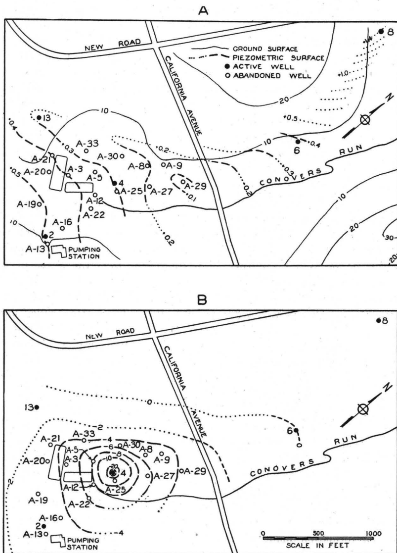
FIGURE 9.—Maps of well field at Atlantic City Water Works, showing the location of wells to the 100-foot sand and indicating by contours the elevation of the ground surface and of the piezometric surface. A, Ground surface and piezometric surface before well 4 was pumped. B, Piezometric surface after well 4 had been pumped 7 days at 1.46 million gallons daily.
