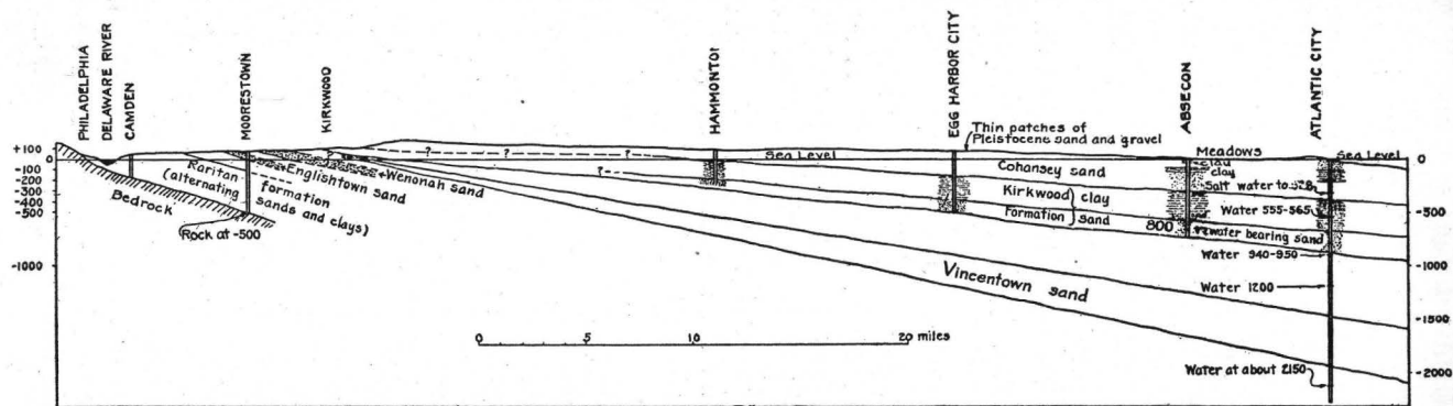
FIGURE 2.—Generalized cross section from Philadelphia to Atlantic City, showing principal water-bearing beds.
