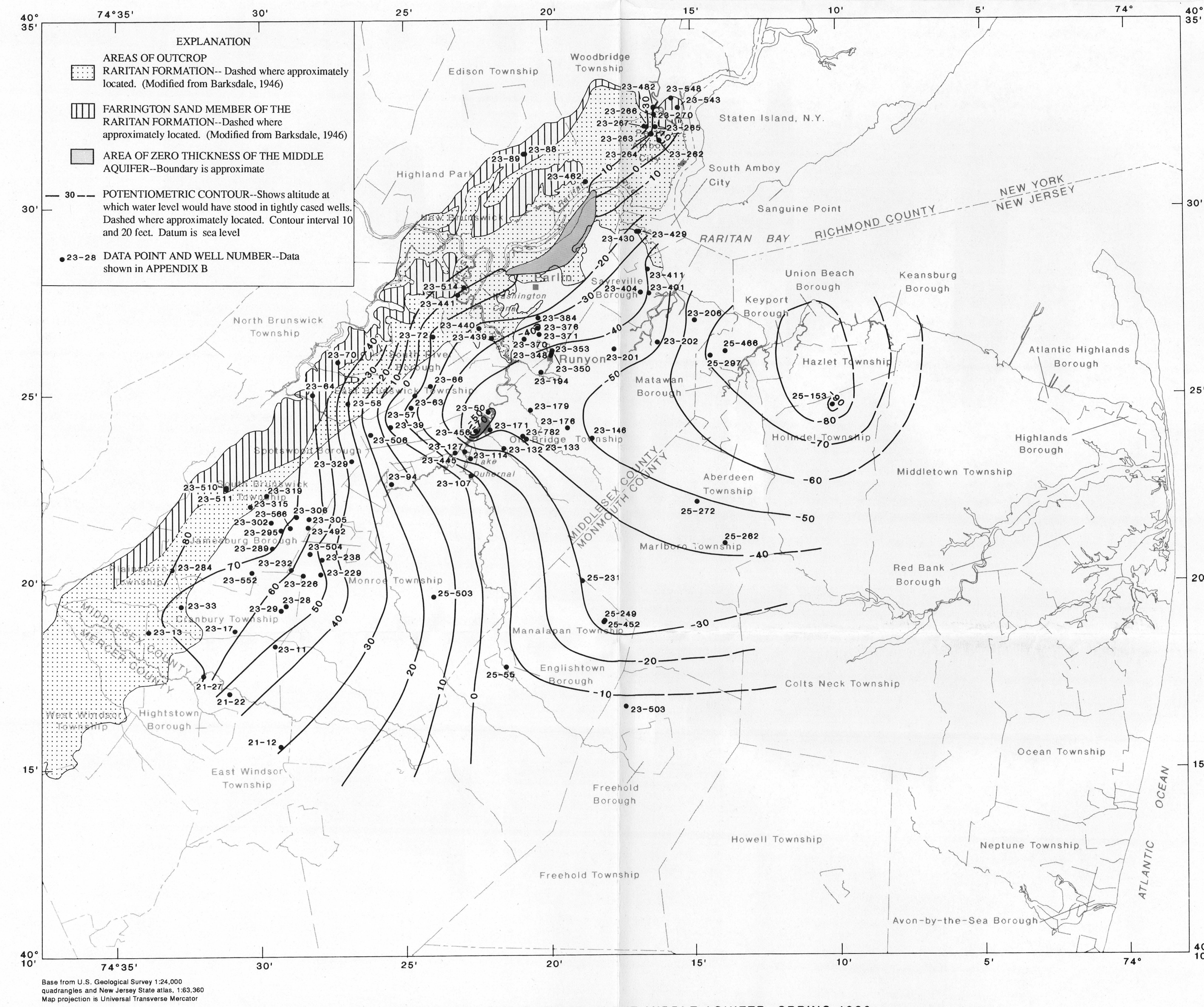
D. POTENTIOMETRIC SURFACE IN THE MIDDLE AQUIFER, SPRING 1986
