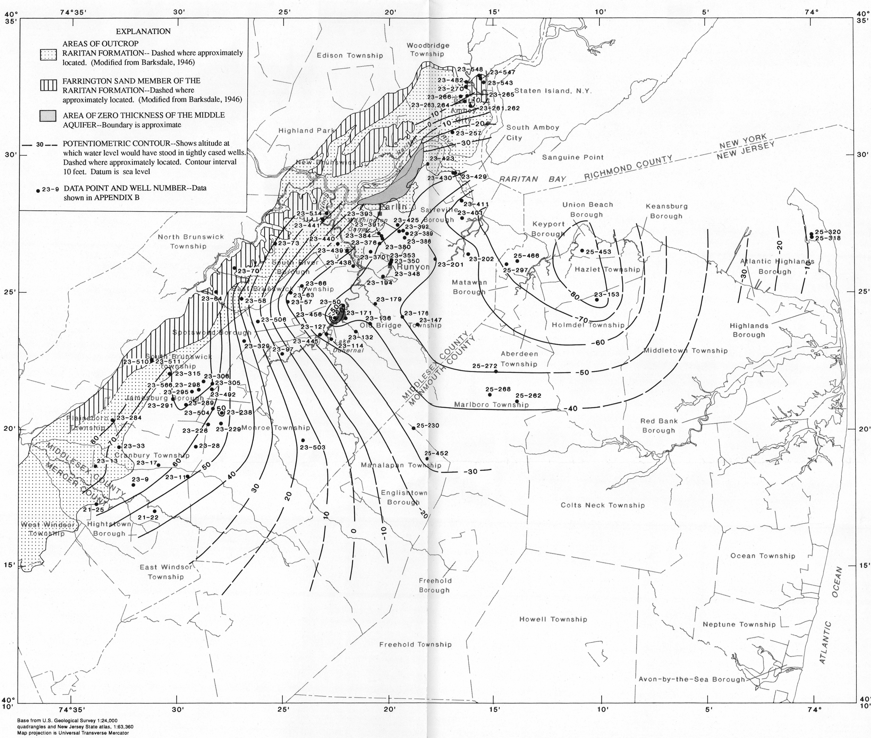
C. POTENTIOMETRIC SURFACE IN THE MIDDLE AQUIFER, FALL 1984
