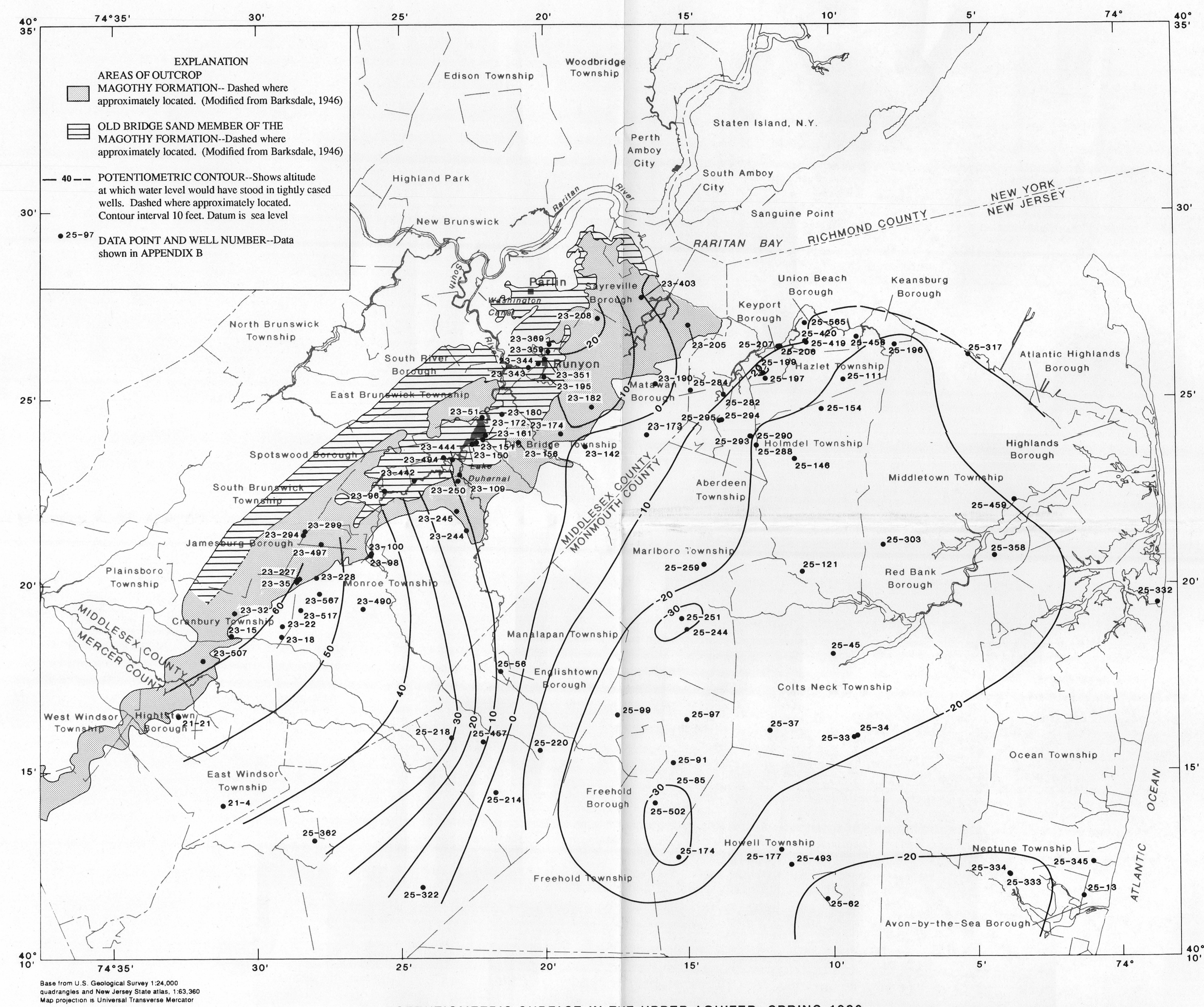
B. POTENTIOMETRIC SURFACE IN THE UPPER AQUIFER, SPRING 1986
