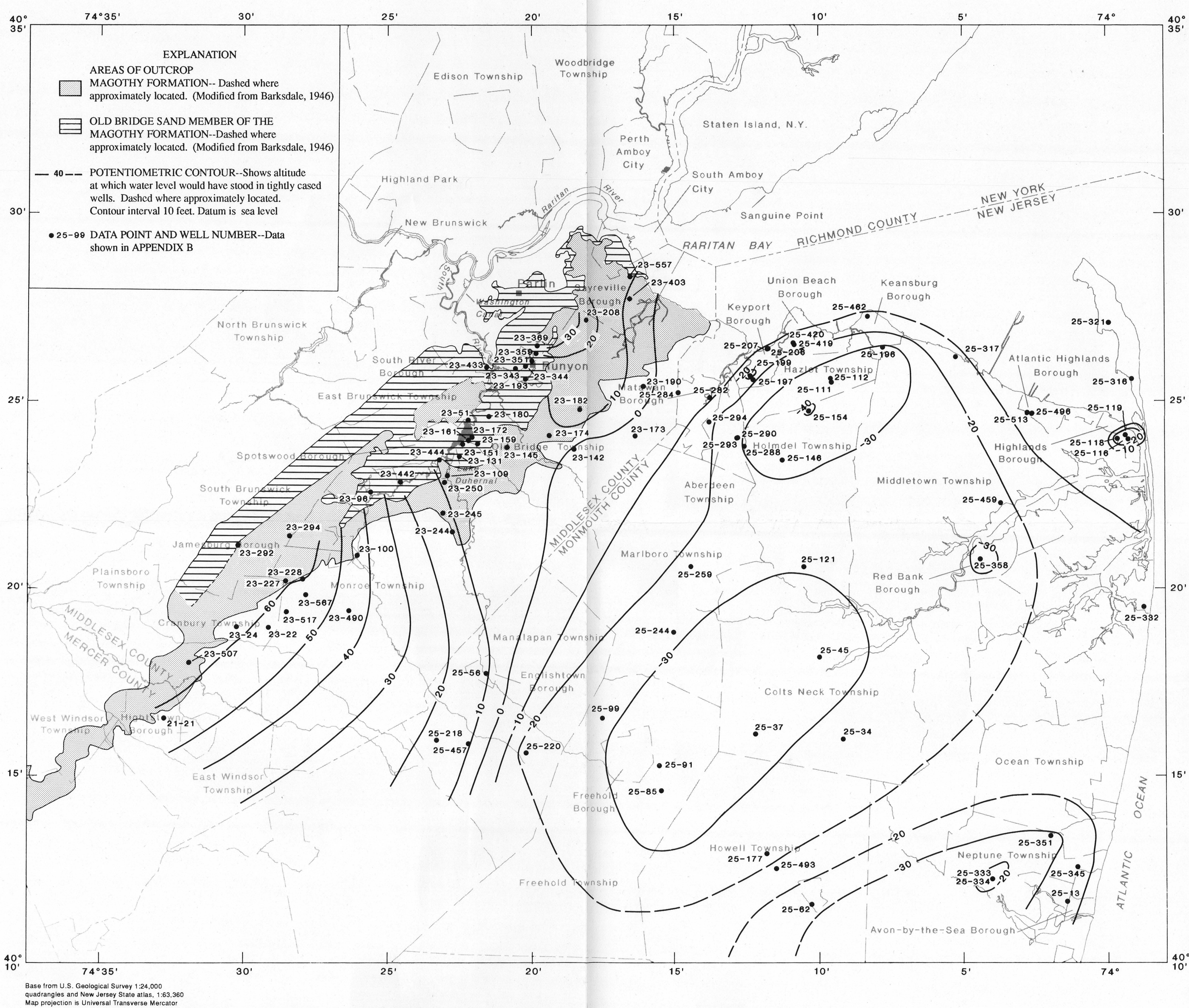
A. POTENTIOMETRIC SURFACE IN THE UPPER AQUIFER, FALL 1984
