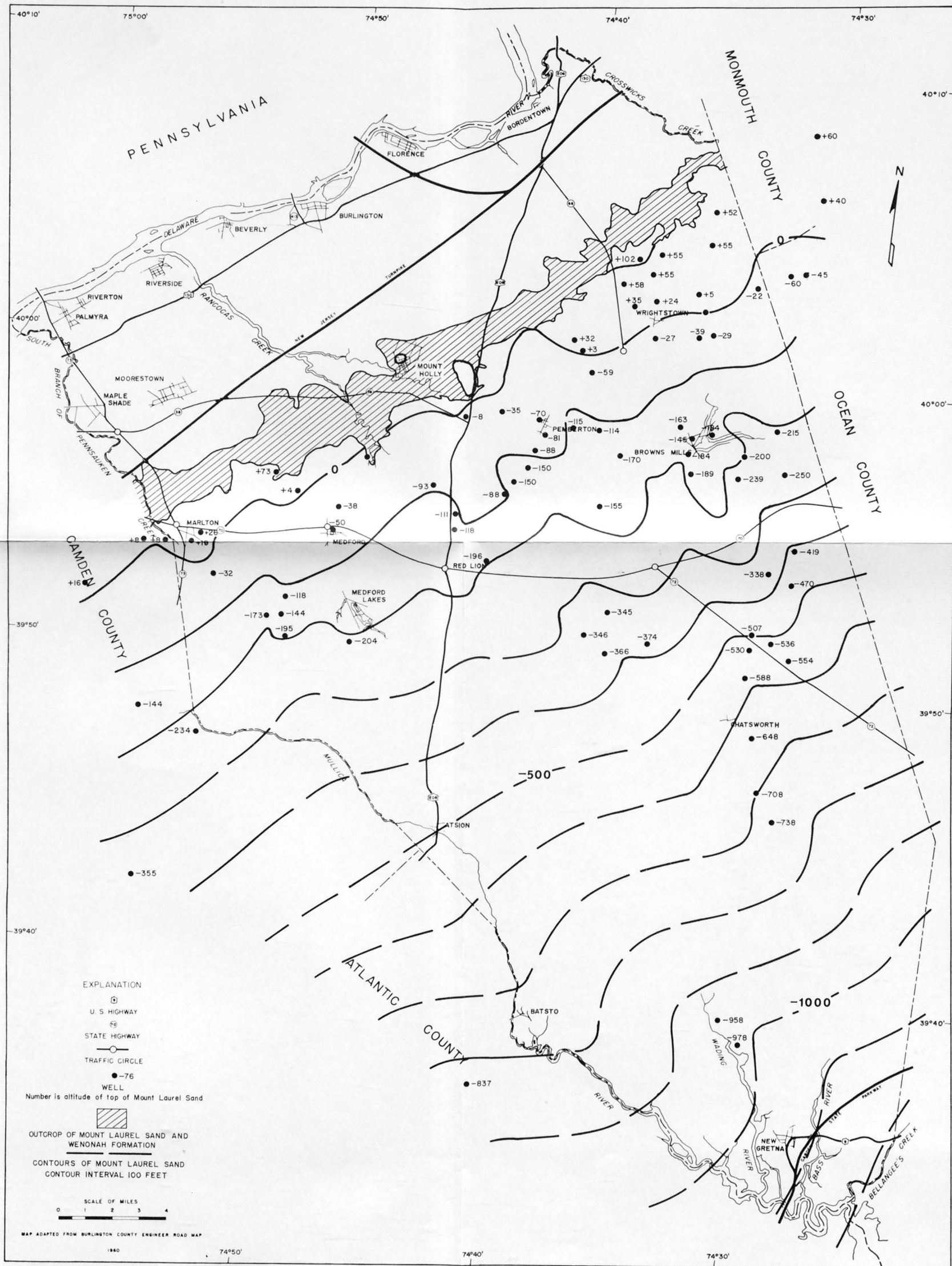
Figure 10.—Structural contour map of the top of the Mount Laurel Sand in Burlington County, N. J.
