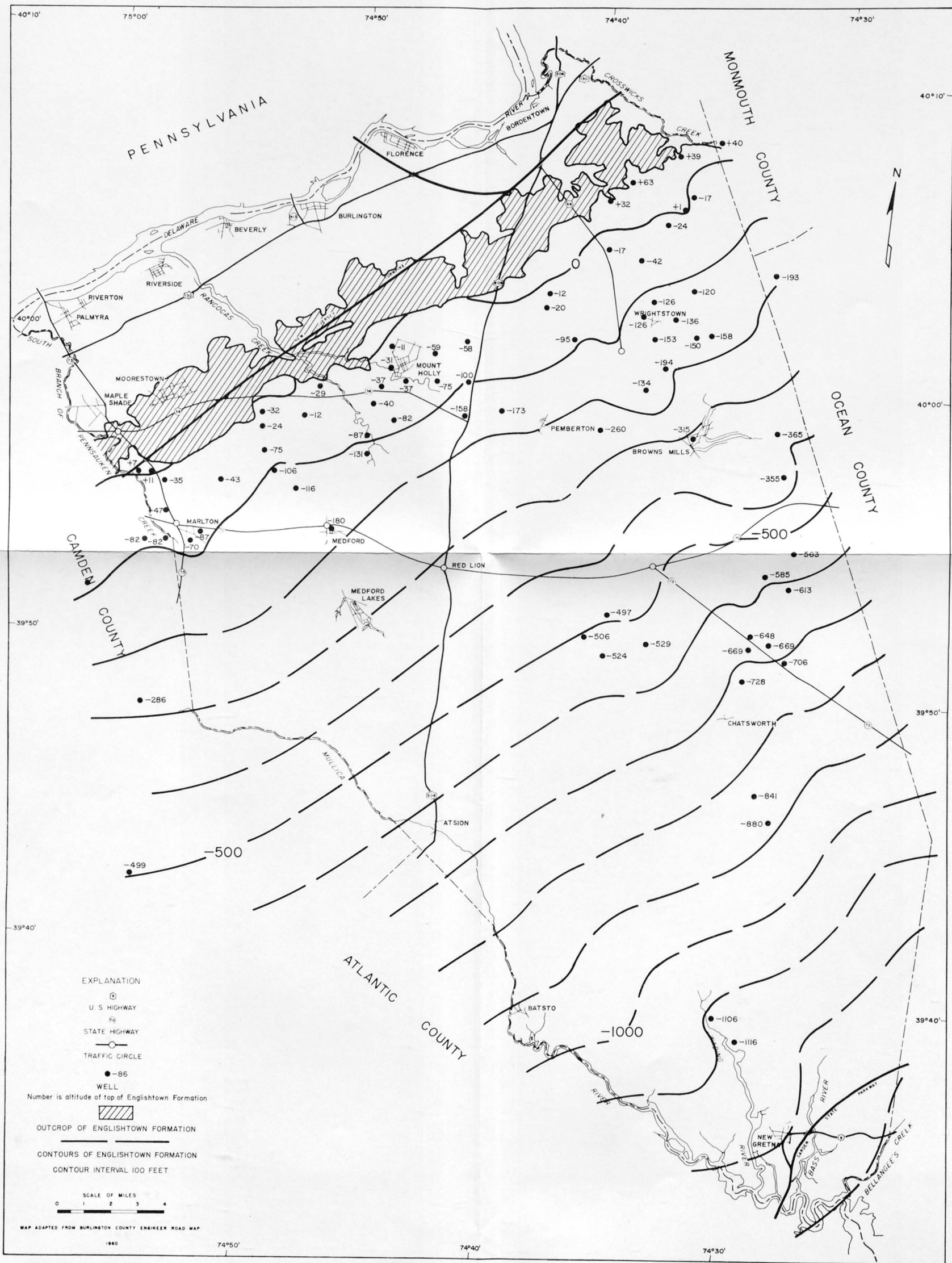
Figure 9.—Structural contour map of the top of the Englishtown Formation in Burlington County, N. J.
