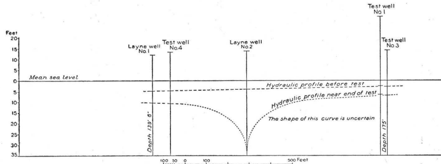
FIG. 5.—Hydraulic profile in the Puchack well field at the beginning and near the end of pumping test of well No. 2, April 3, 1924.
