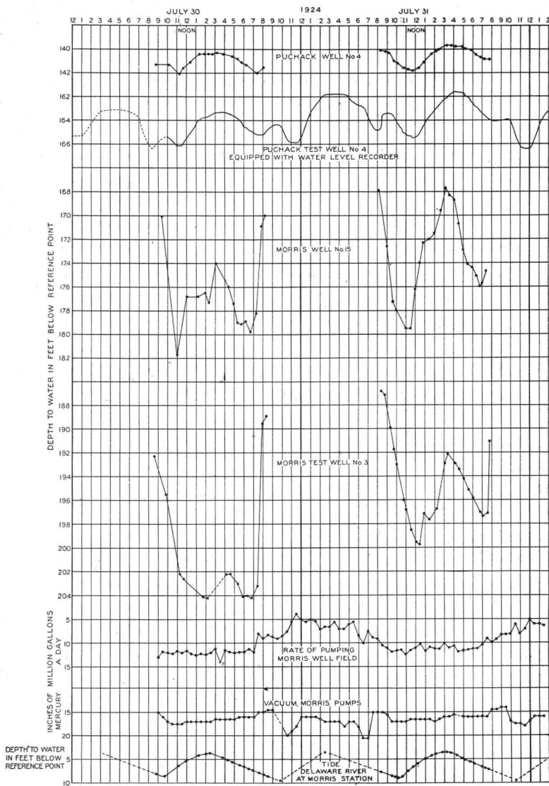
FIG. 8.—Graph showing movement of water levels in observation wells in the Puchack and Morris fields, rate of pumping and vacuum at the Morris plant, and tide level in Delaware River, July 30 and 31, 1924.
