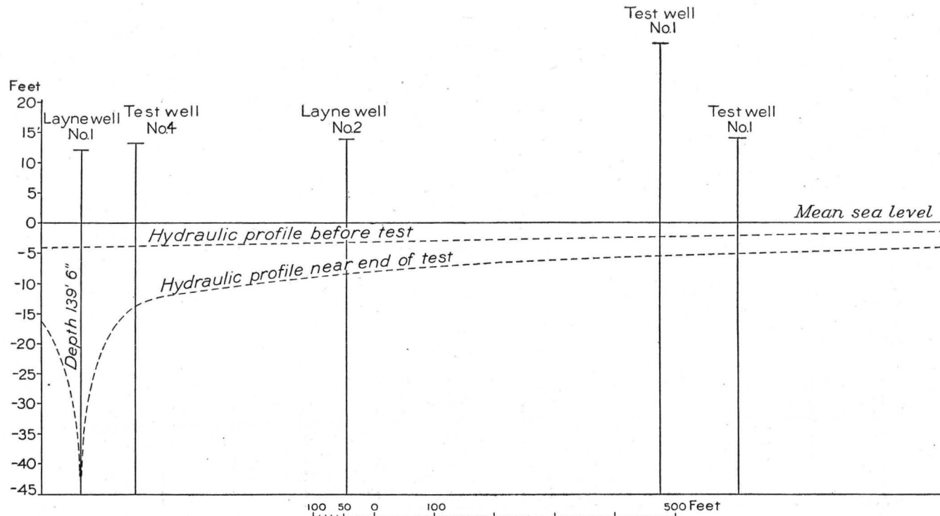
FIG. 3—Hydraulic profiles in the Puchack well field at the beginning and near the end of the pumping test of well No. 1, March 27, 1924.
