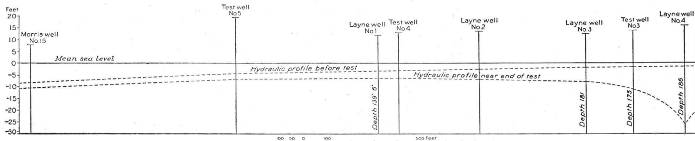
FIG. 6.—Hydraulic profiles in the Puchack field at the beginning and near the end of pumping test of well No. 4, May 10, 1924.
