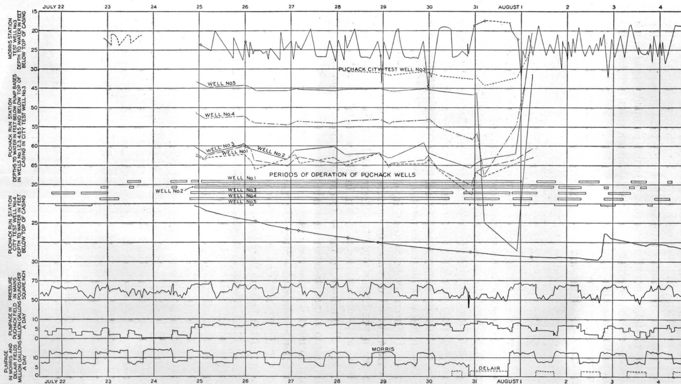
FIG. 12.—Graph showing movements of water levels in observation wells, rate of pumping, pressure in distribution main, and hours of operation of wells in the Puchack, Morris and Delair fields, July 22 to August 4, 1927.
