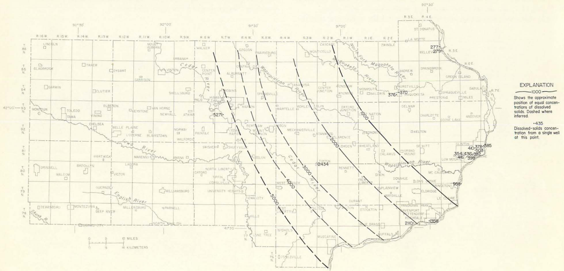
Figure 61.—Dissolved-solids concentrations in the Dresbach aquifer
