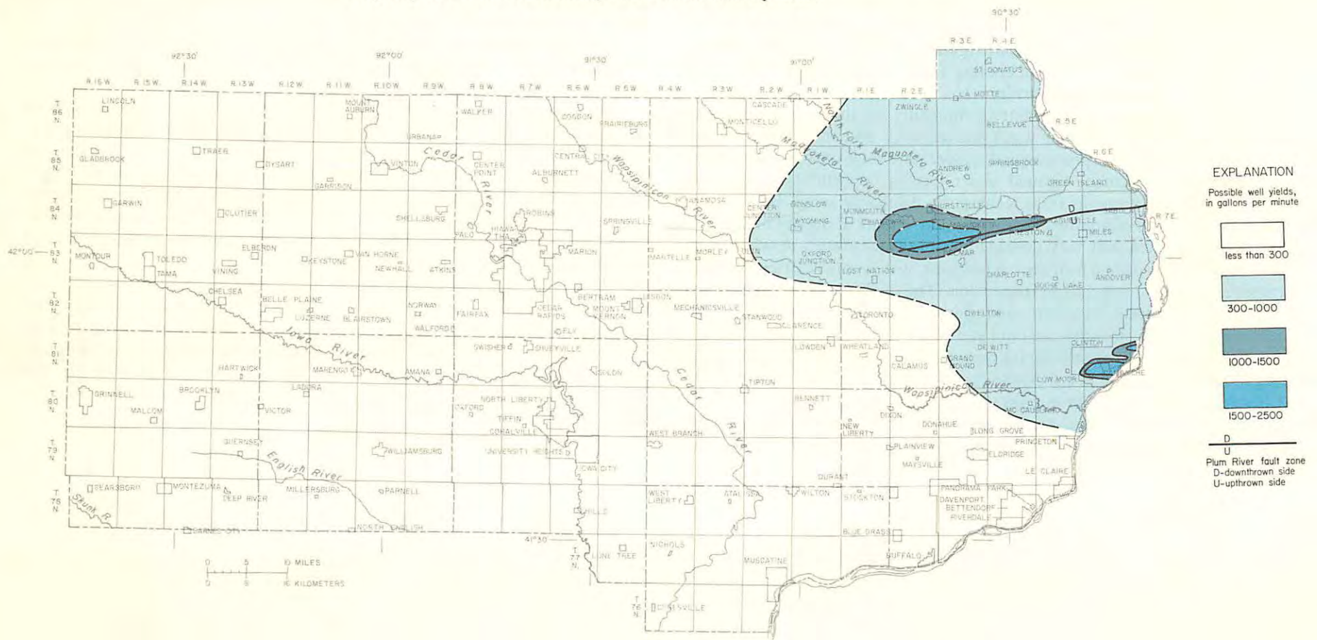
Figure 54.—Possible yields to individual wells; Dresbach aquifer
