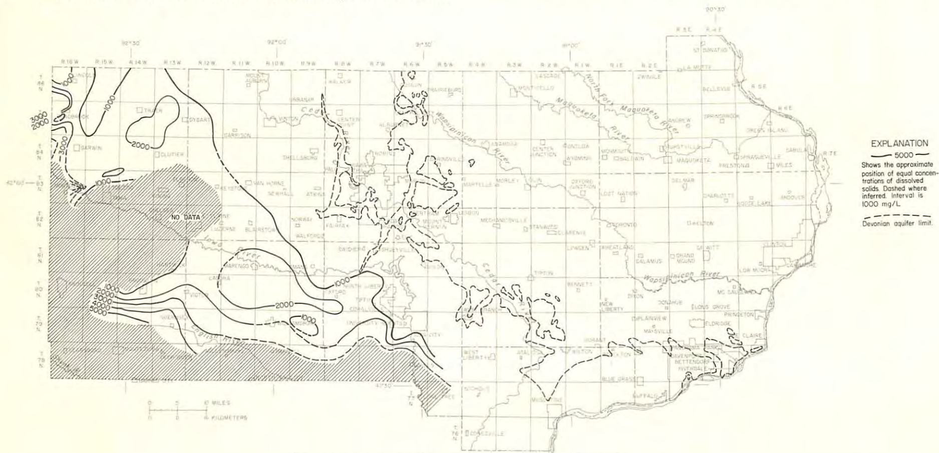
Figure 58.—Dissolved-solids concentrations in the Devonian aquifer
