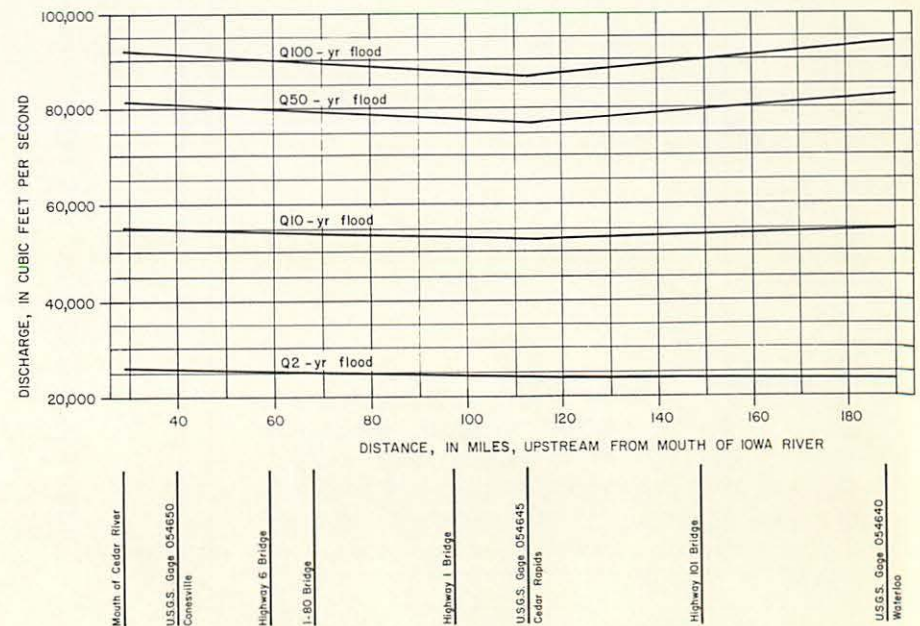
Figure 19.—Peak discharge for indicated recurrence interval for the main stem of Cedar River (from Lara, 1973)
