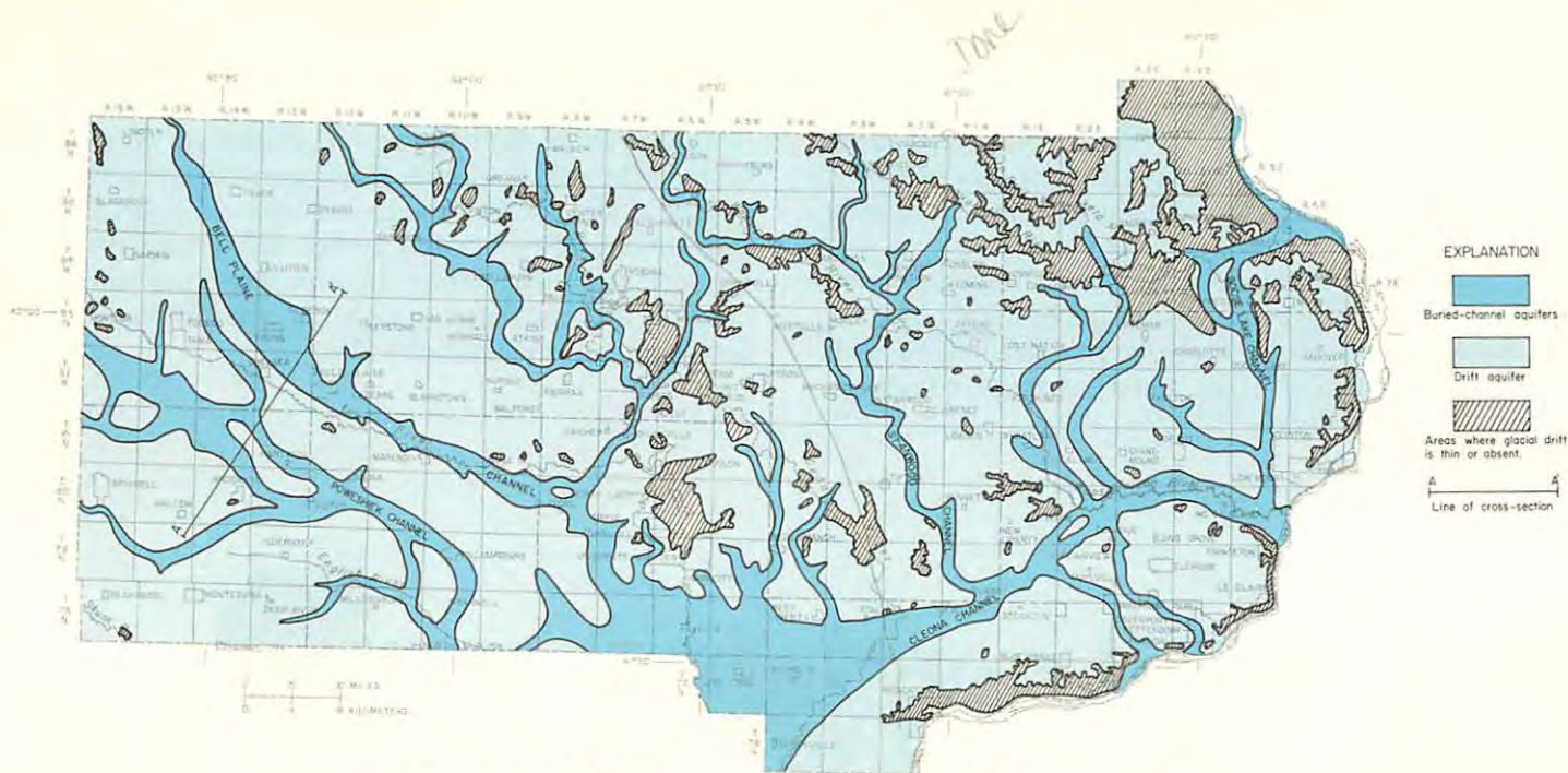
Figure 23.—Areal distribution of buried-channel and drift aquifers
