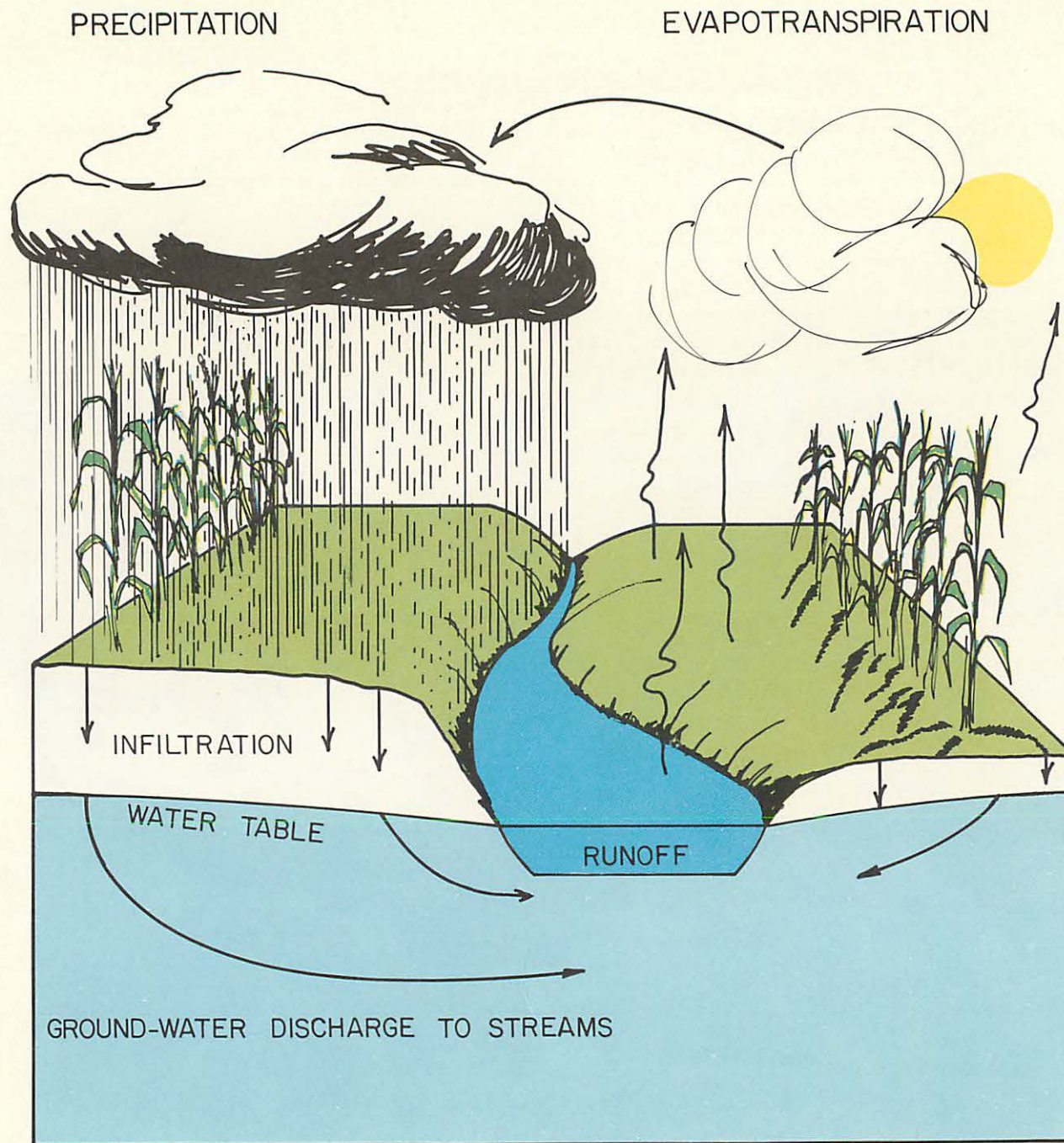
Figure 6.—The hydrologic cycle
