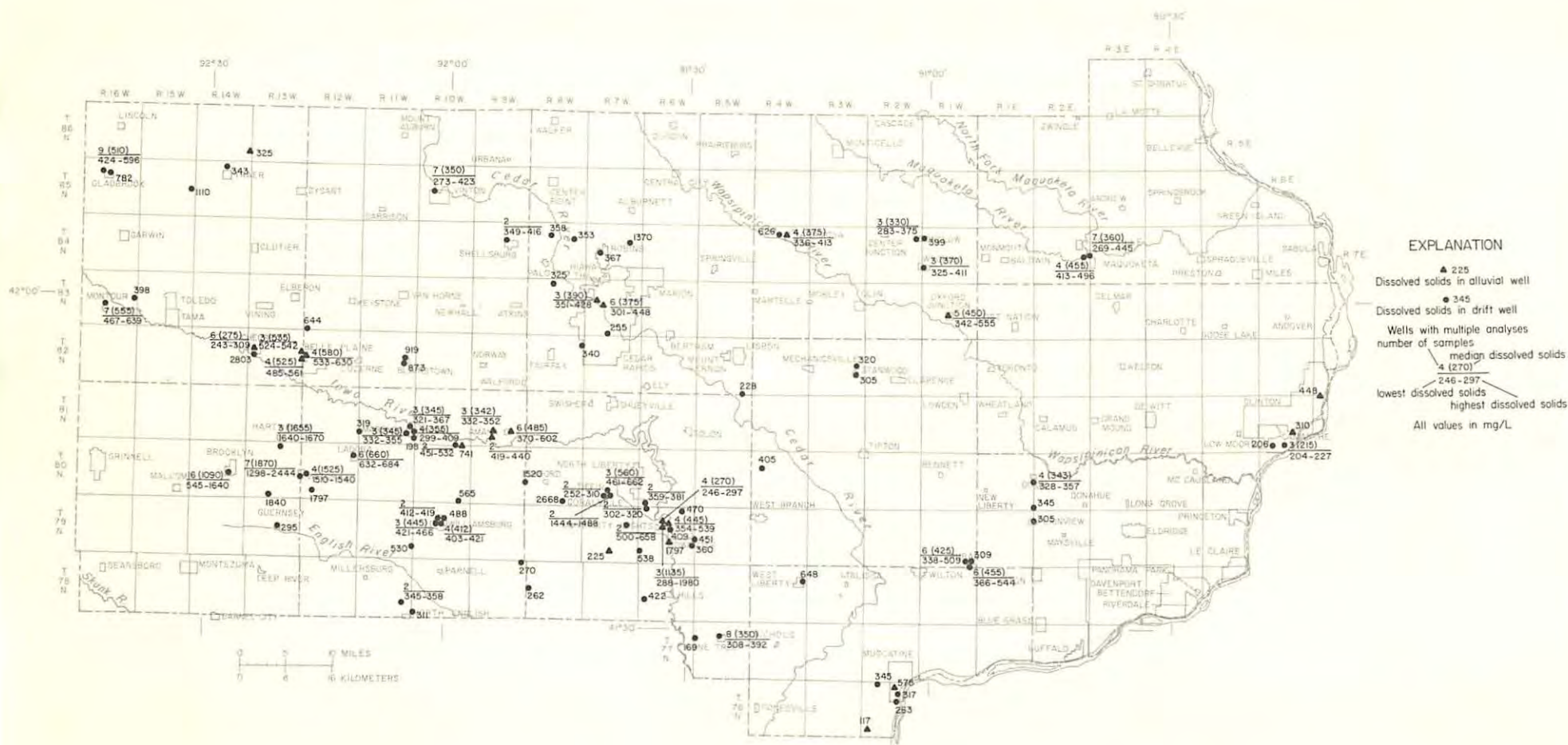
Figure 56.—Dissolved-solids concentrations in the surficial aquifer
