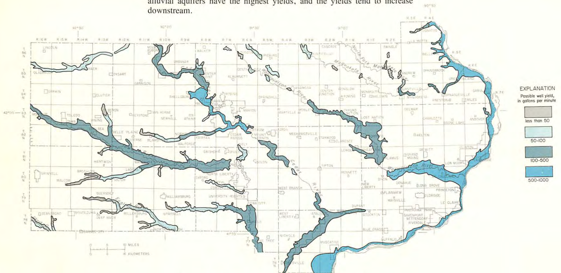
Figure 48.—Possible yields to individual wells; alluvial aquifers
