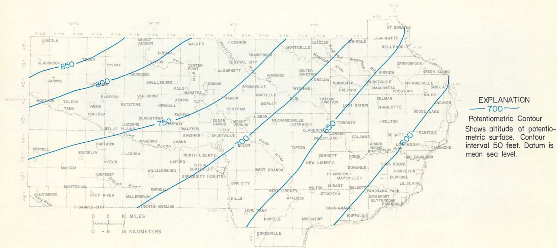
Figure 46.—Potentiometric surface of the Cambrian-Ordovician aquifer before extensive withdrawals began
