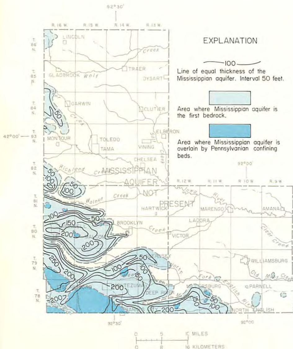
Figure 34.—Thickness of the Mississippian aquifer
