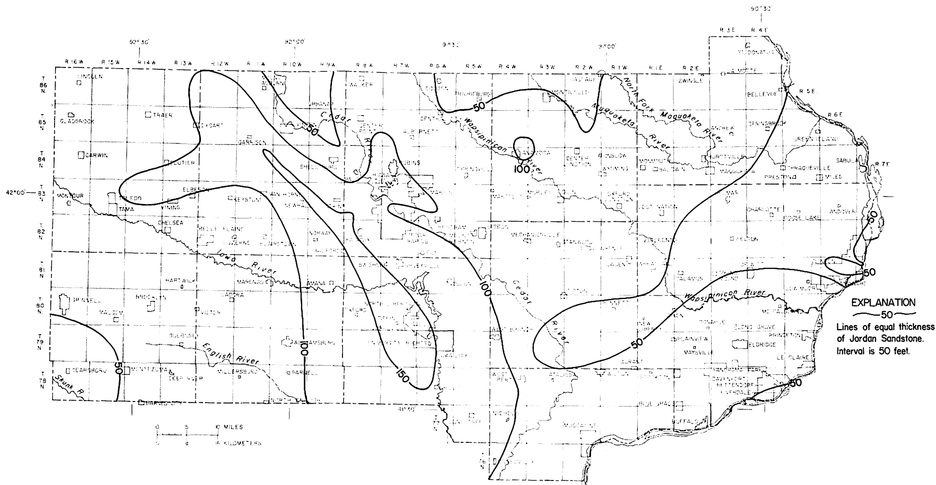
Figure 38.—Thickness of the Jordan Sandstone
