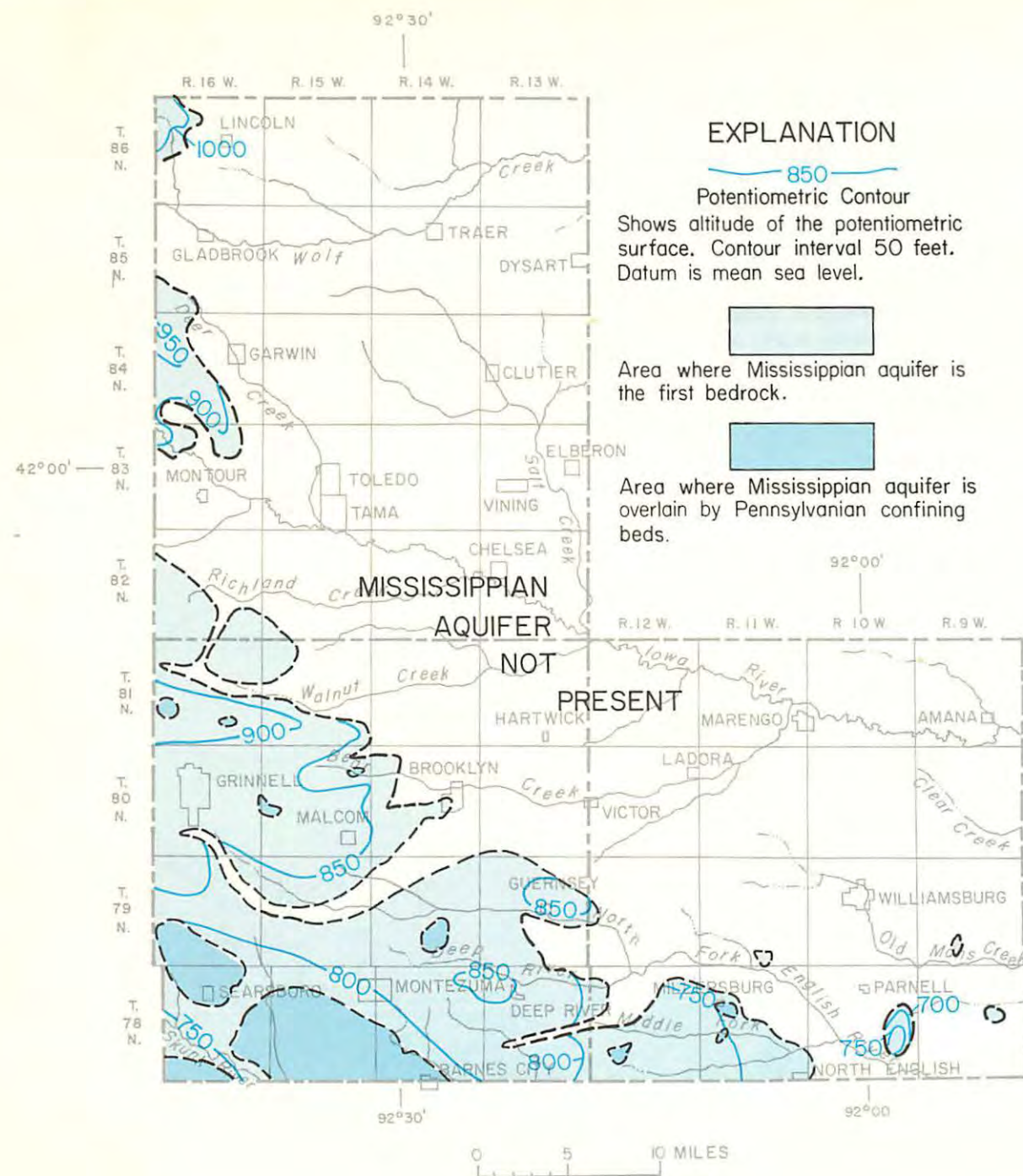
Figure 43.—Potentiometric surface of the Mississippian aquifer
