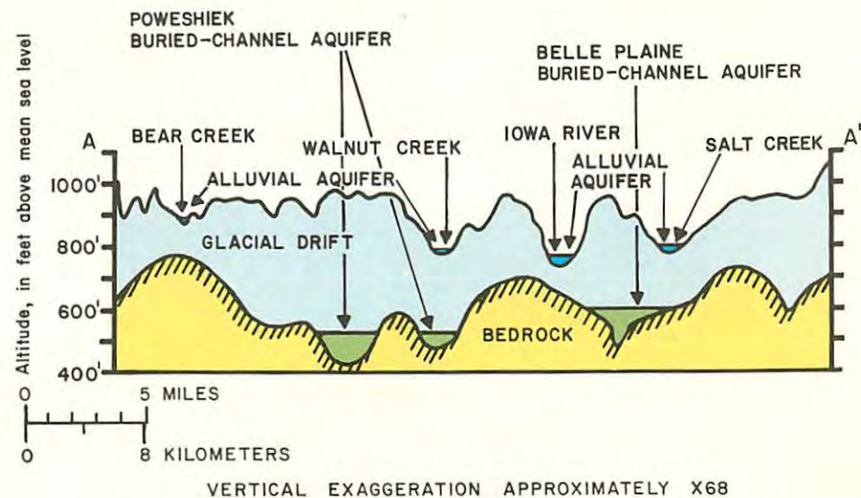
Figure 24.—Hydrogeologic cross section of surficial aquifers
