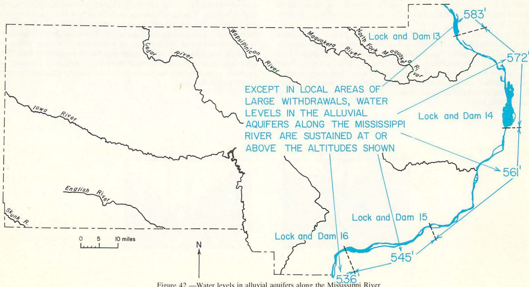
Figure 42.—Water levels in alluvial aquifers along the Mississippi River
