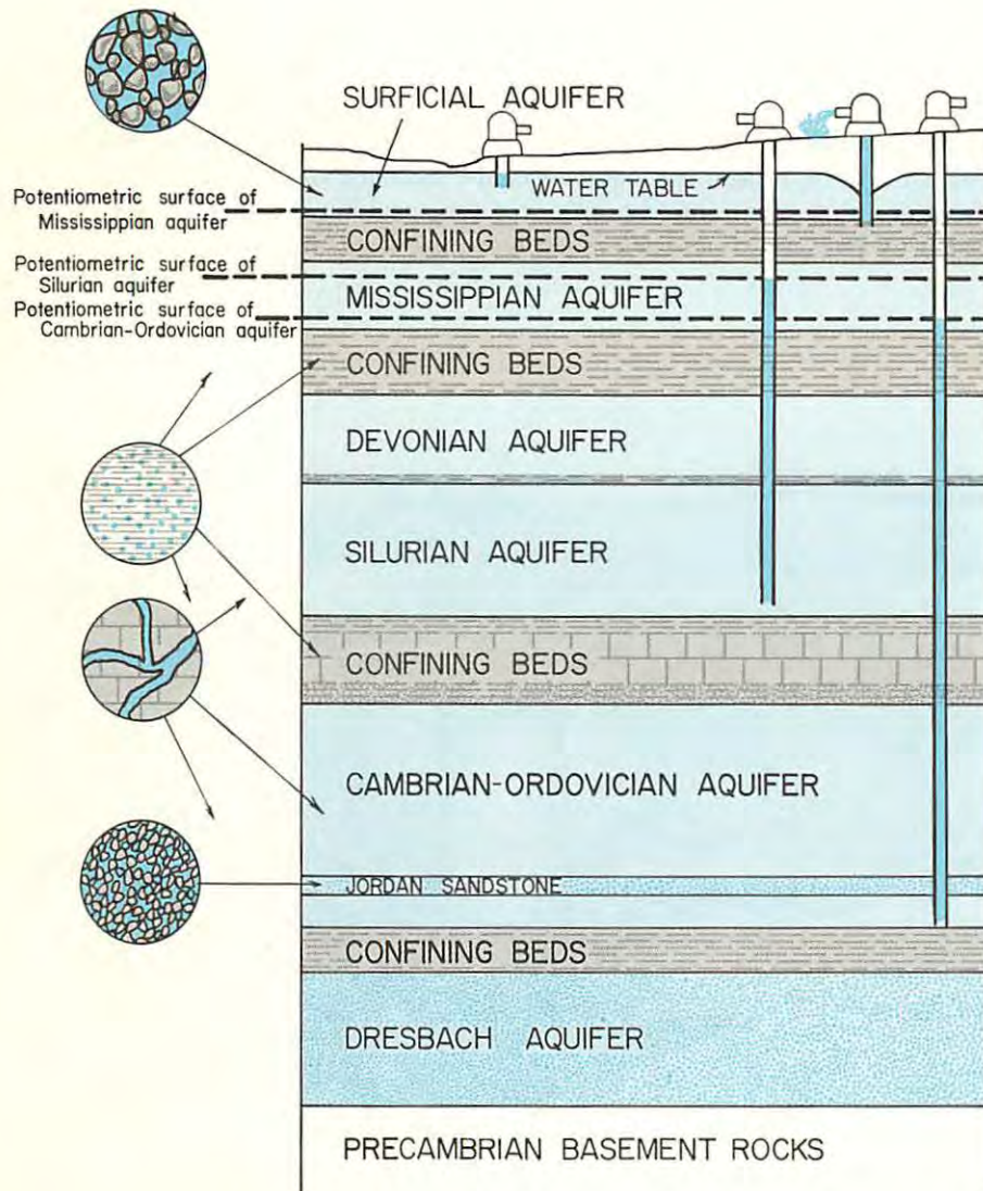
Figure 40.—Occurrence of water in the aquifers
