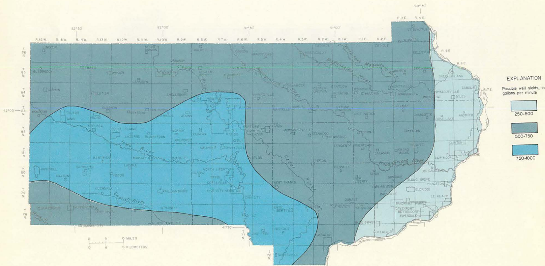
Figure 53.—Possible yields to individual wells; Cambrian-Ordovician aquifer
