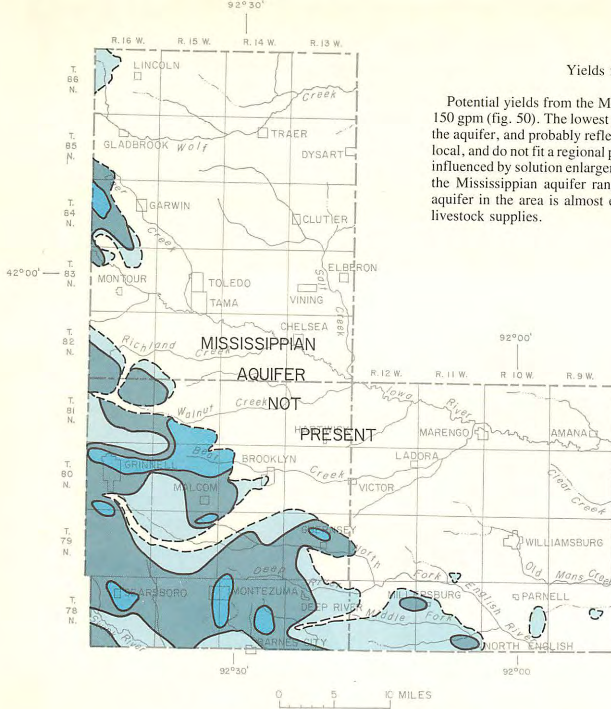
Figure 50.—Possible yields to individual wells; Mississippian aquifer
