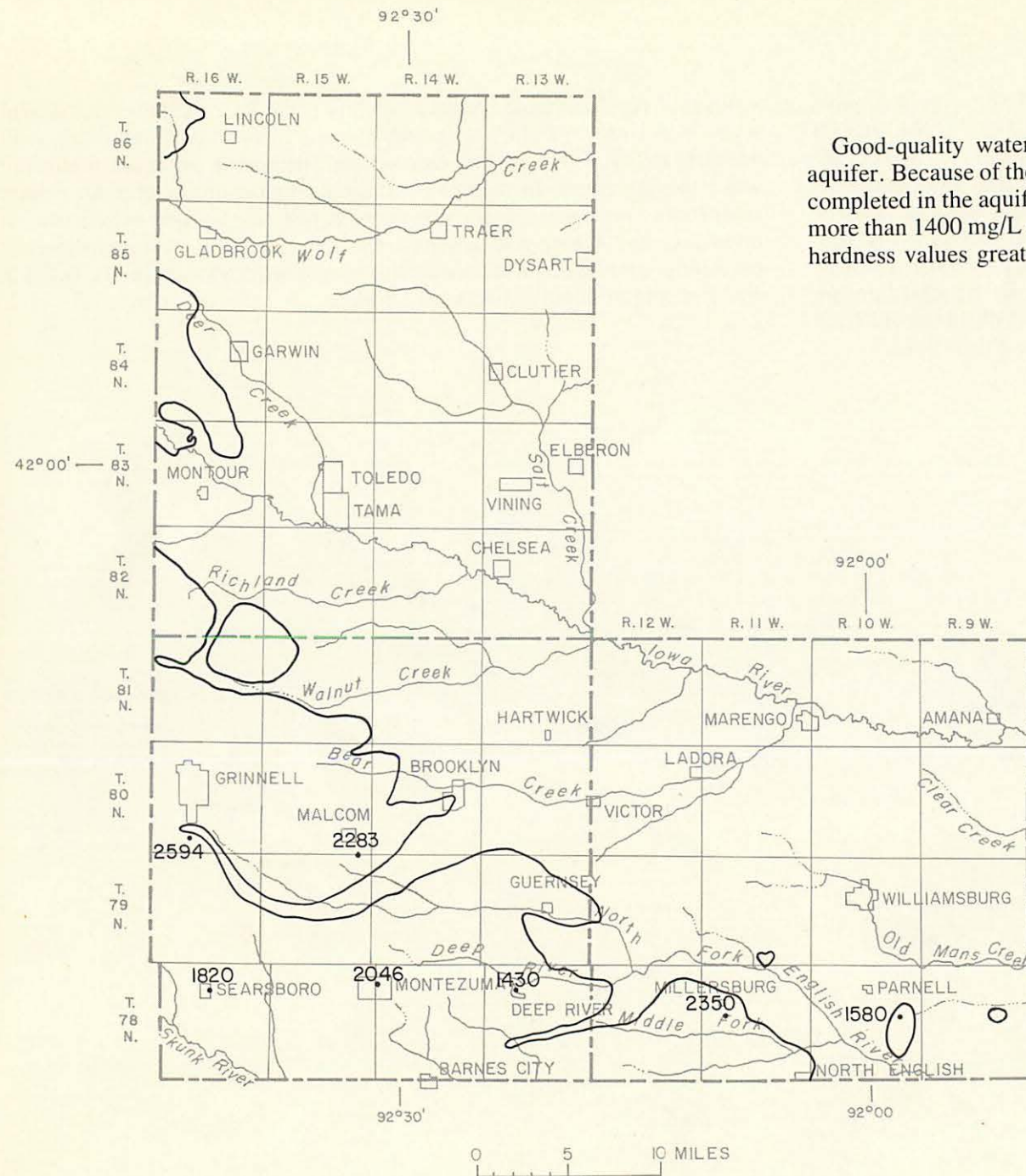
Figure 57.—Dissolved-solids concentrations in the Mississippian aquifer
