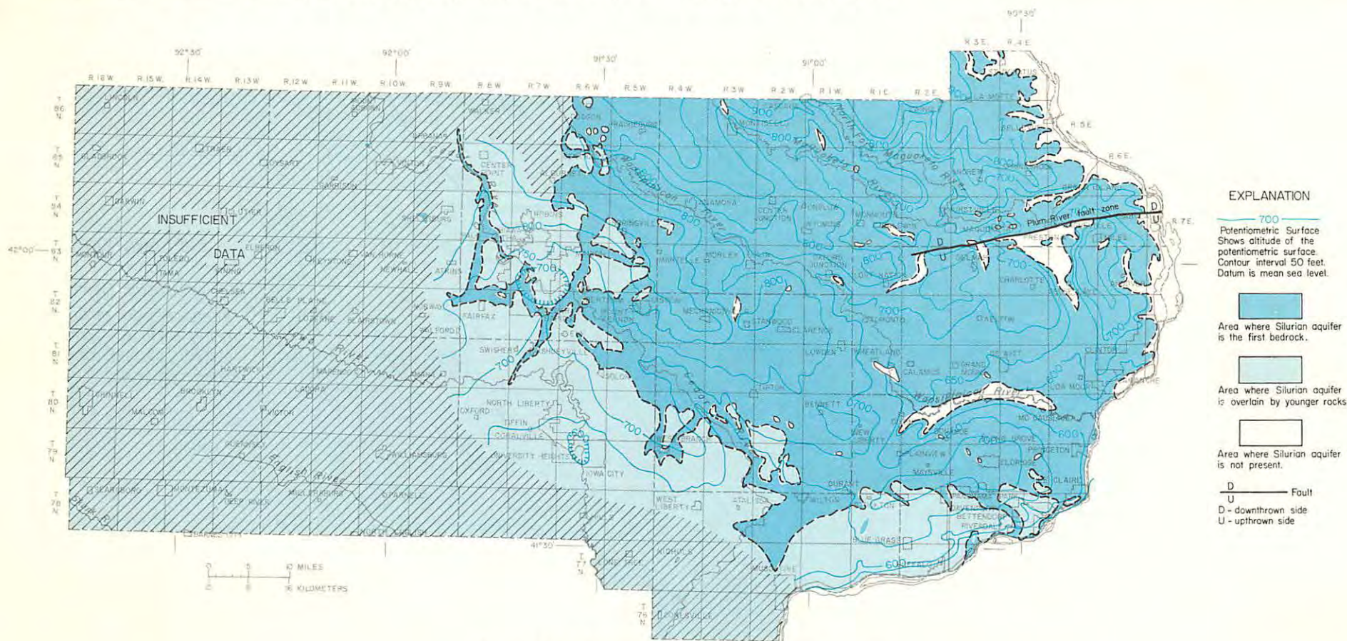
Figure 45.—Potentionmetric surface of the Silurian aquifer
