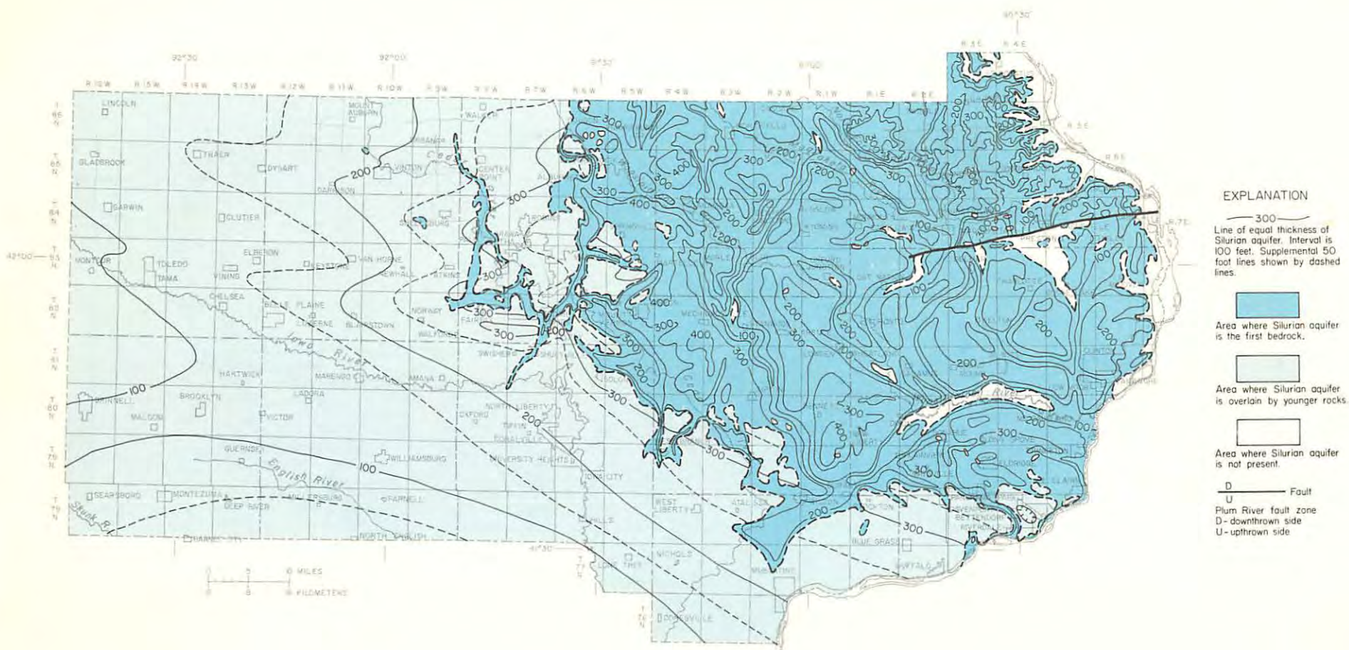
Figure 36.—Thickness of the Silurian aquifer
