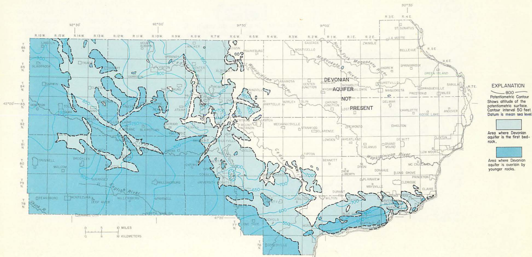
Figure 44.—Potentiometric surface of the Devonian aquifer
