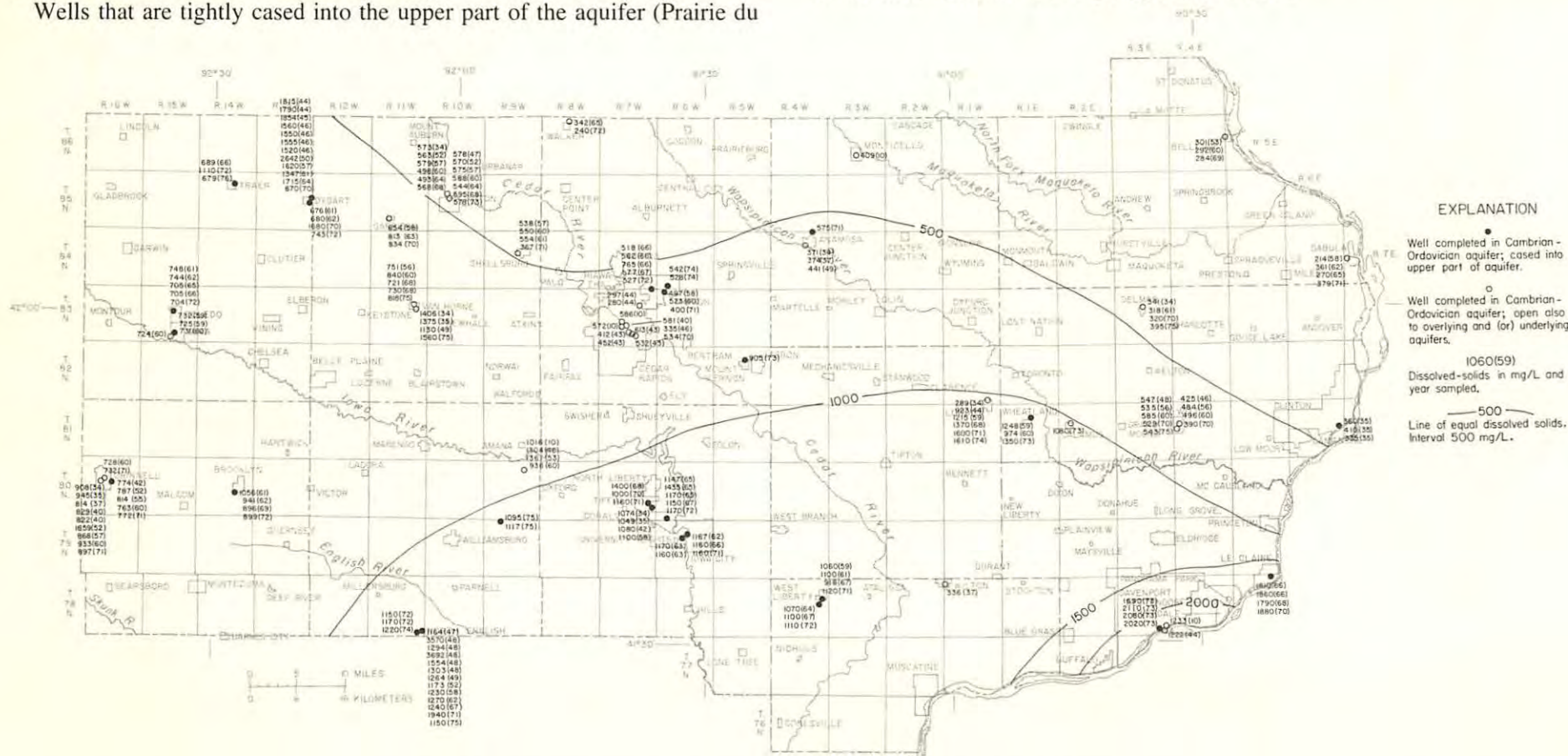
Figure 60.—Dissolved-solids concentrations in the Cambrian-Ordovician aquifer
