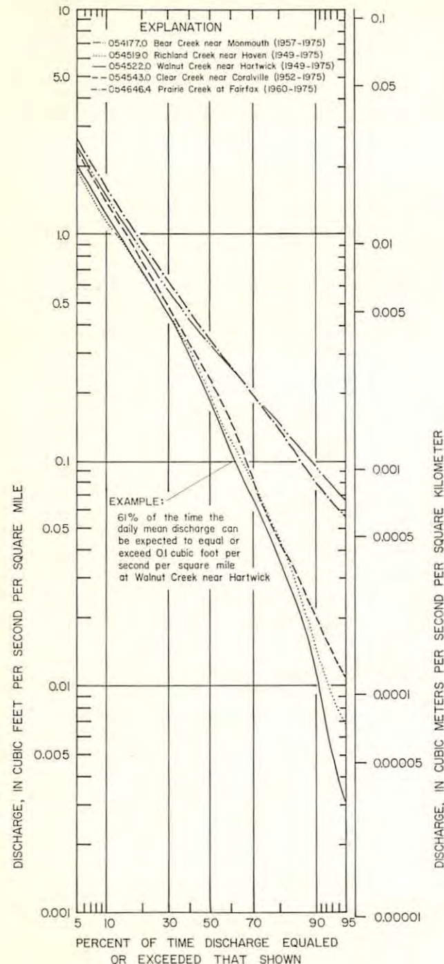
Figure 15.—Flow-duration curves for five east-central Iowa streams
