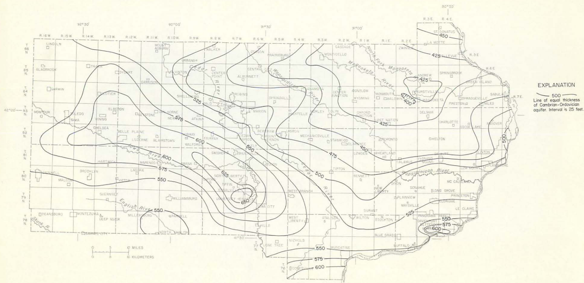
Figure 37.—Thickness of the Cambrian-Ordovician aquifer
