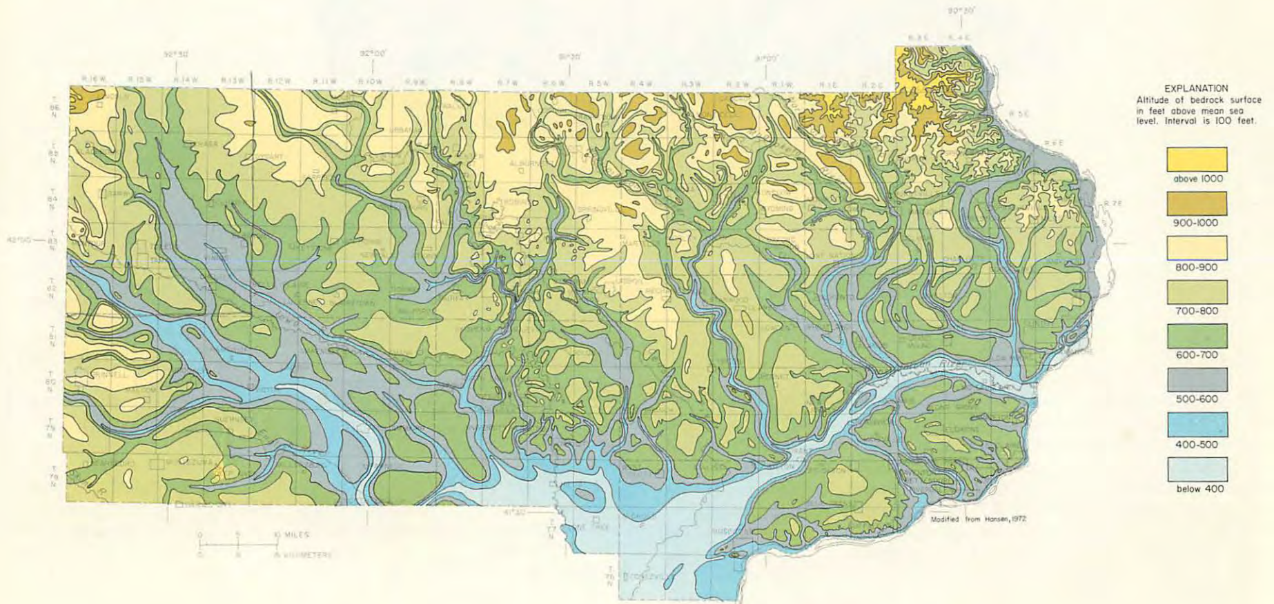
Figure 25.—Altitude and configuration of the bedrock surface
