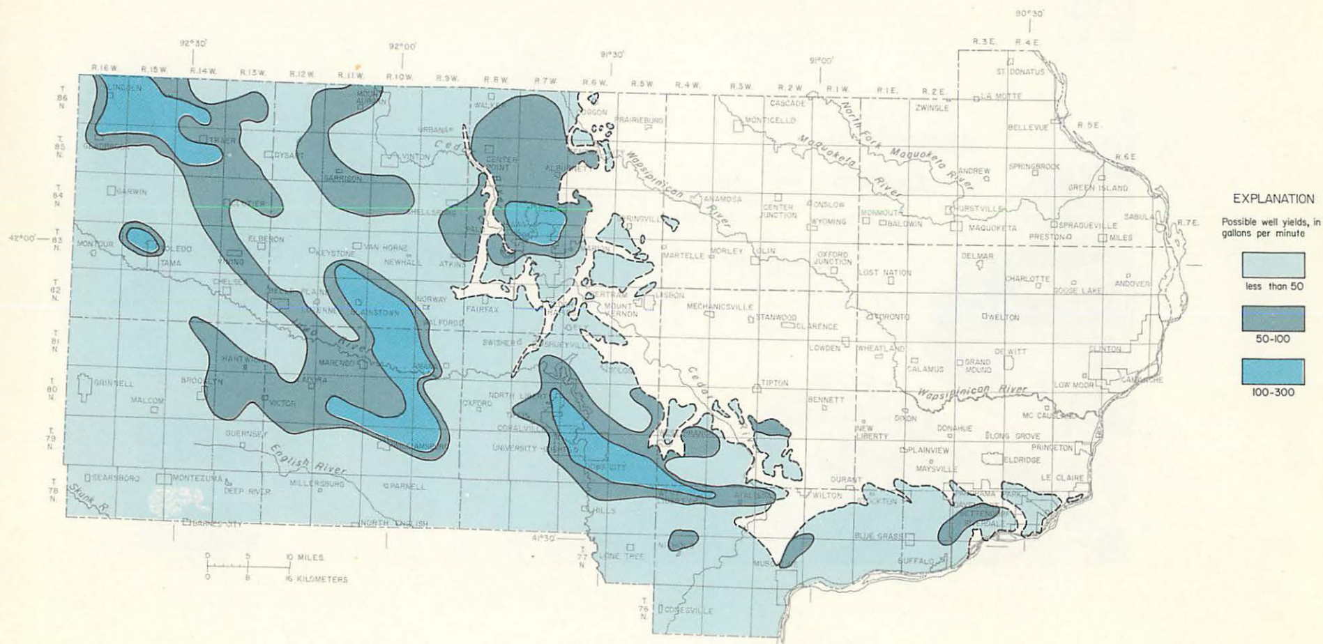
Figure 51.—Possible yields to individual wells; Devonian aquifer
