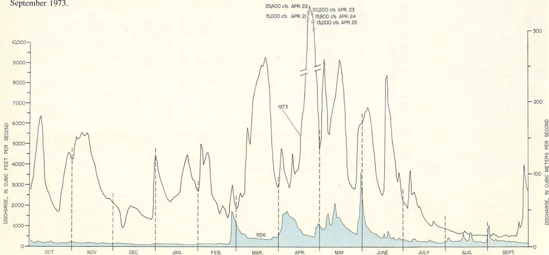
Figure 12.—Streamflow in Wapsipinicon River at DeWitt, Iowa in 1956 and 1973
