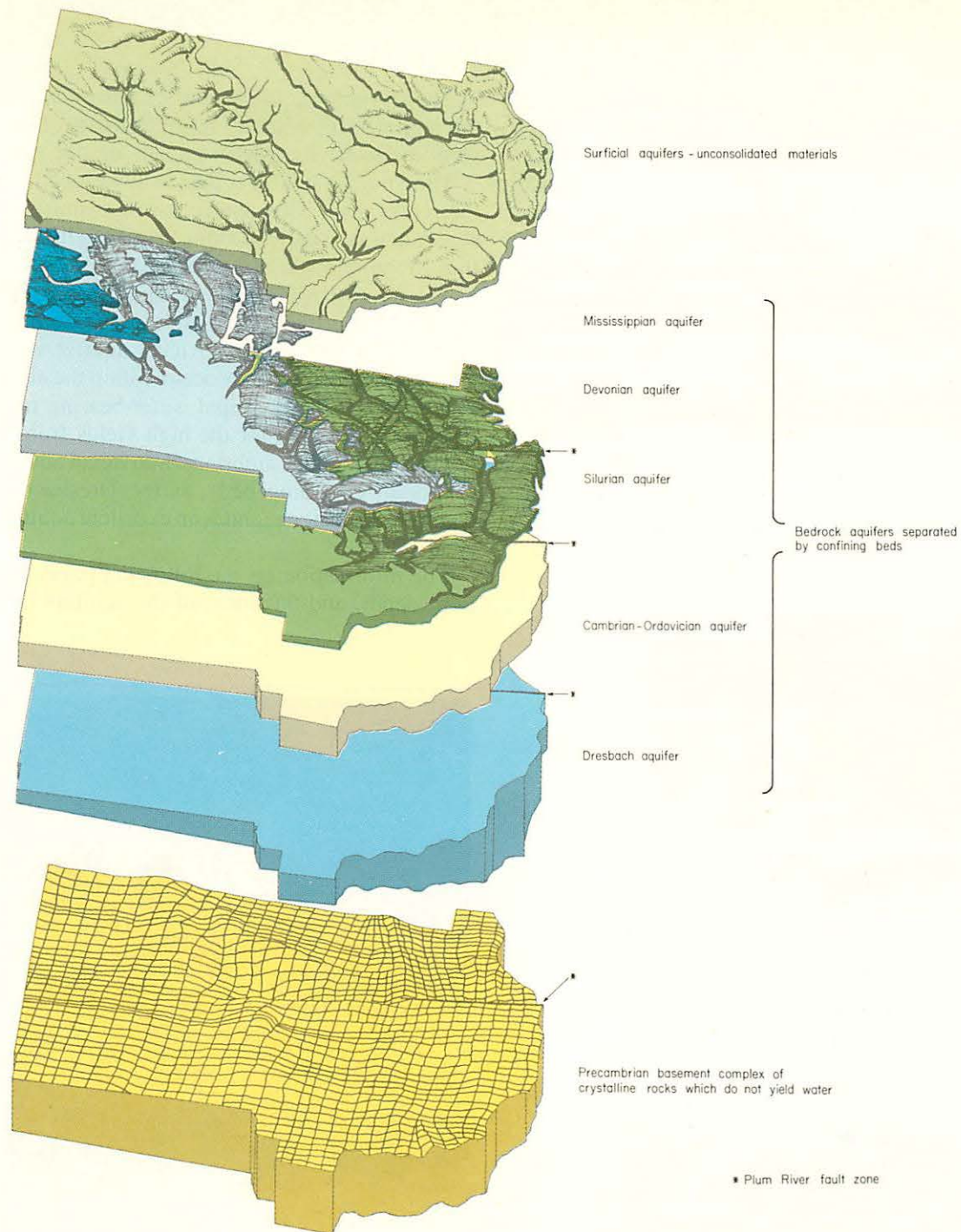
Figure 21.—The aquifers in east-central Iowa
