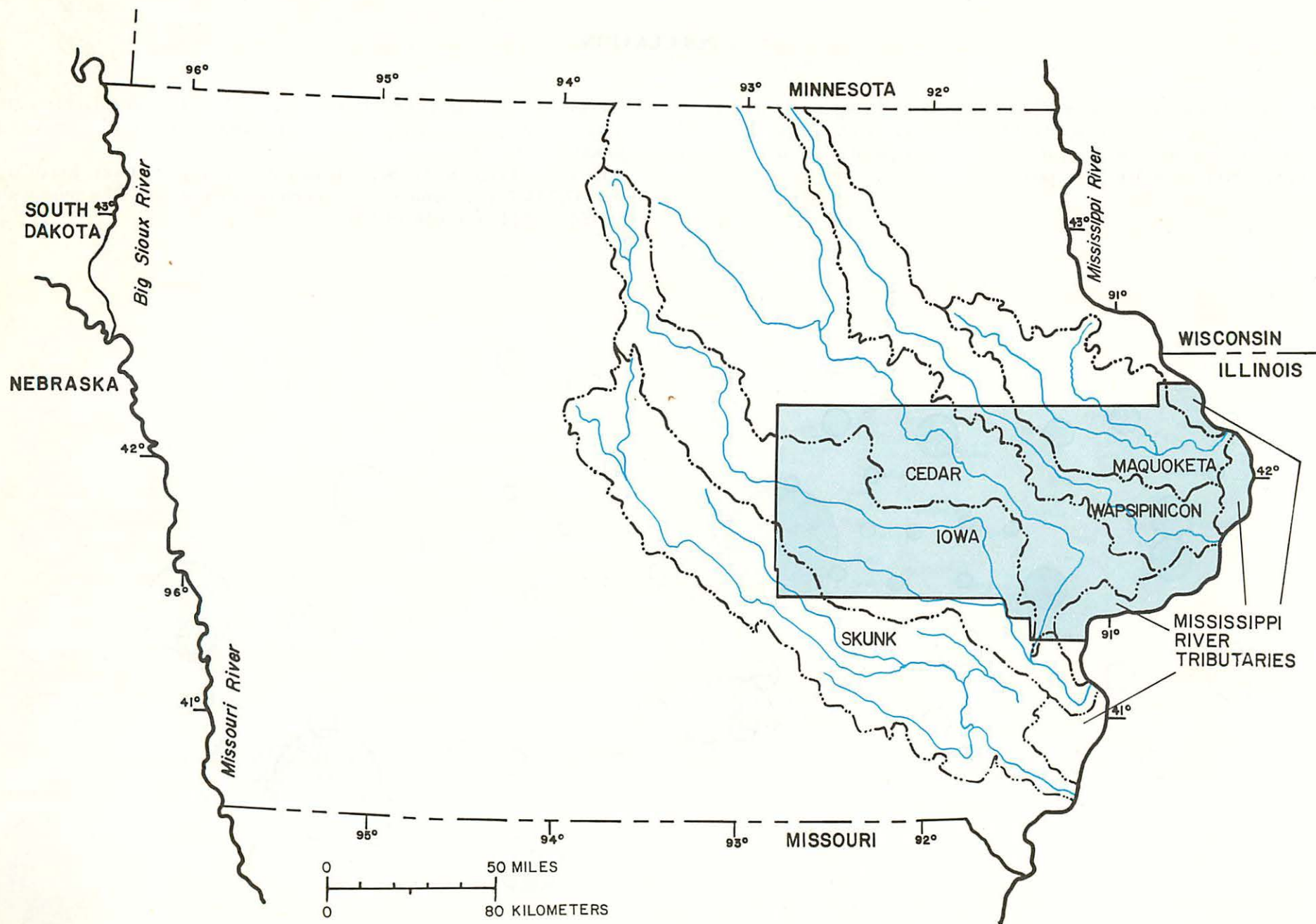
Figure 2.—Drainage basins in east-central Iowa
