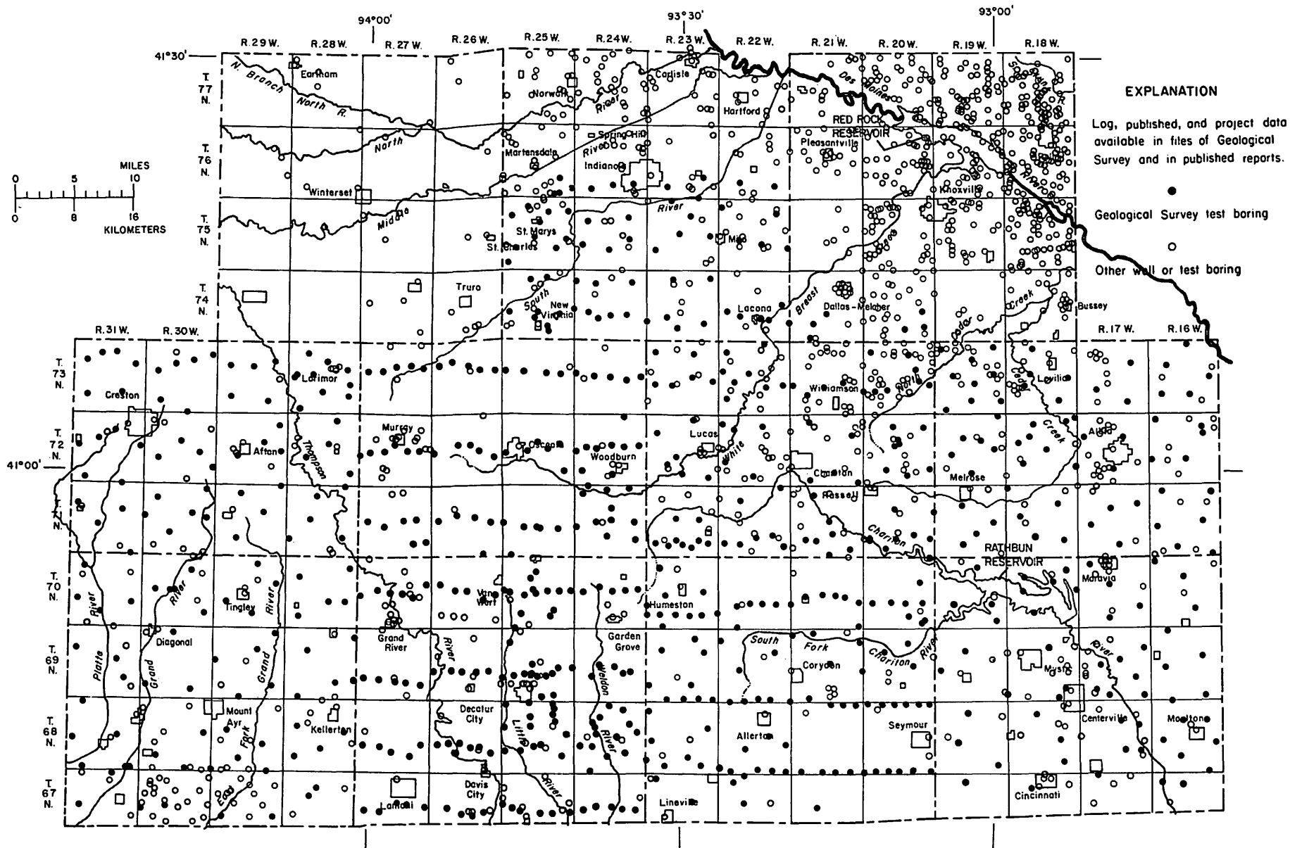
Figure 27.— Availability of well data
