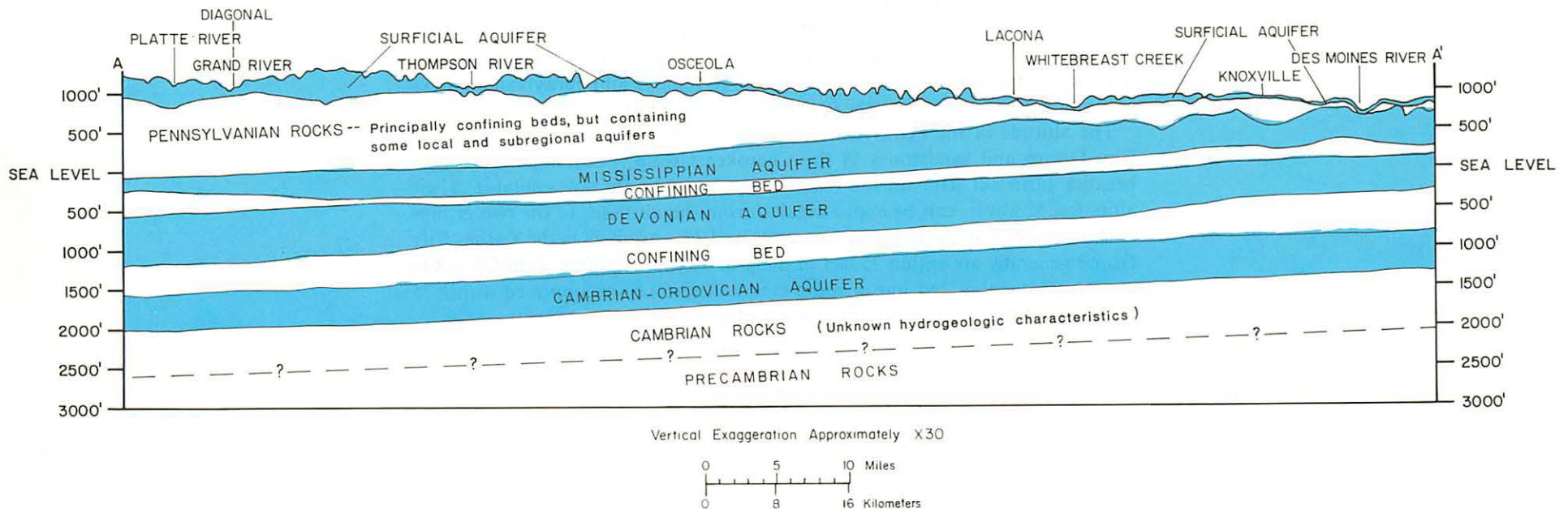
Figure 32.— Hydrogeologic cross section
