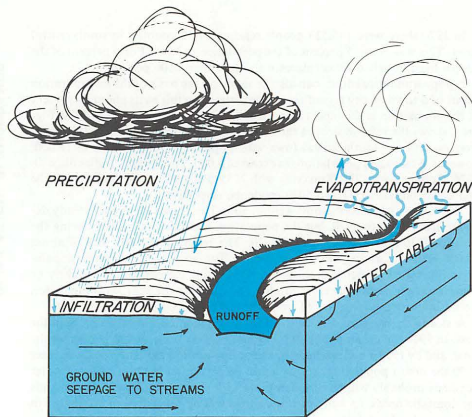
Figure 6.— The hydrologic cycle
