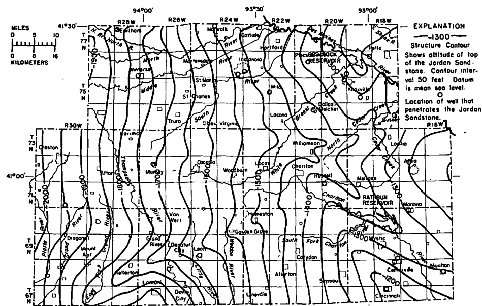
Figure 37.— Altitude of the top of the Jordan Sandstone
