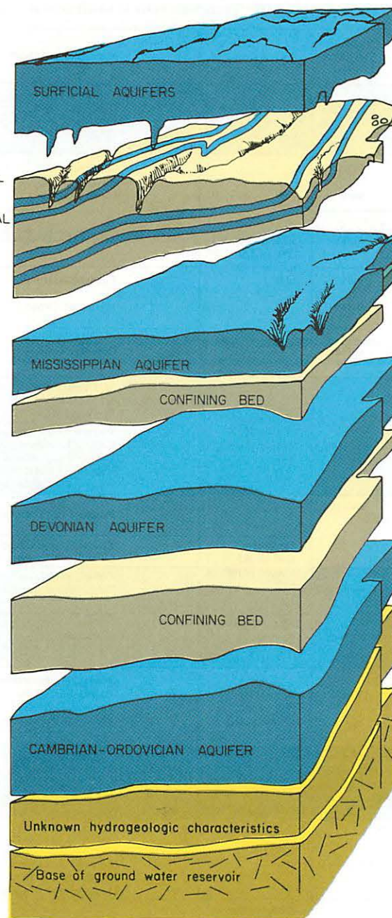
Figure 26.— The aquifers in south-central Iowa
