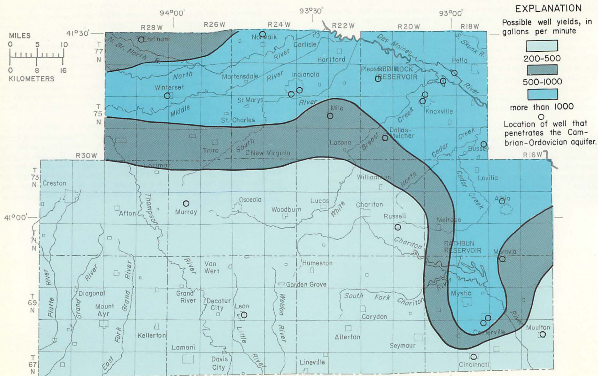
Figure 52.— Yields to individual wells; Cambrian-Ordovician aquifer
