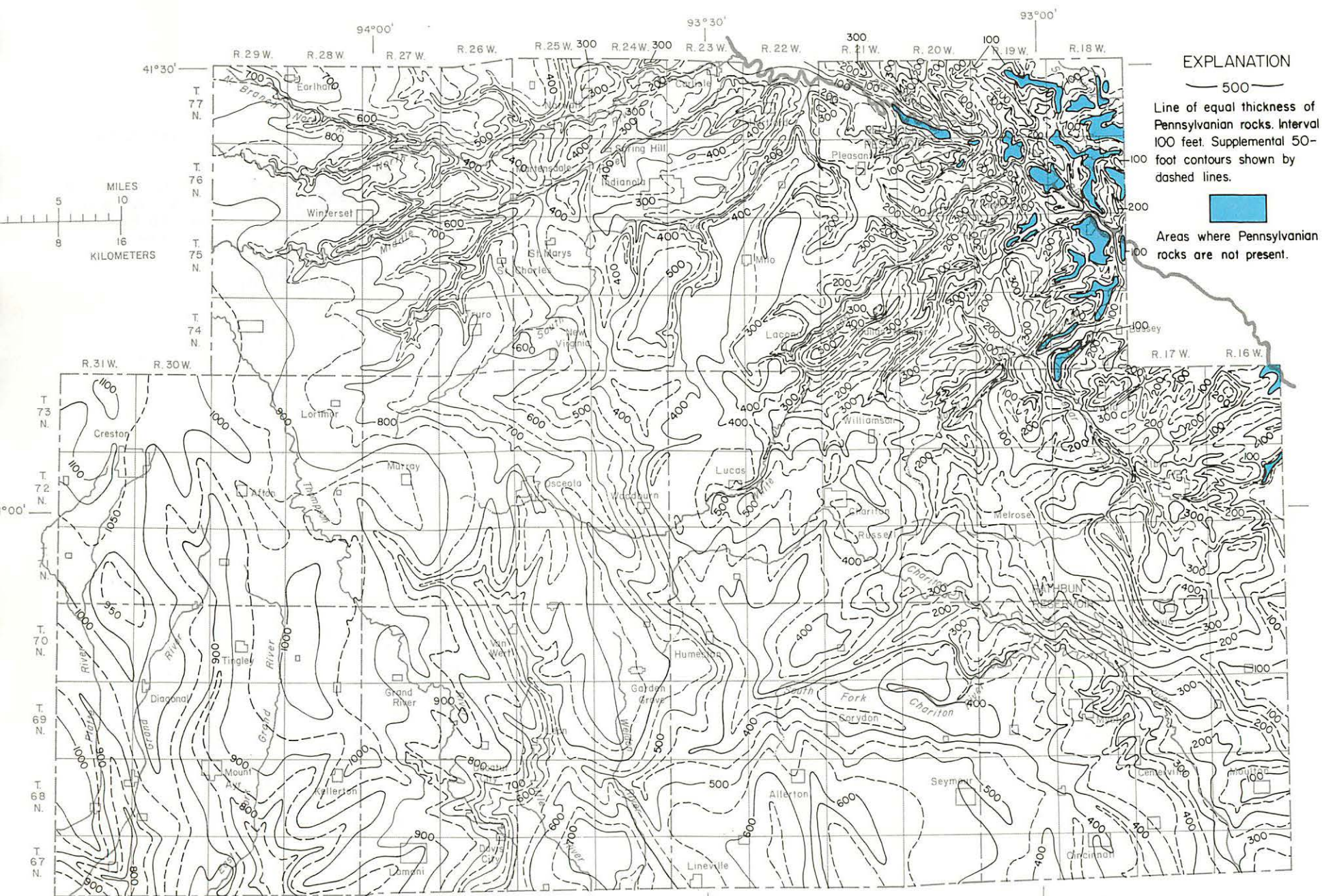
Figure 38.— Thickness of the Pennsylvanian rocks
