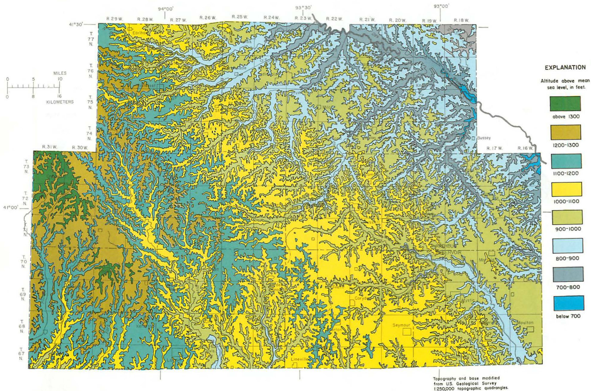
Figure 3.— Topographic map of south-central Iowa
