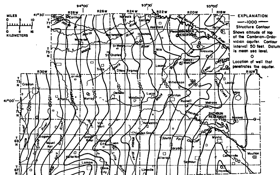
Figure 36.— Altitude of the top of the Cambrian-Ordovician aquifer
