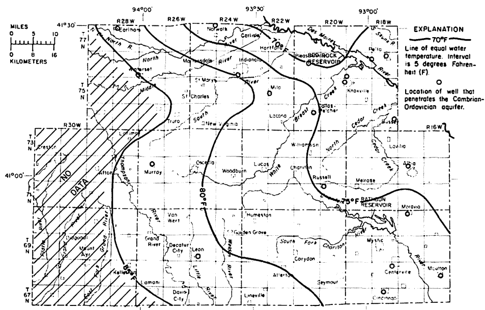
Figure 57.—Temperature of water in the Cambrian-Ordovician aquifer
