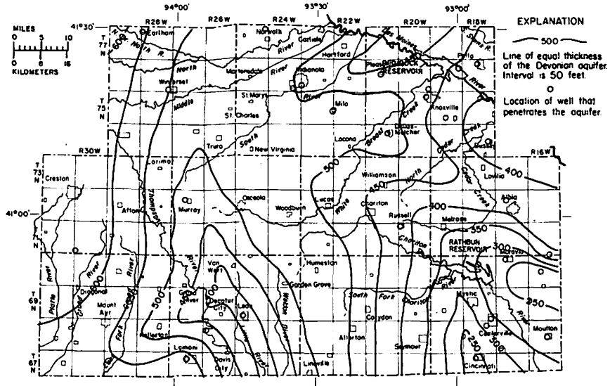
Figure 40.— Thickness of the Devonian aquifer
