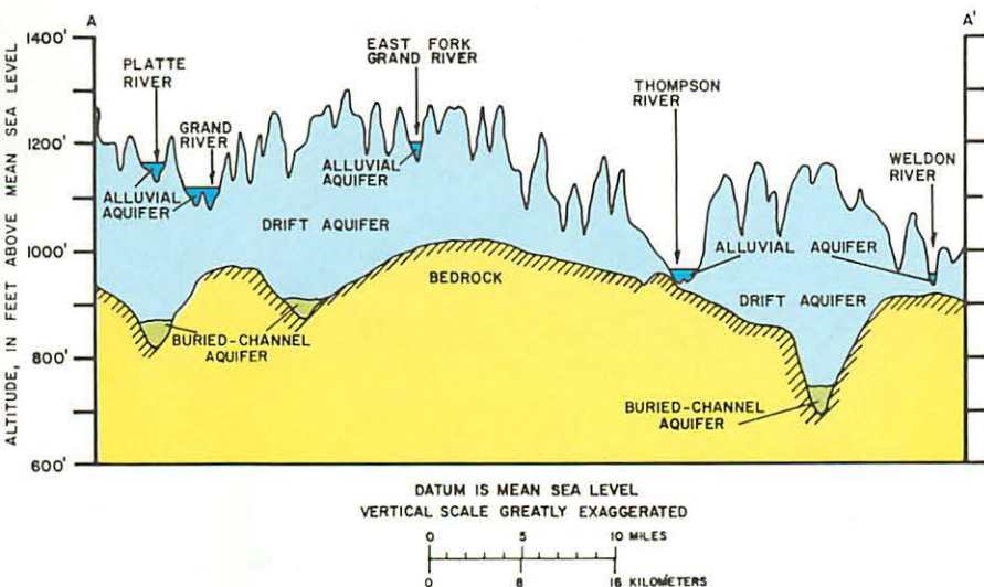
Figure 29.— Generalized hydrogeologic cross section of the surficial aquifers
