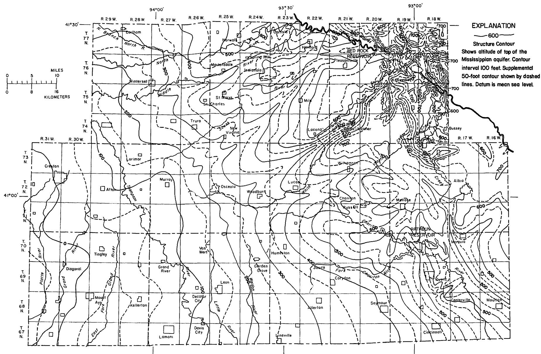
Figure 34.— Altitude of the top of the Mississippian aquifer
