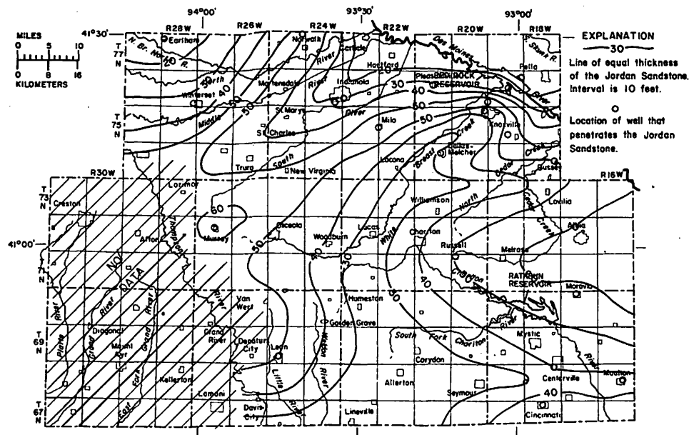
Figure 42.— Thickness of the Jordan Sandstone
