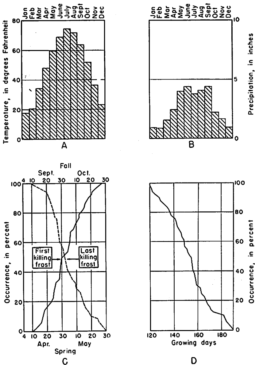
Figure 4.—Graphs showing (A) average temperature by months, (B) average precipitation by months, (C) occurrence of first and last killing frosts, and (D) length of growing season at Fort Dodge, Iowa. (Basic data from records of the U. S. Weather Bureau.)
