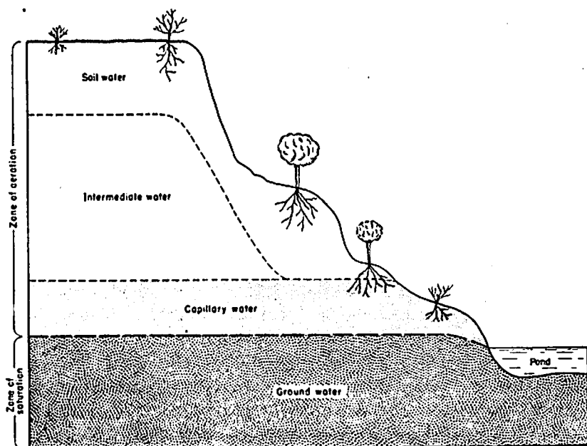
Figure 10.—Diagram showing divisions of subsurface water. (From Hershey, Robinson, and Jeffords, ms. in preparation, after Meinzer, 1923b.)
