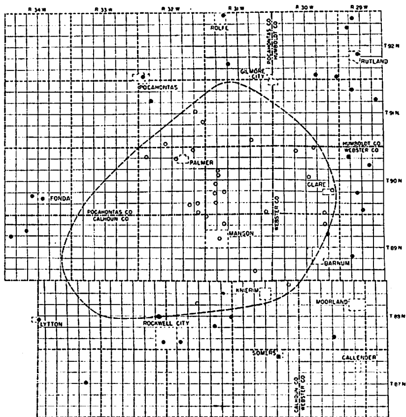
Figure 26.—Map of parts of Calhoun, Humboldt, Pocahontas, and Webster Counties showing the area occupied by the abnormal sequence of rocks in the vicinity of Manson, Calhoun County. Solid circles represent wells that encounter a normal Paleozoic section; open circles represent wells that encounter no Paleozoic rocks at equivalent depths.
