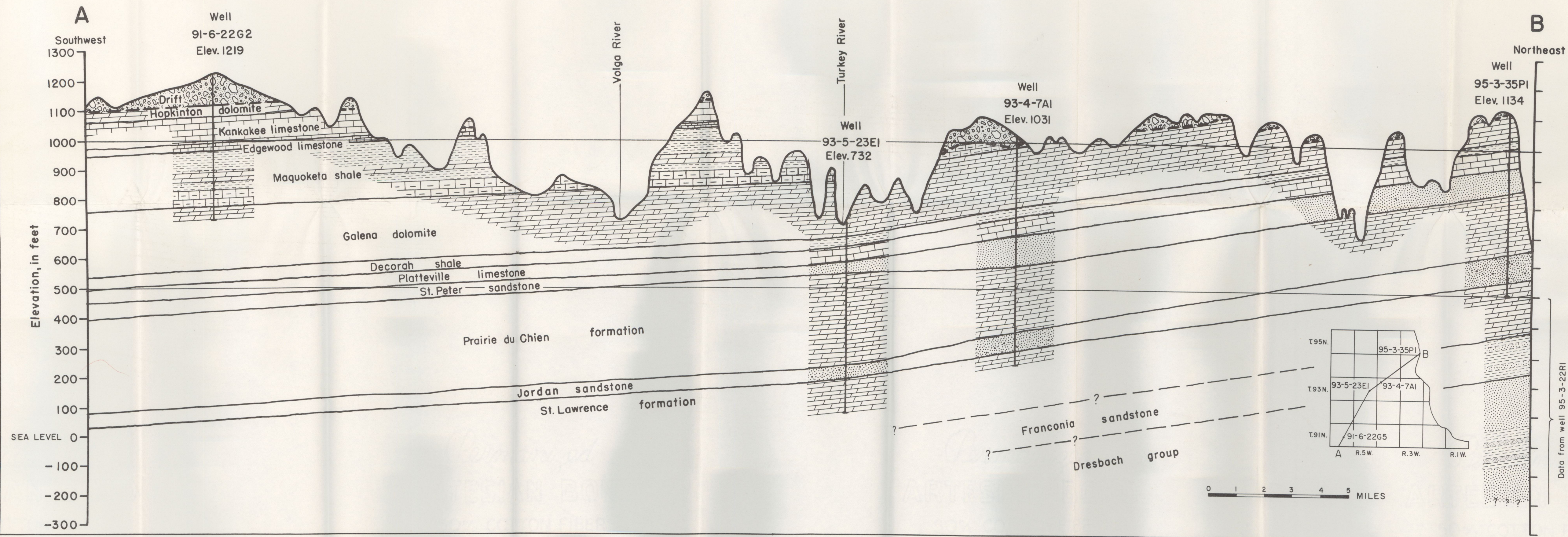
GEOLOGIC SECTION FROM STRAWBERRY POINT TO MCGREGOR, CLAYTON COUNTY, IOWA
