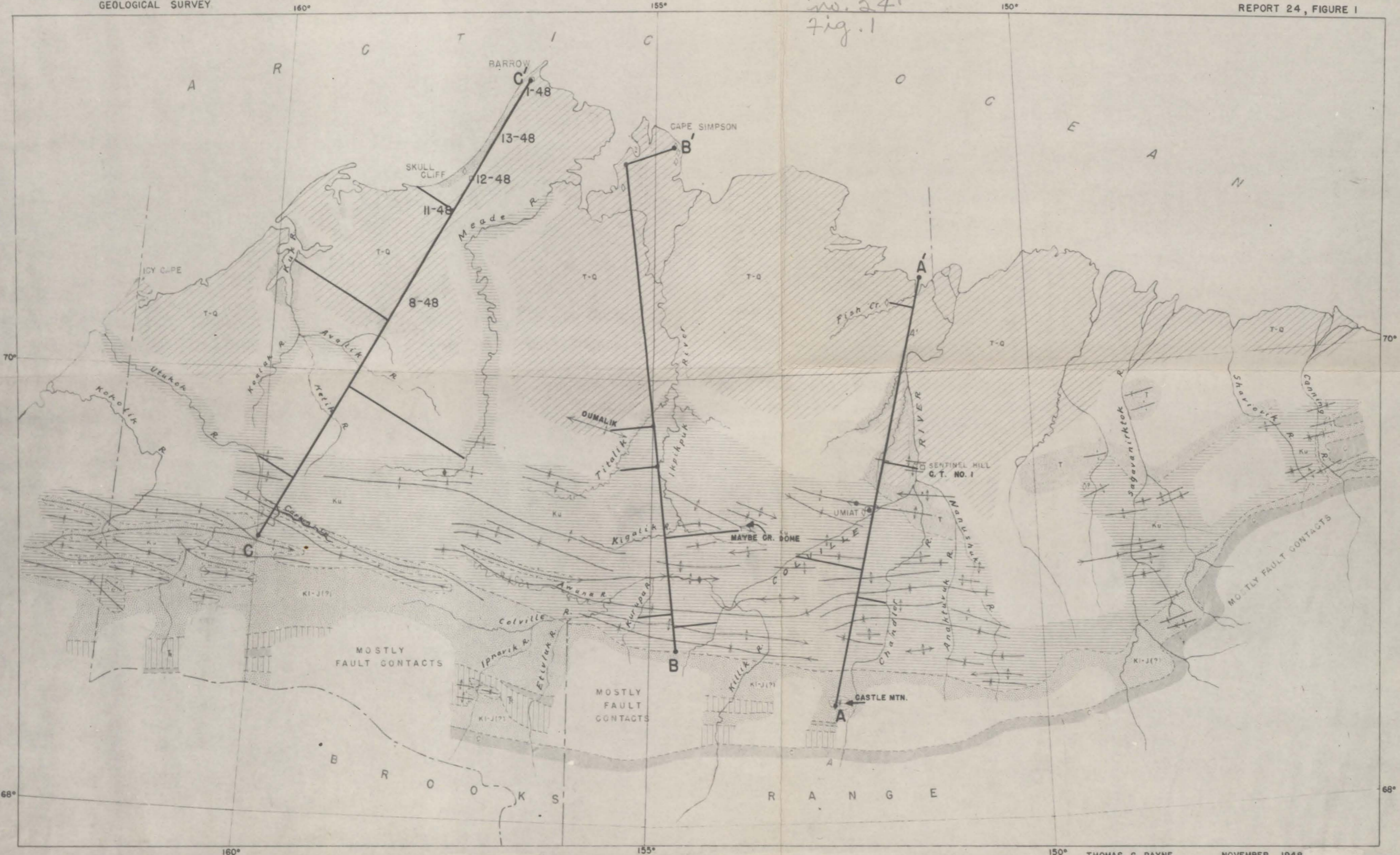
LOCATION MAP OF FACIES CROSS SECTIONS NORTHERN ALASKA
