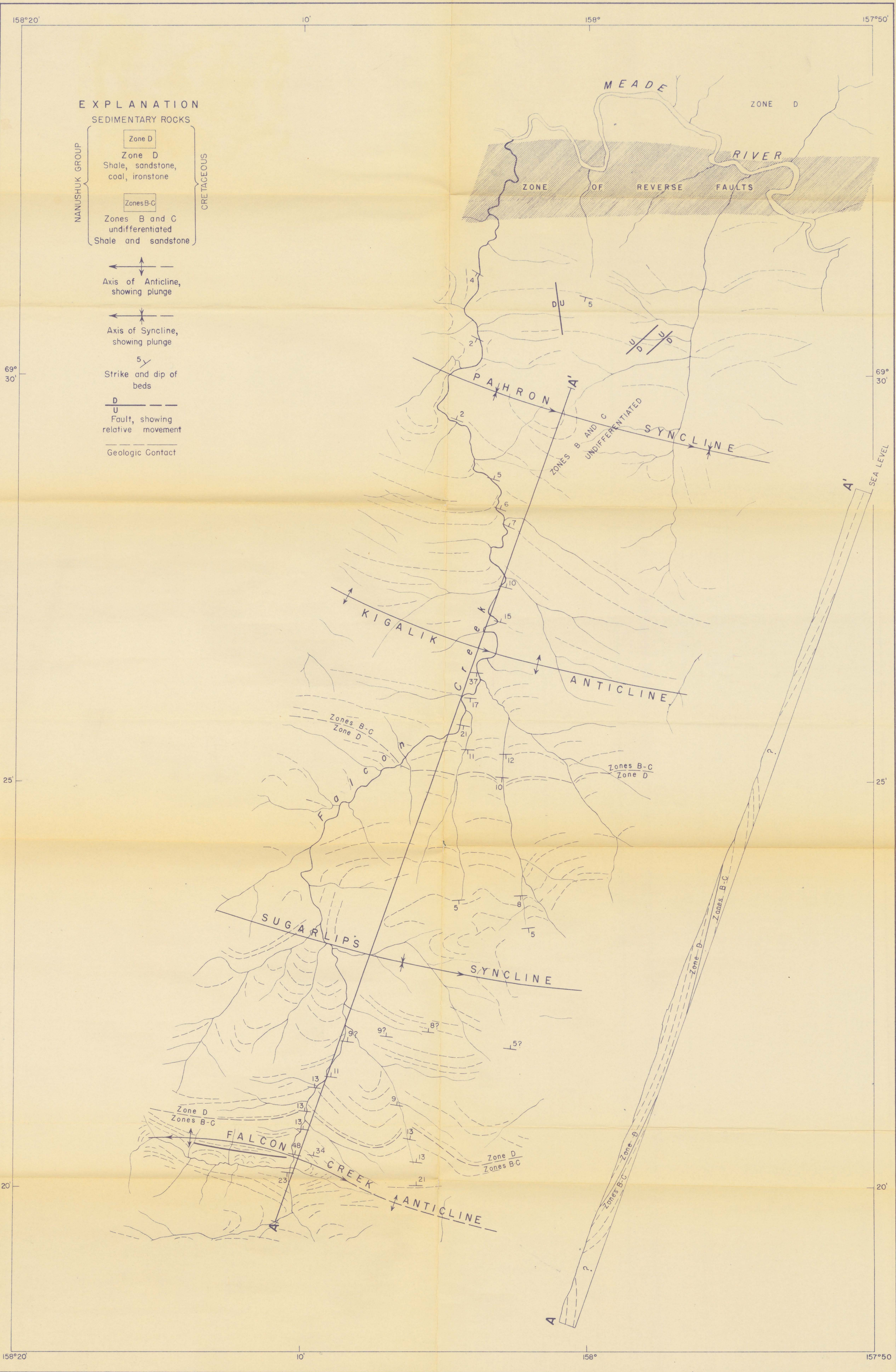
GEOLOGIC MAP AND CROSS-SECTION FALCON CREEK, UPPER MEADE RIVER AREA, ALASKA
