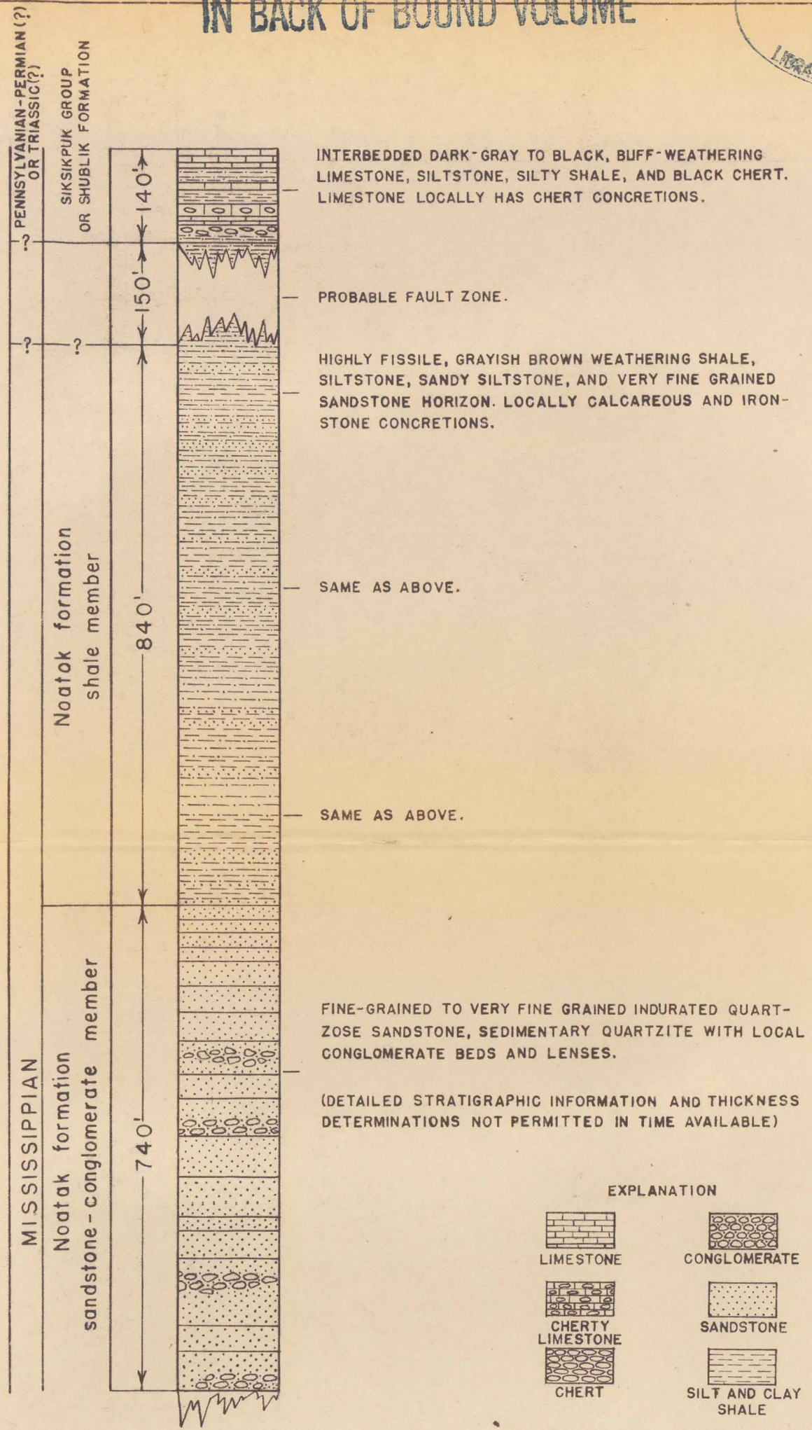
FIGURE 2 STRATIGRAPHIC SECTION ON EAST FORK OF THE ETIVLUK RIVER at approximately 68°21'N and 155°30' W
