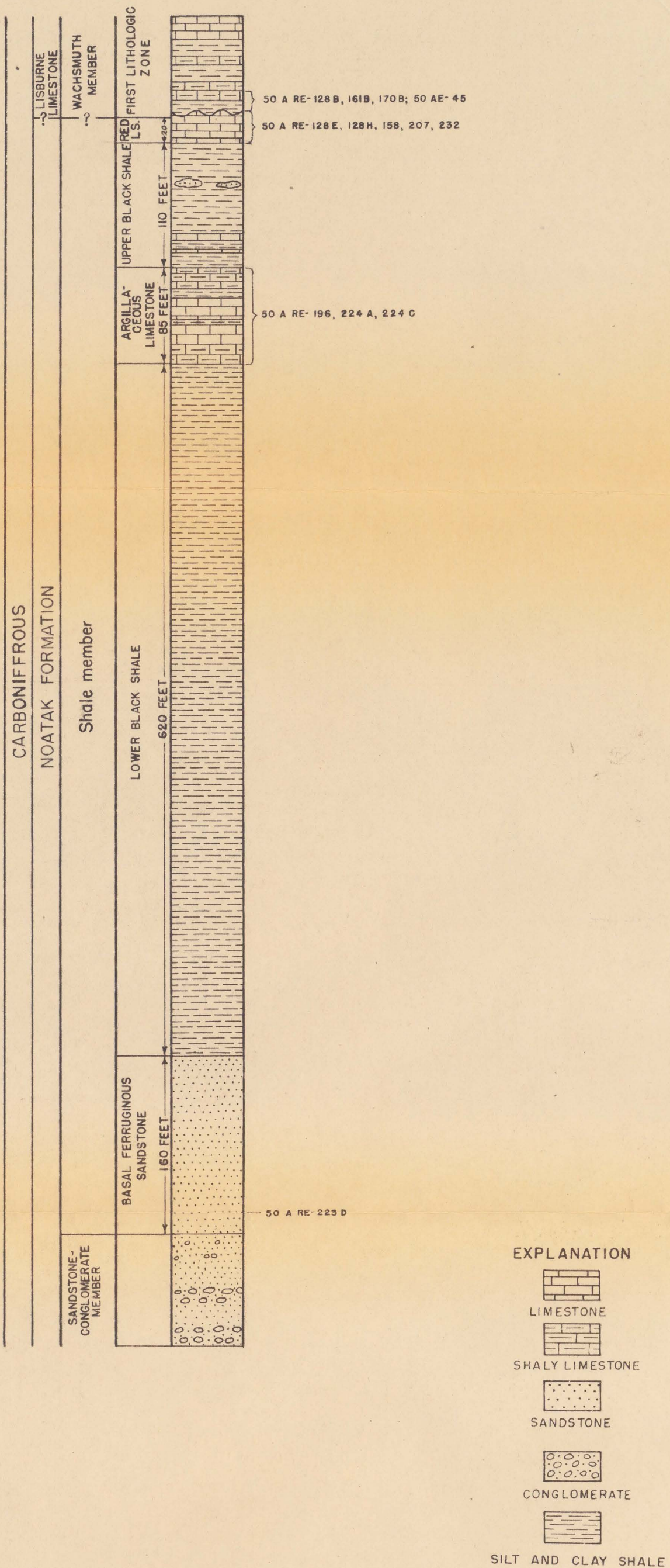
FIGURE 3.— NOATAK FORMATION, SHALE MEMBER TYPE SECTION AT KANAYUT LAKE, SHOWING PROBABLE CORRELATIONS WITH FOSSIL COLLECTIONS IN THE KURUPA — ETIVLUK RIVERS AREA
