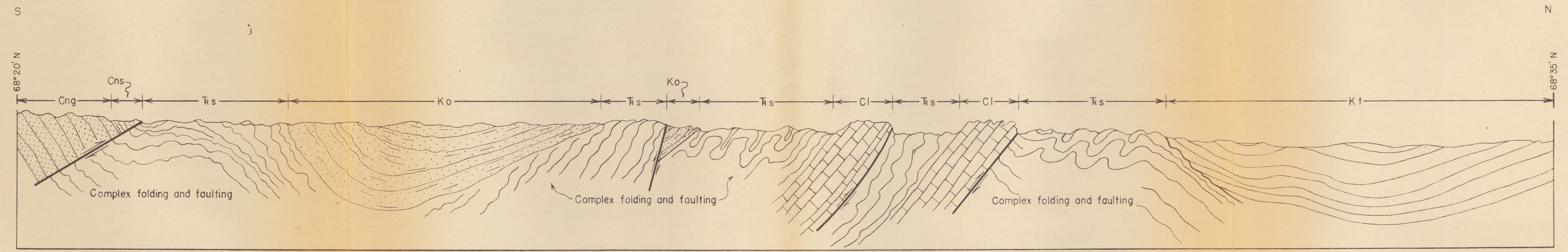
FIGURE 8. DIAGRAMMATIC STRUCTURE SECTION APPROXIMATELY ALONG 155^{\circ}30' W. , EAST FORK ETIVLUK RIVER
