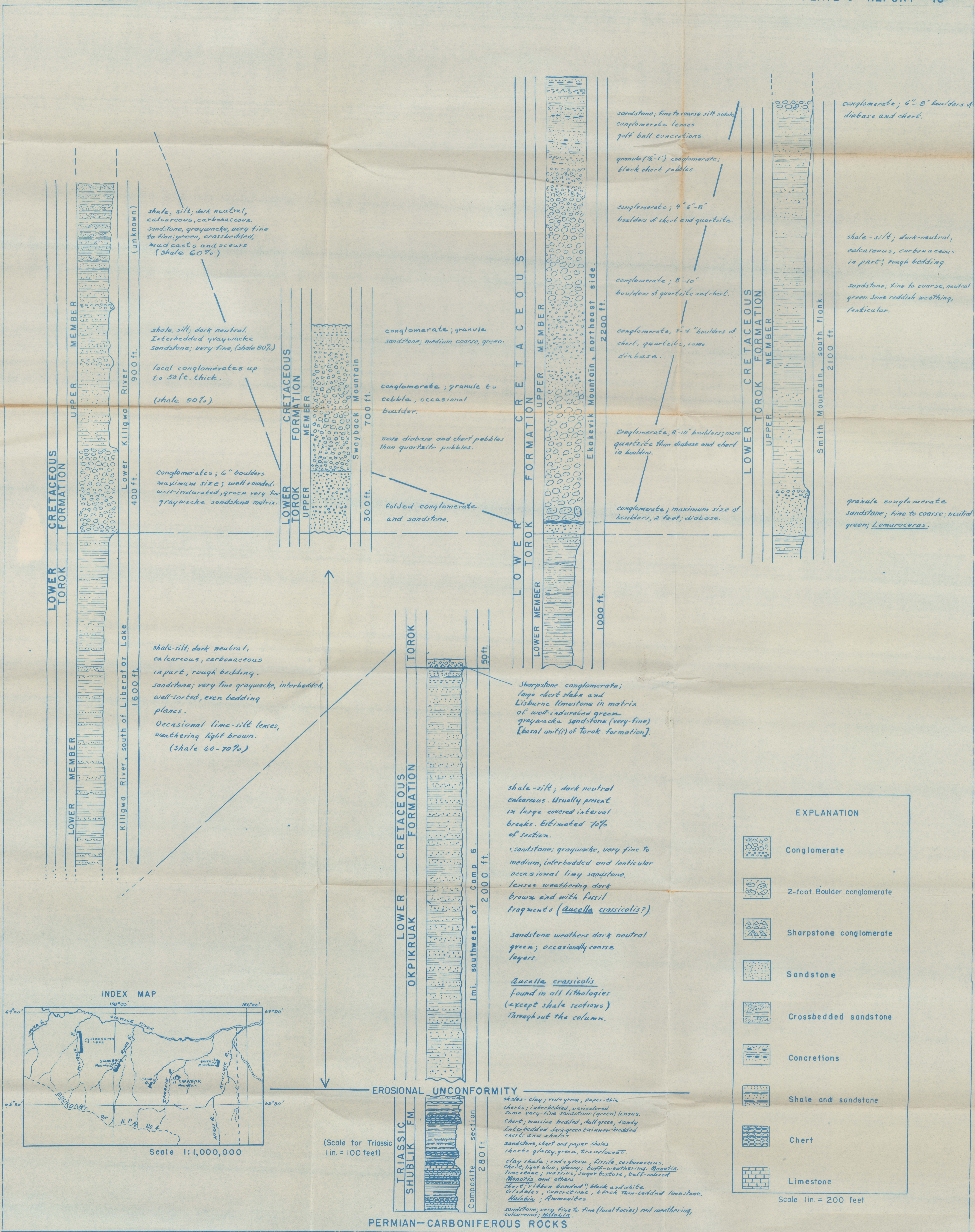
CORRELATED COLUMNAR SECTIONS OF MESOZOIC ROCK FORMATIONS in the SOUTHERN FOOTHILLS SECTION between the ETIVLUK and the KILIGWA RIVERS, ALASKA
