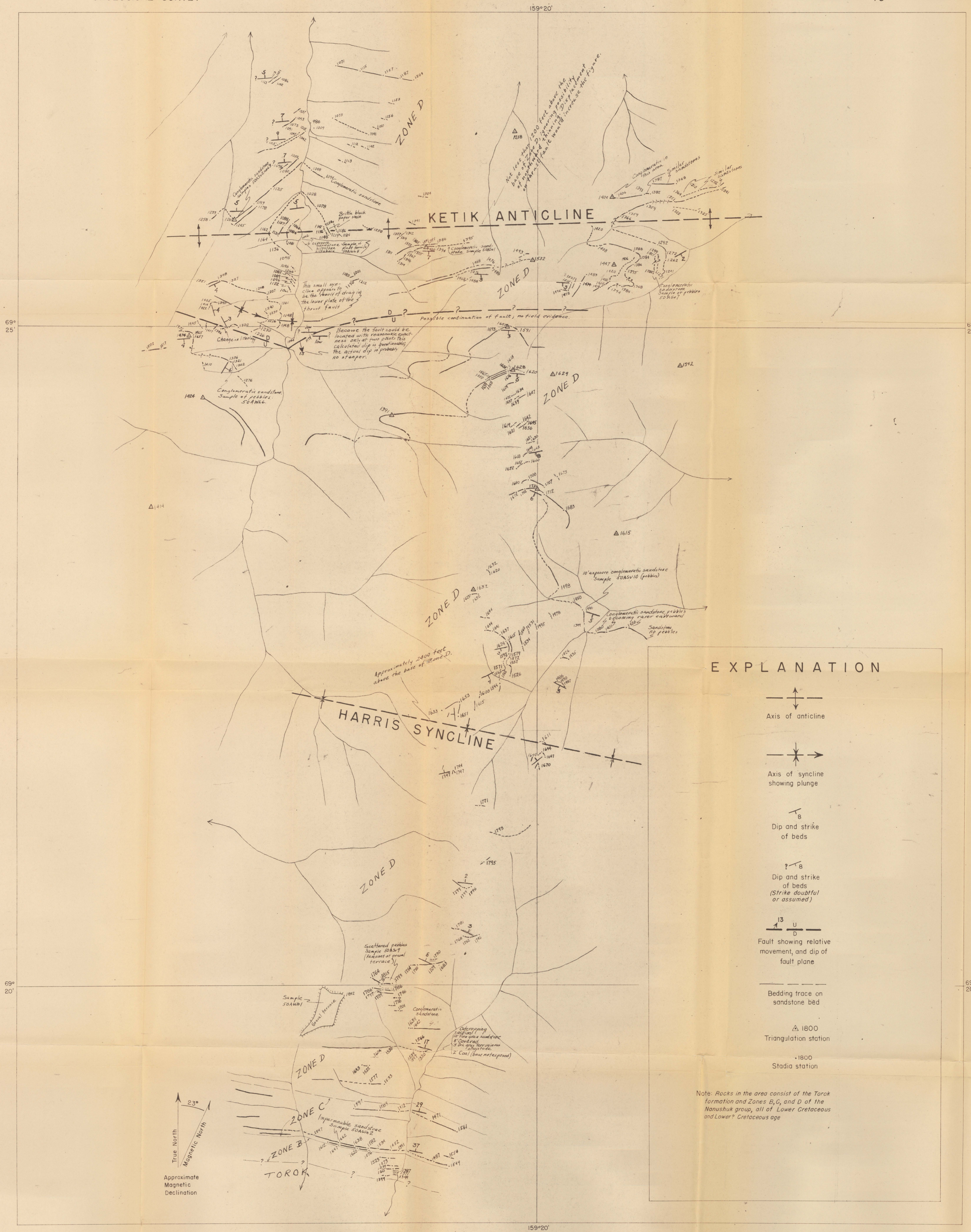
FIGURE 3.— GEOLOGIC MAP OF PART OF THE KETIK ANTICLINE AND AREA TO THE SOUTH, ALASKA
