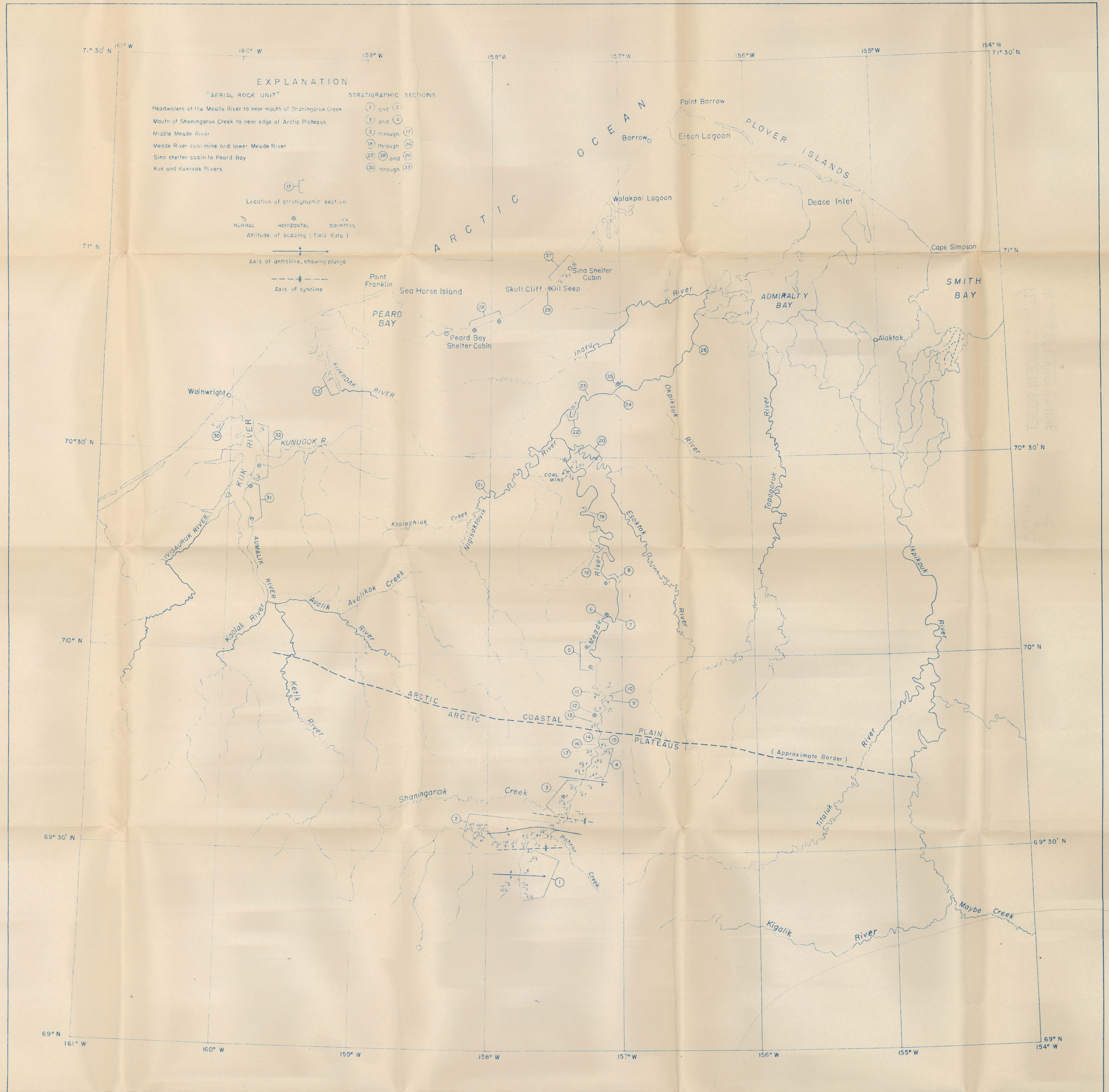
MAP SHOWING GEOLOGICAL DATA OF THE AREA OF THE MEADE AND KUK RIVERS AND POINT BARROW, ALASKA
