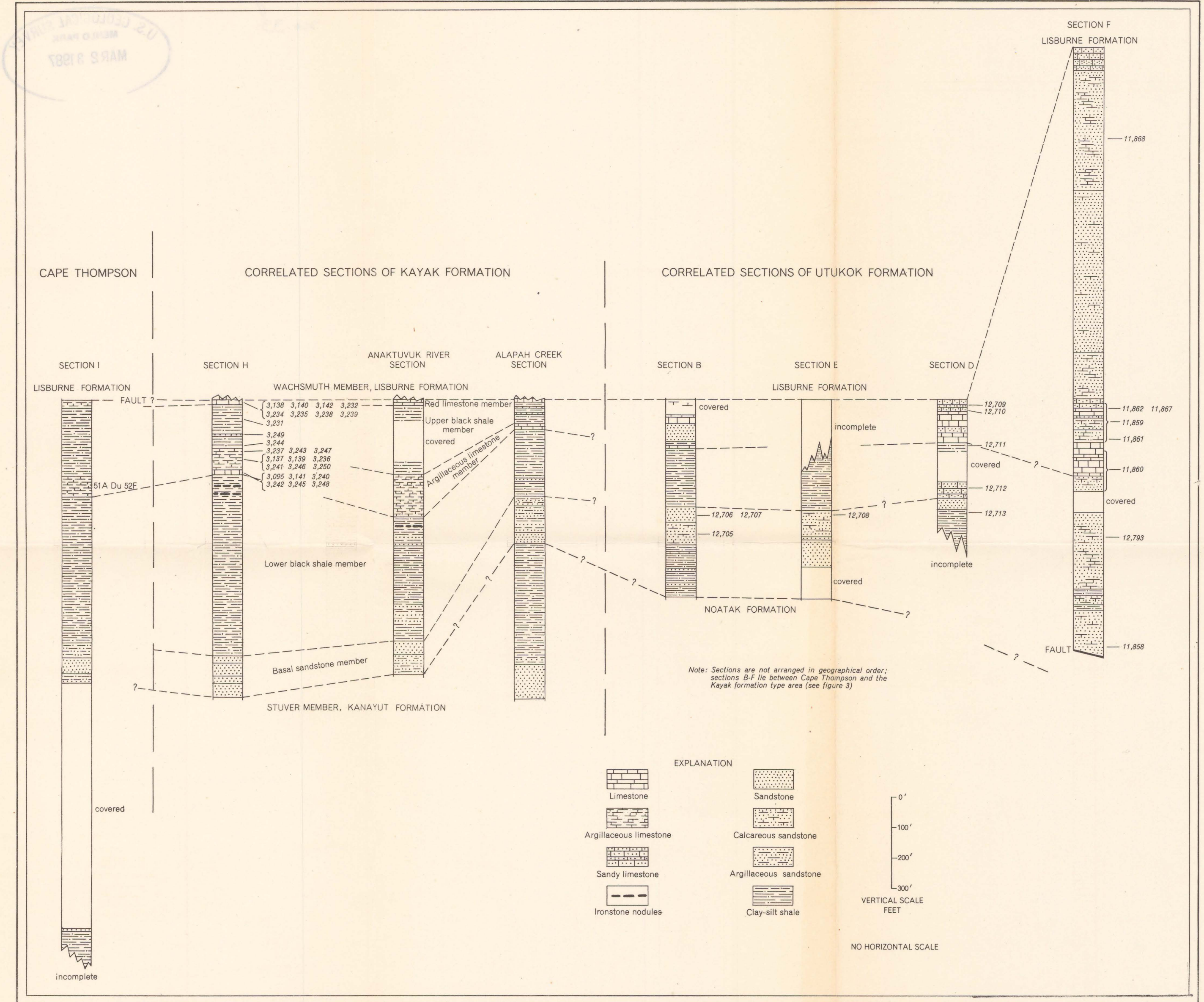
PLATE 3 — CORRELATION OF GENERALIZED SECTIONS OF THE KAYAK AND UTUKOK FORMATIONS
