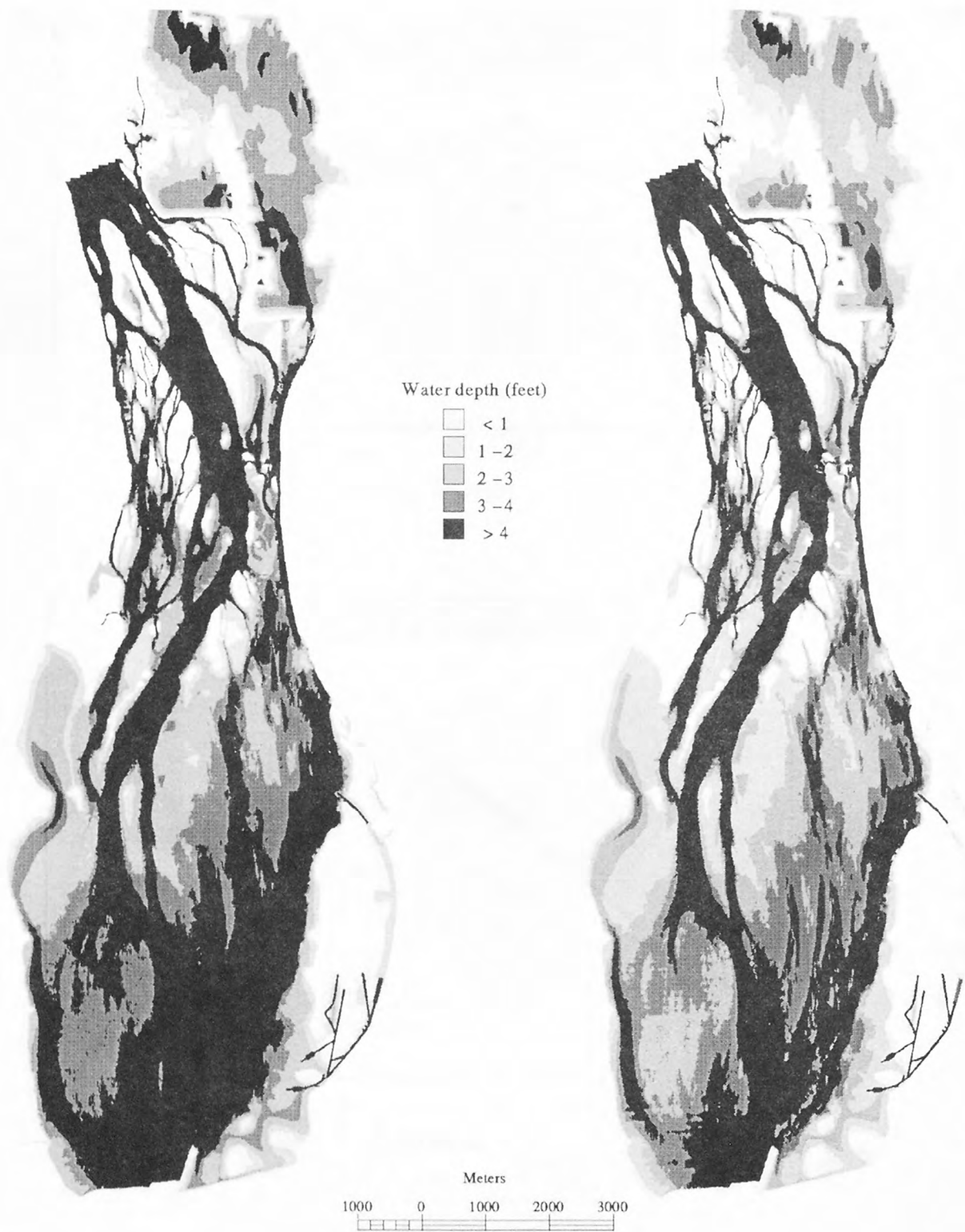
Figure 9. Maps of water depth, at 50,000 cfs, for the study area of Pool 13 when water levels at the dam are held at 583 feet (left) and 582 feet (right) above sea level.
