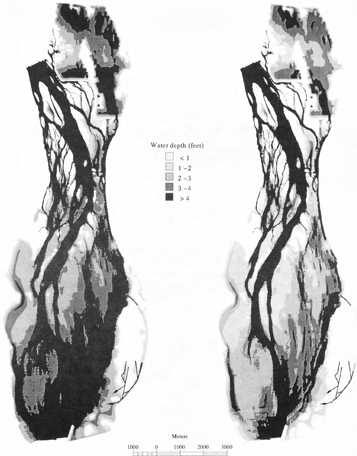
Figure 10. Maps of water depth, at 70,000 cfs, for the study area of Pool 13 when water levels at the dam are held at 583 feet (left) and 581 feet (right) above sea level.
