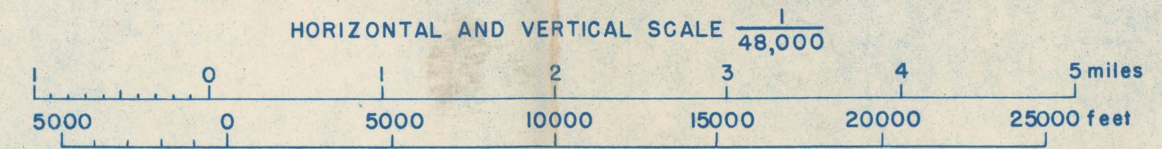
PRELIMINARY GEOLOGICAL CROSS SECTIONS IN THE AREA OF THE KIGALIK AND AWUNA RIVERS, ALASKA
