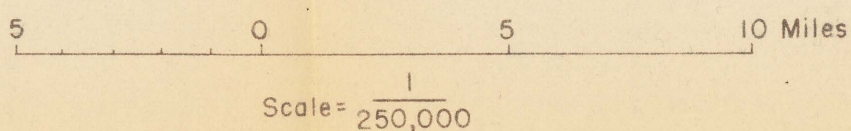
MAP SHOWING GEOLOGICAL DATA IN THE AREA OF THE TITALUK AND UPPER IKPIJUK AND MEADE RIVERS, NAVAL PETROLEUM RESERVE NO. 4, ALASKA
