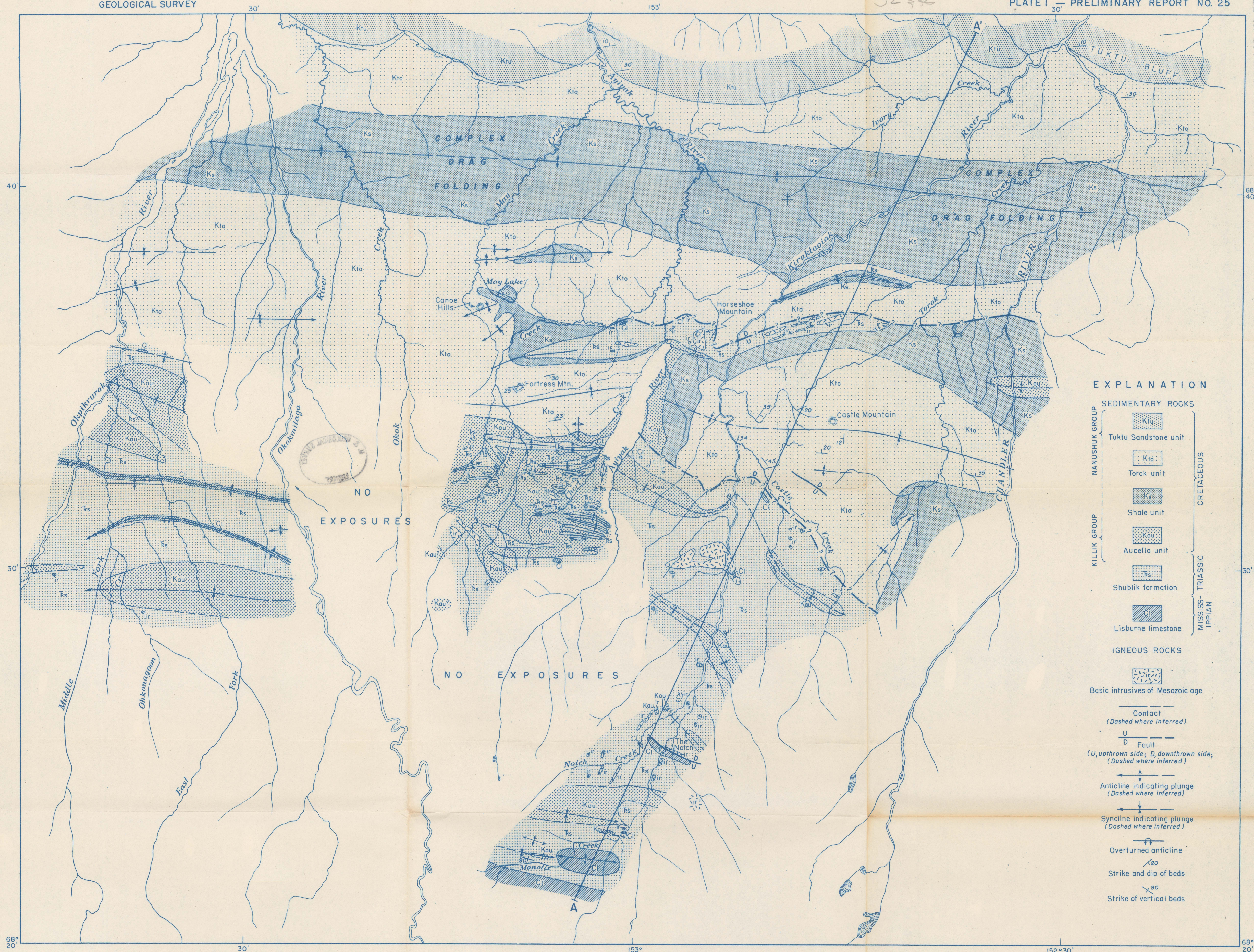
PLATE I. — PRELIMINARY GEOLOGIC MAP OF THE OKPIKRURAK AND KIRUKTAGIAK RIVERS AREA, ALASKA
