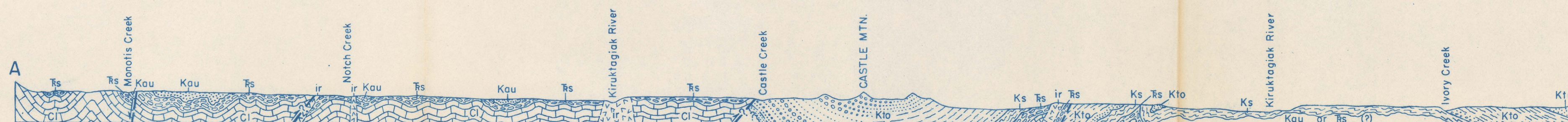
GENERALIZED CROSS-SECTION APPROXIMATELY ALONG LINE A-A' (NO VERTICAL EXAGGERATION)
