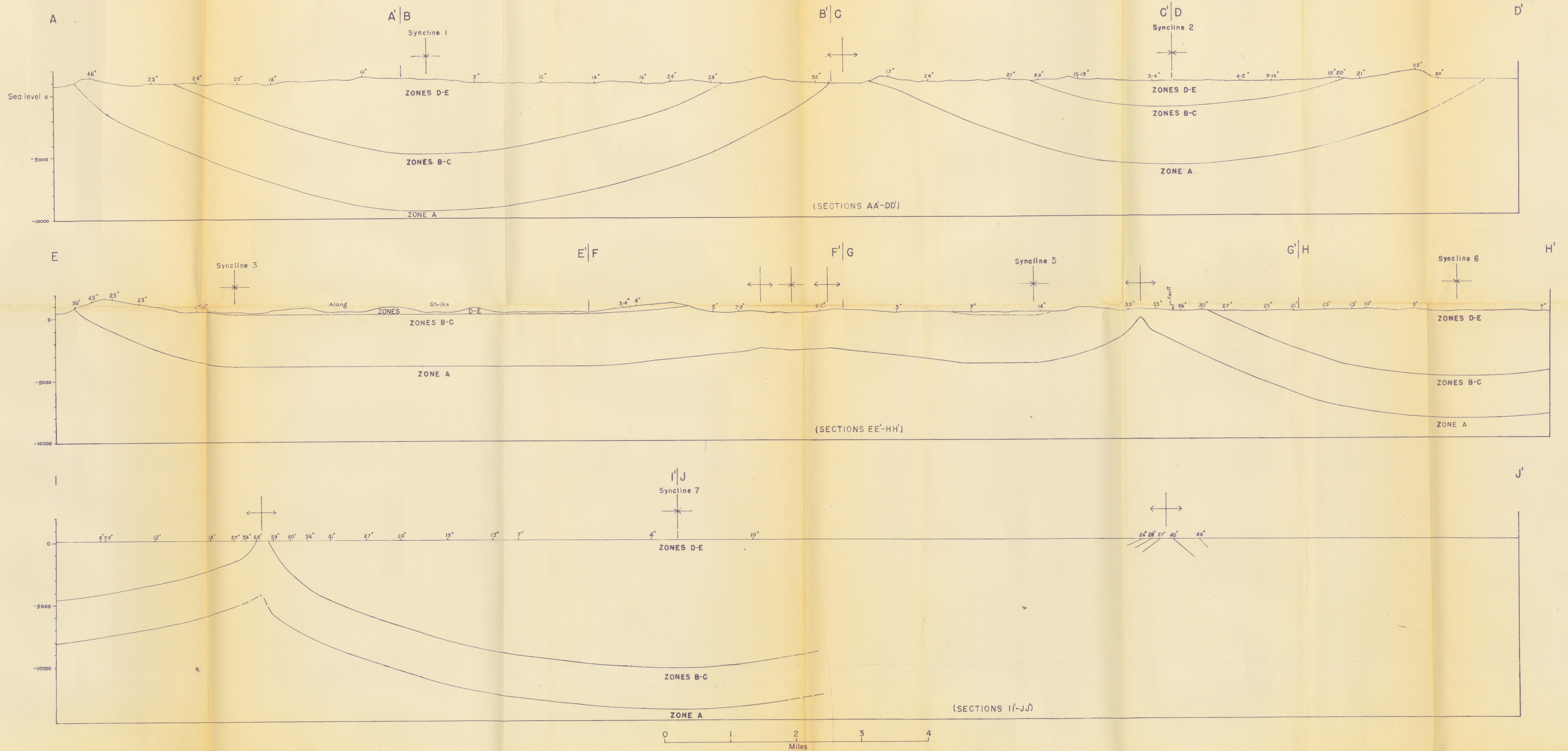
FIGURE 2. STRUCTURE SECTIONS OF NANUSHUK GROUP — KUKPOWRUK RIVER
