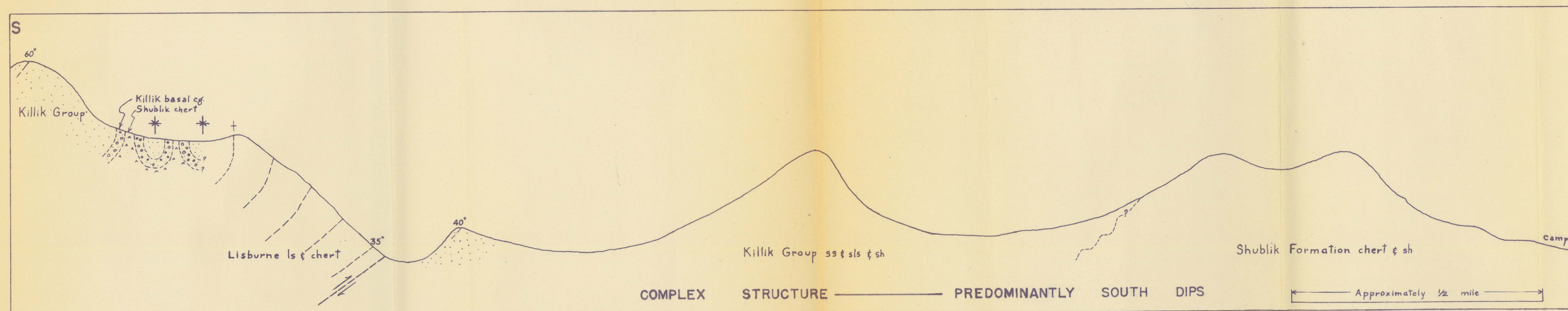
FIGURE 3. STRUCTURAL INTERPRETATION AT MOUNTAIN FRONT - KUKPOWRUK RIVER (NOT TO SCALE)
