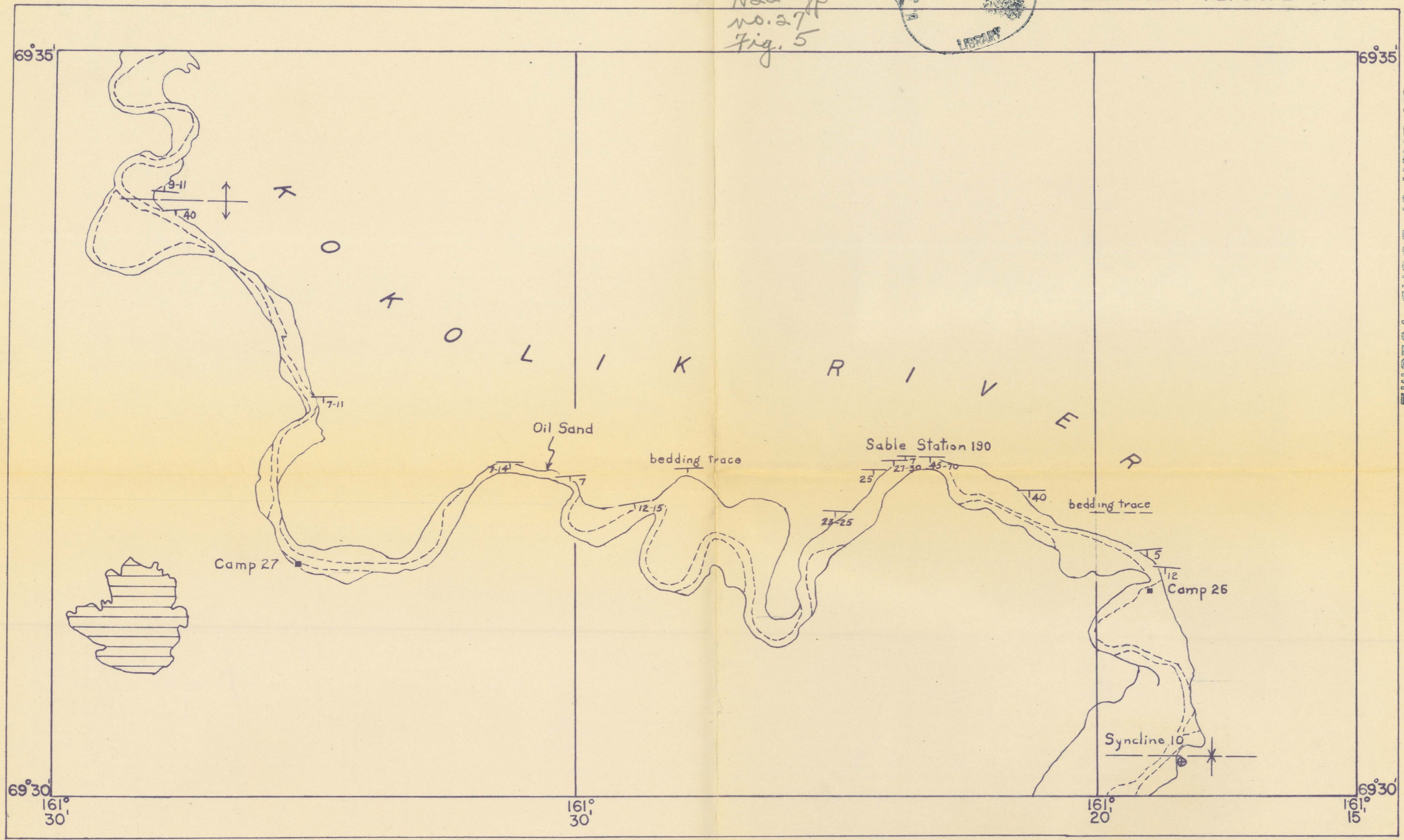
STRUCTURAL MAP OF OIL SAND AREA ON KOKOLIK RIVER
