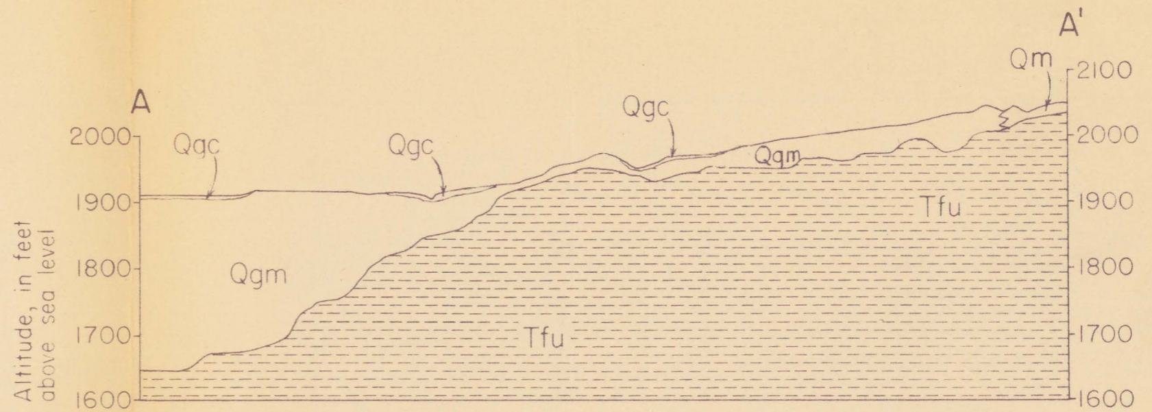
GENERALIZED GEOLOGIC CROSS SECTION ALONG LINE A-A'
