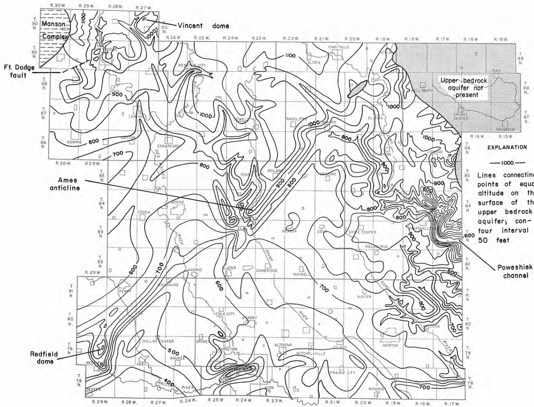
The upper bedrock aquifer, its altitude and surface configuration
