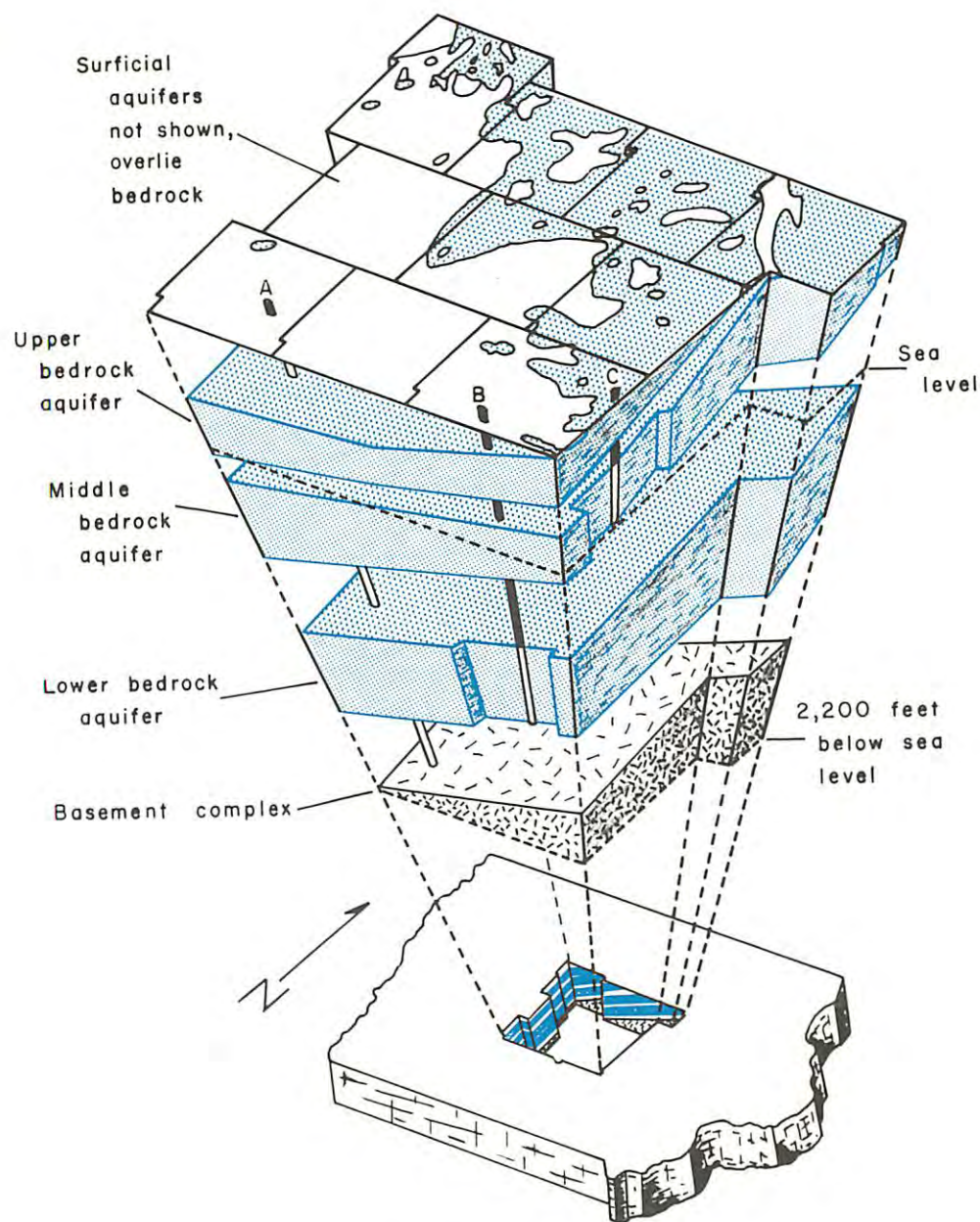
The aquifers and how they occur.
