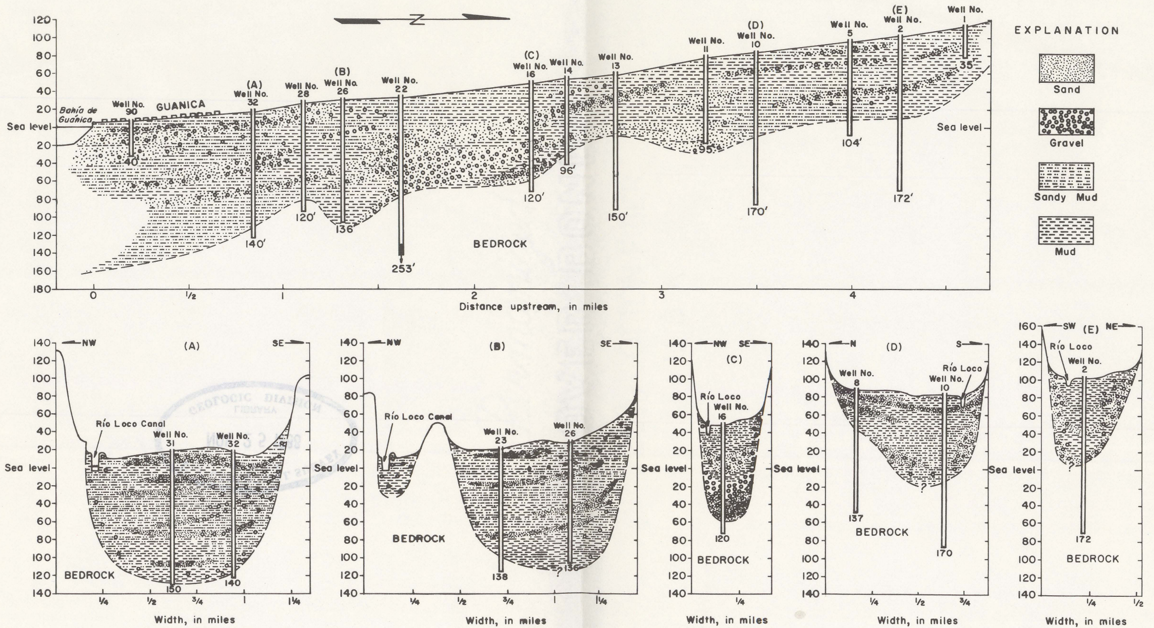
Figure 7.-- Interpretive sections of alluvium along lower Rio Loco valley.
