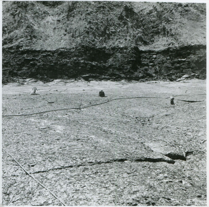
Floor of Makaopuli lava lake 8/13/65
