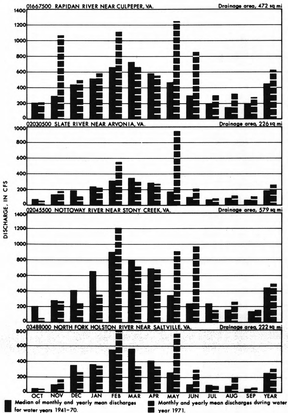
Figure 1. Runoff during 1971 water year compared with median runoff for period 1941-70 for four representative gaging stations
