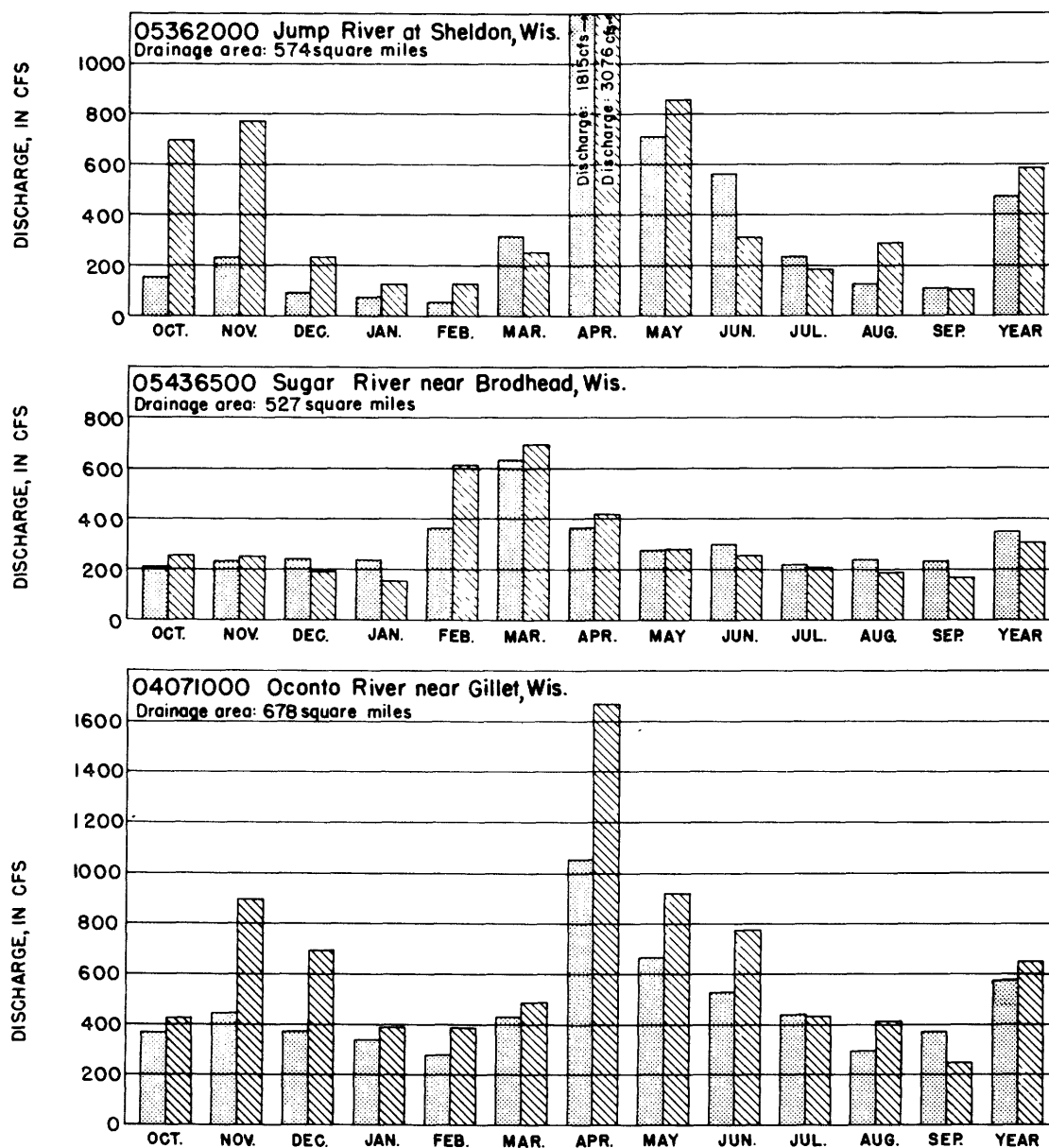
Figure 3. Comparison of discharge at three long-term representative gaging stations during 1971 water year with median discharge for period 1931-60.
