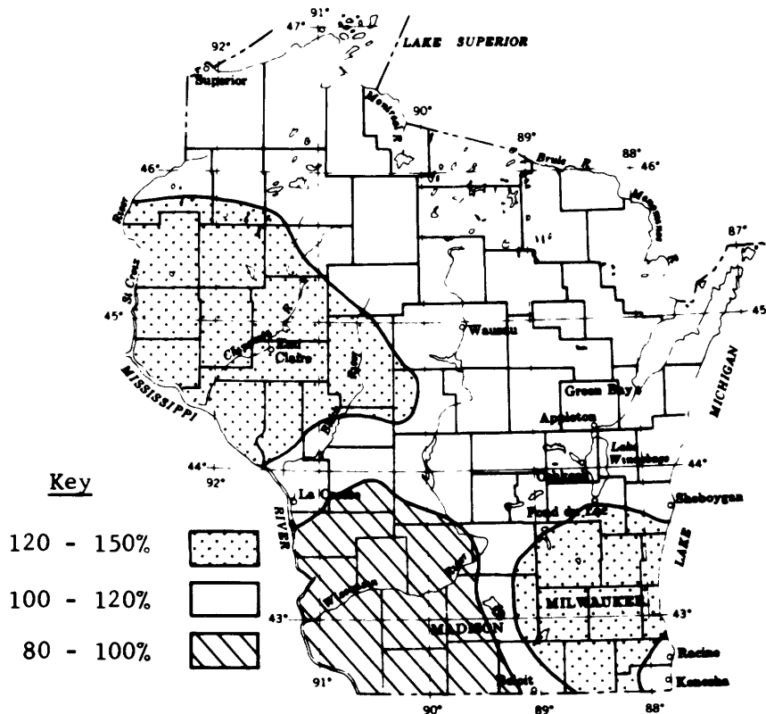
Figure 2. Variation of the 1971 runoff compared with the long-term average runoff.
