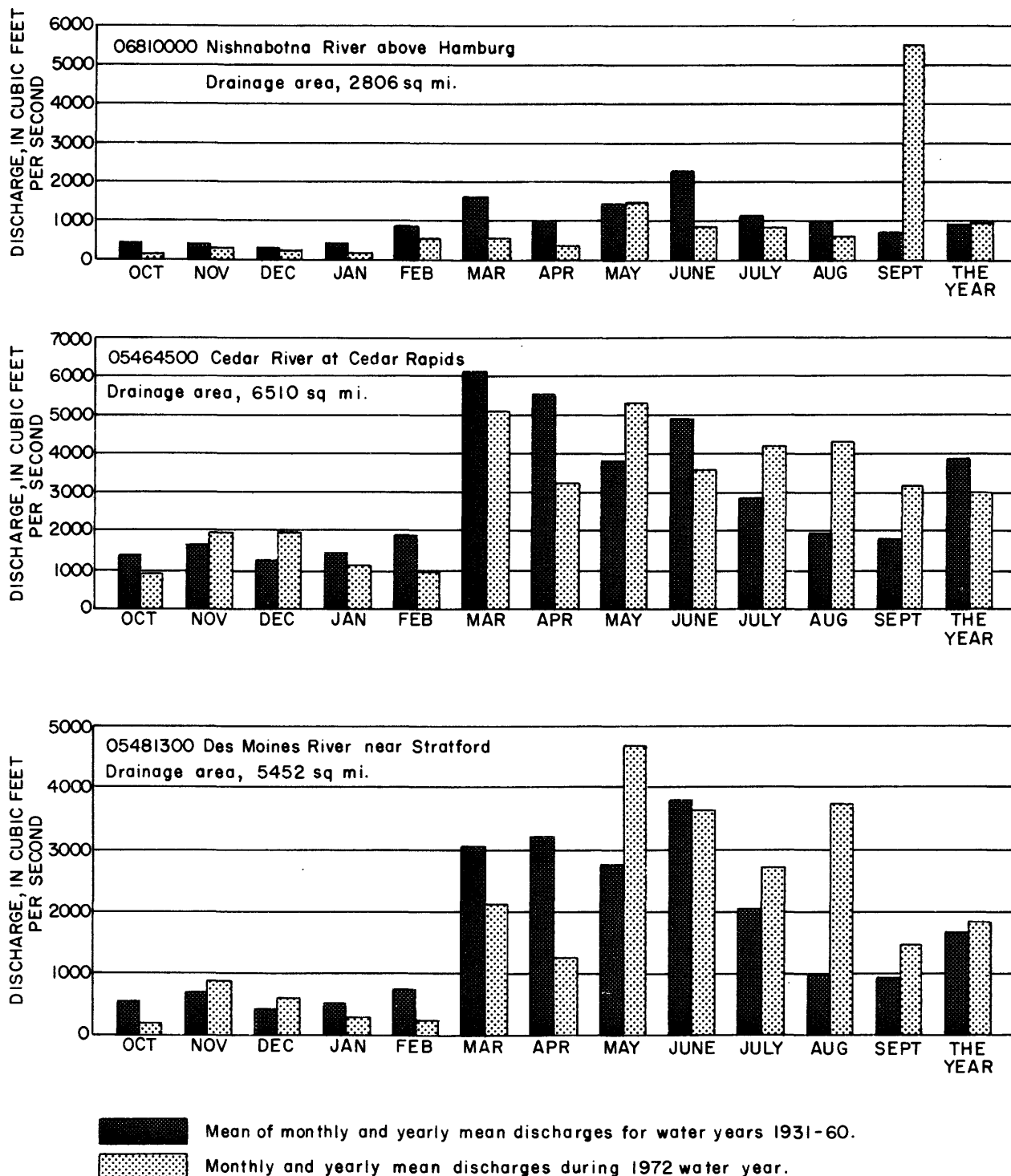
FIGURE 3.-- RUNOFF DURING 1972 WATER YEAR COMPARED WITH MEAN RUNOFF FOR PERIOD 1931-60 FOR THREE REPRESENTATIVE GAGING STATIONS
