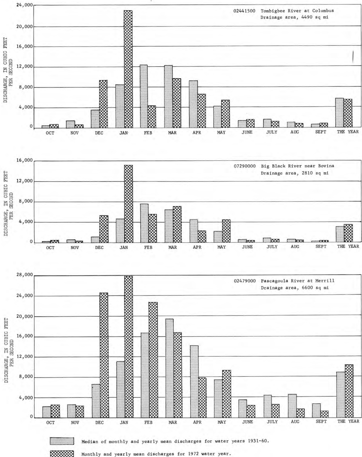
FIGURE 3.--COMPARISON OF DISCHARGE AT THREE LONG-TERM REPRESENTATIVE GAGING STATIONS DURING 1972 WATER YEAR WITH MEDIAN DISCHARGE FOR PERIOD 1931-60.
