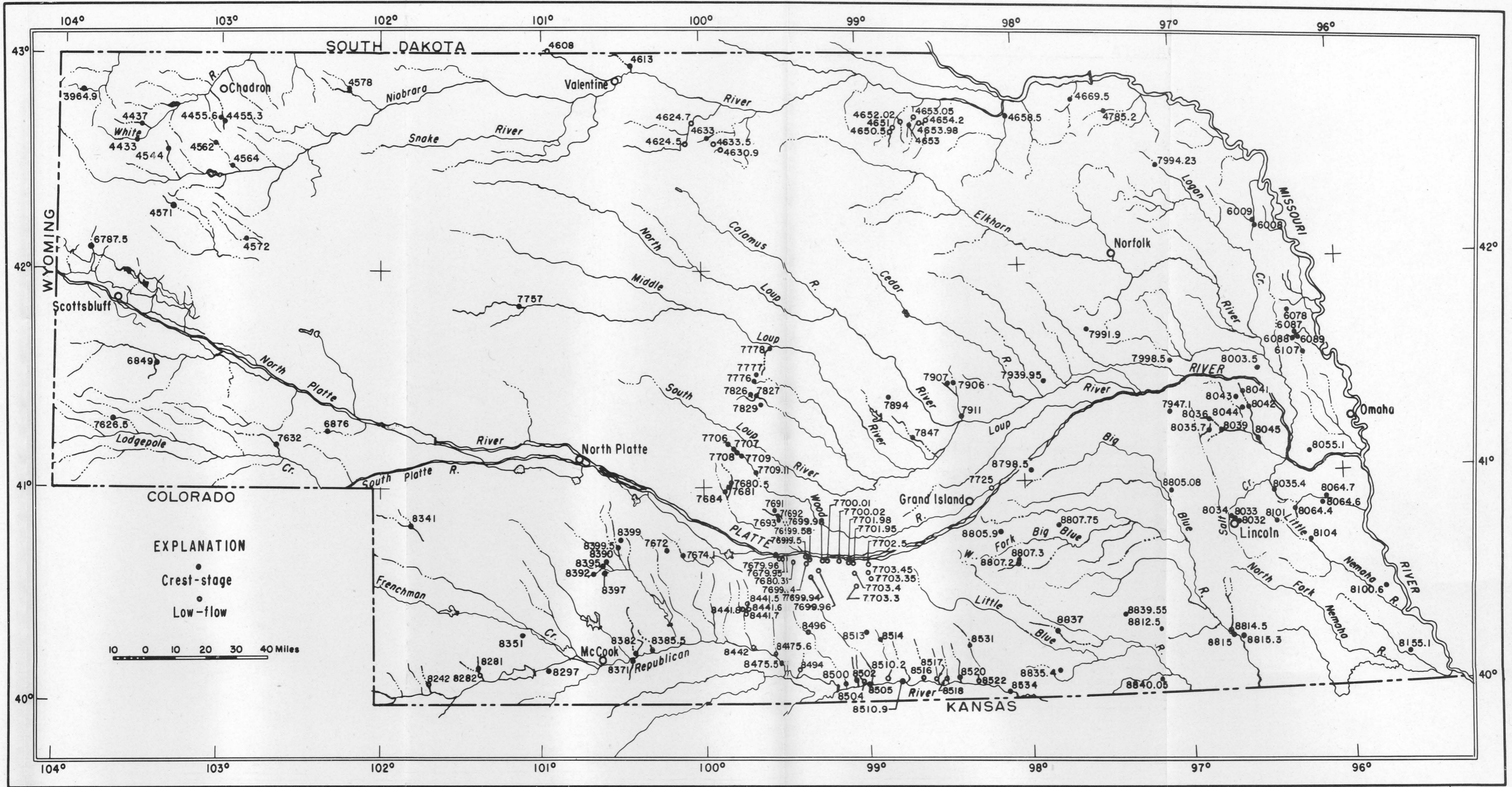
Figure 2.--Map of Nebraska showing location of partial-record stations.
