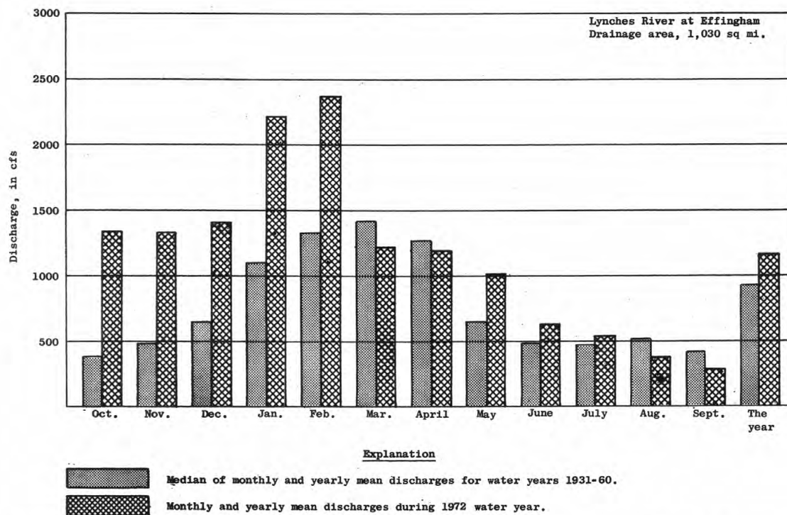
Figure 3. Comparison of discharge at one long-term representative gaging station during 1972 water year with median discharge for water years 1931-60.
