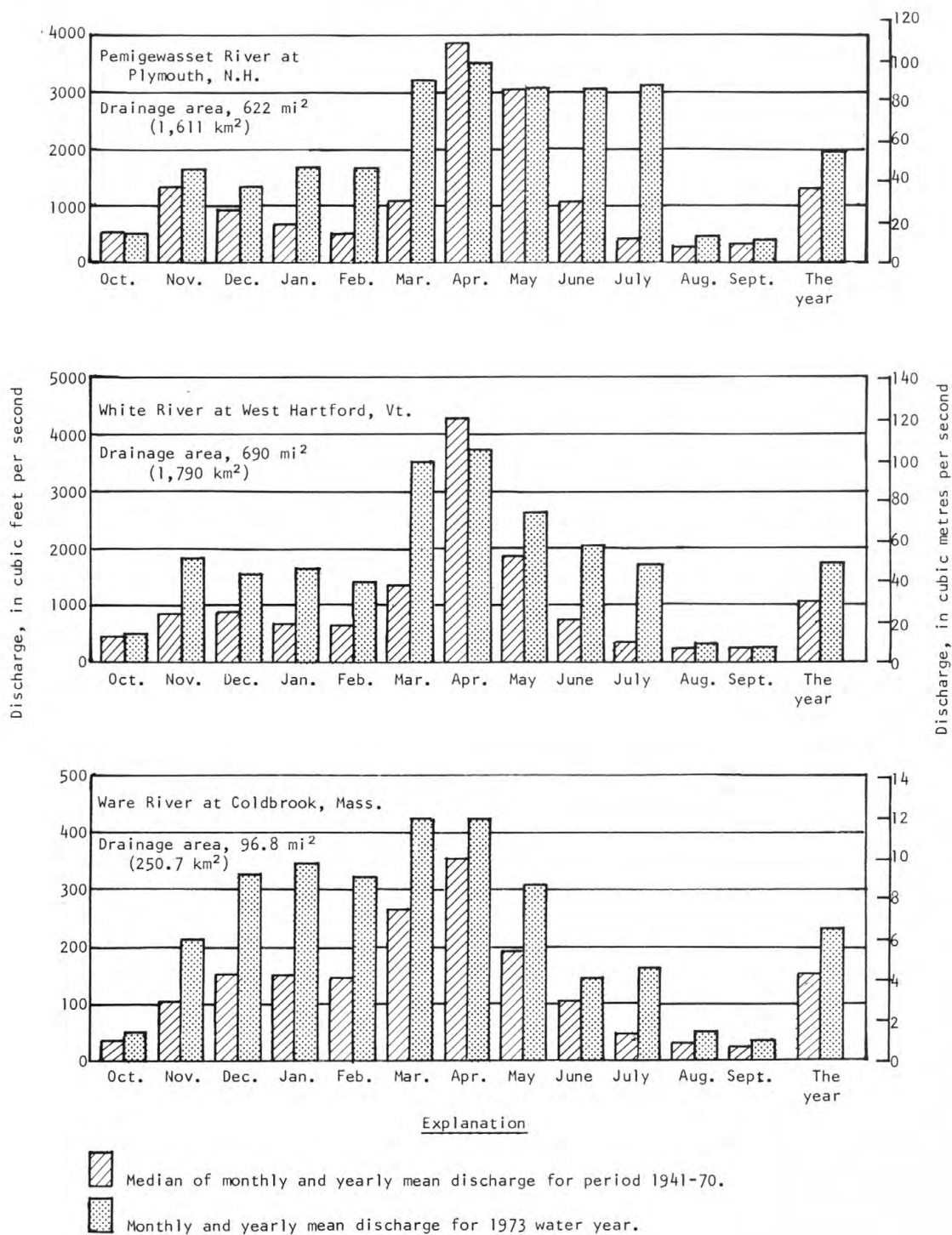
Figure 1.--Comparison of discharge at three long-term index gaging stations during 1973 water year with median discharge for period 1941-70.
