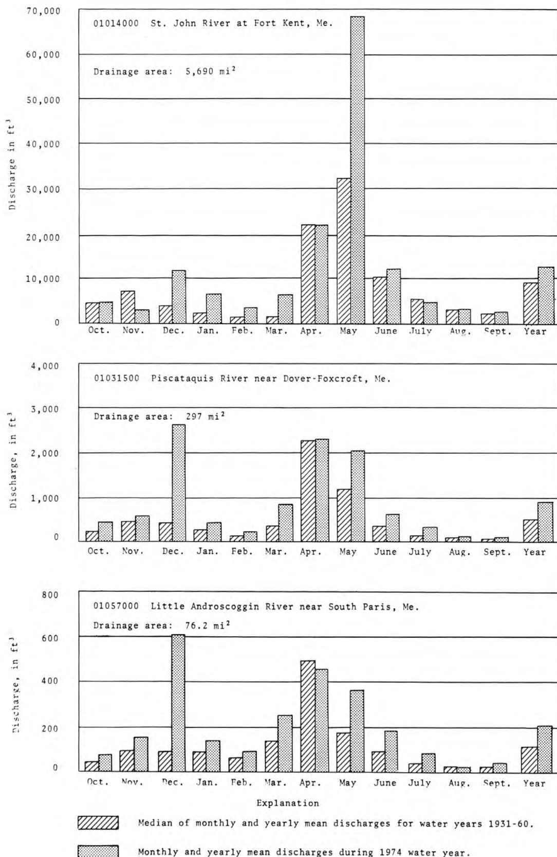
Figure 1.--Comparison of runoff at three long-term index gaging stations during 1974 water year with median runoff for period 1931-60.
