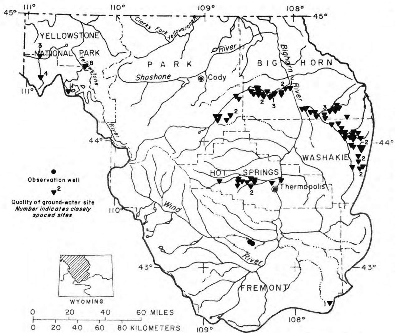
Figure 7.—Location of observation wells and quality of ground-water sites in the Yellowstone River, Clarks Fork Yellowstone River, and Bighorn River basins.
