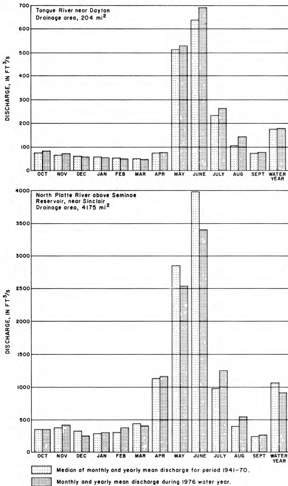
Figure 3.—Discharge during 1976 water year compared with median discharge for period 1941-70 for two representative gaging stations.
