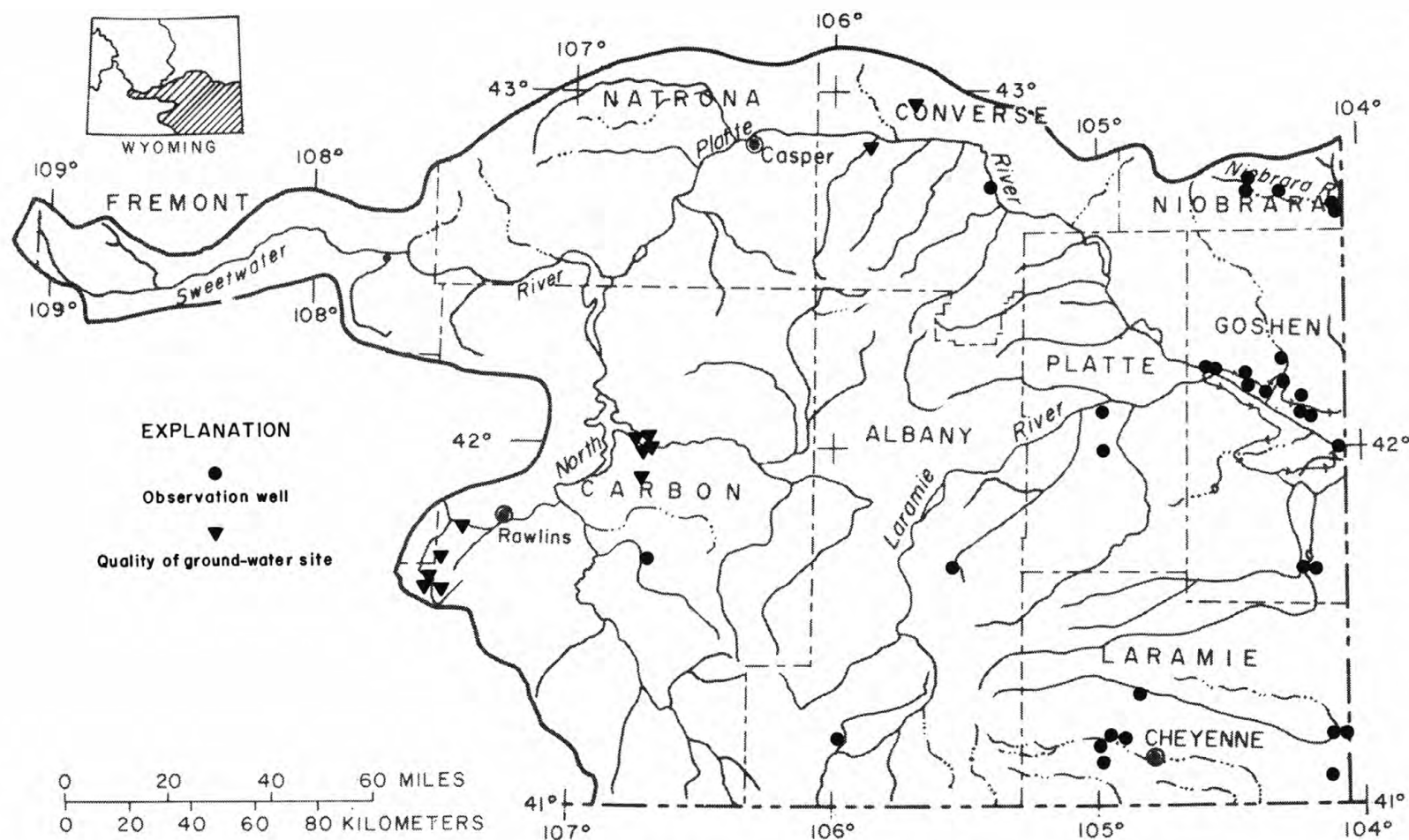
Figure 9.—Location of observation wells and quality of ground-water sites in the Niobrara River and Platte River basins.
