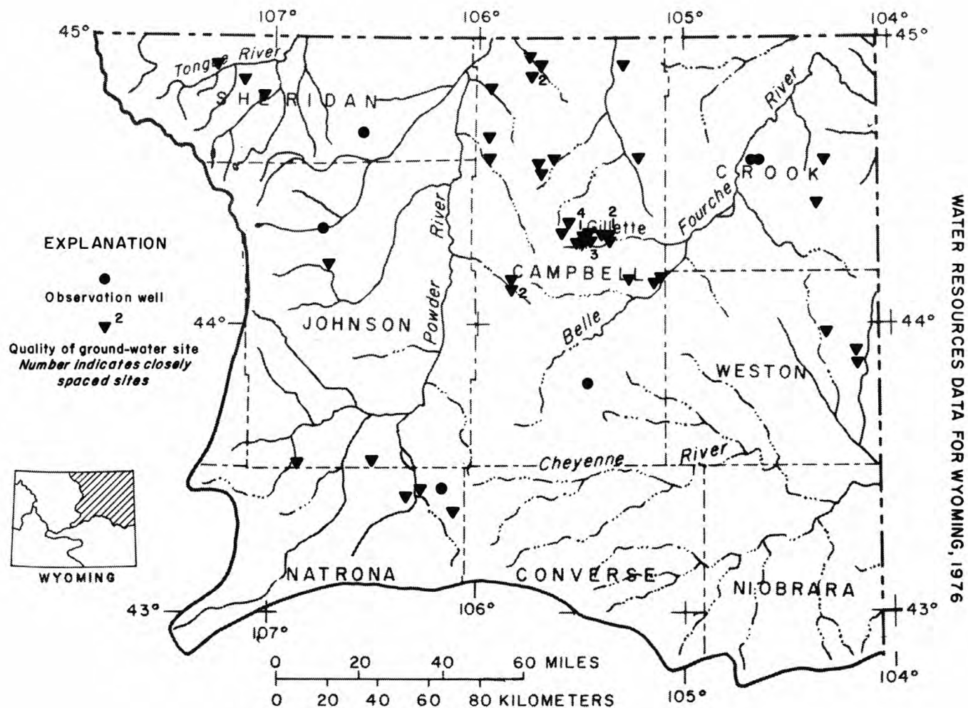
Figure 8.—Location of observation wells and quality of ground-water sites in the Tongue River, Powder River, Belle Fourche River, and Cheyenne River basins.
