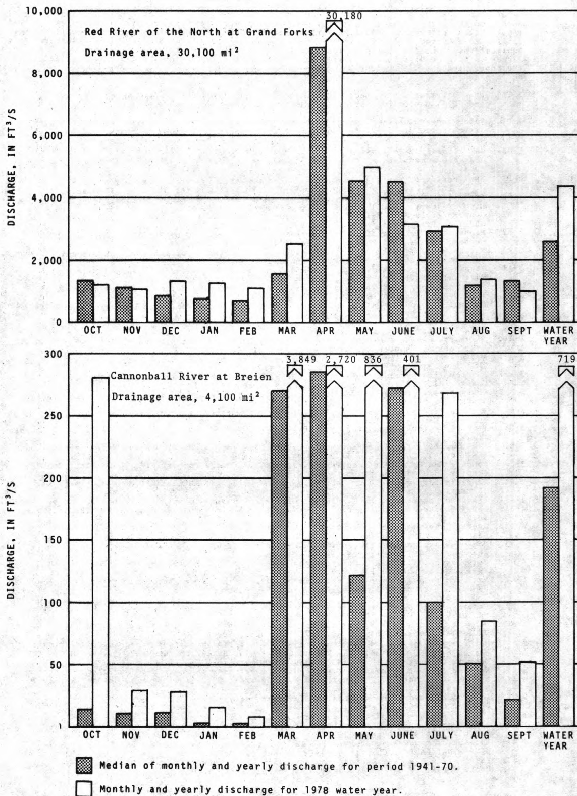
FIGURE 3.--Discharge during 1978 water year compared with median discharge for period 1941-70 for two representative gaging stations.
