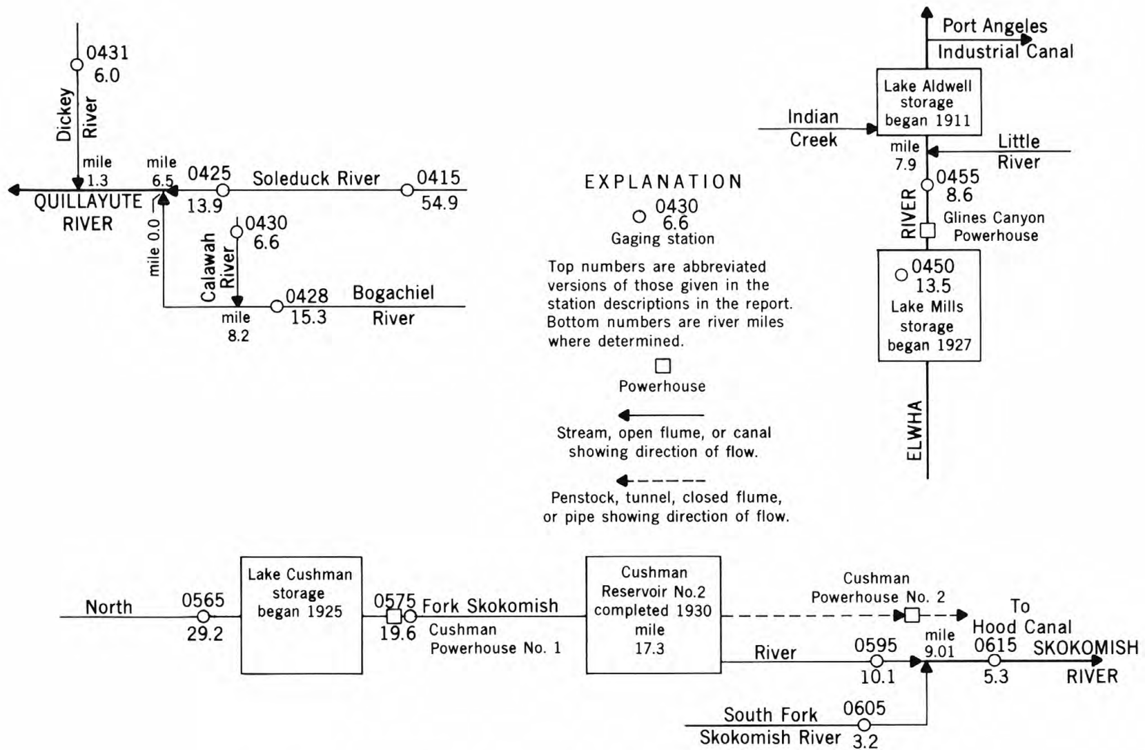
Figure 8. Gaging stations in Quillayute, Elwha, and Skokomish River basins.
