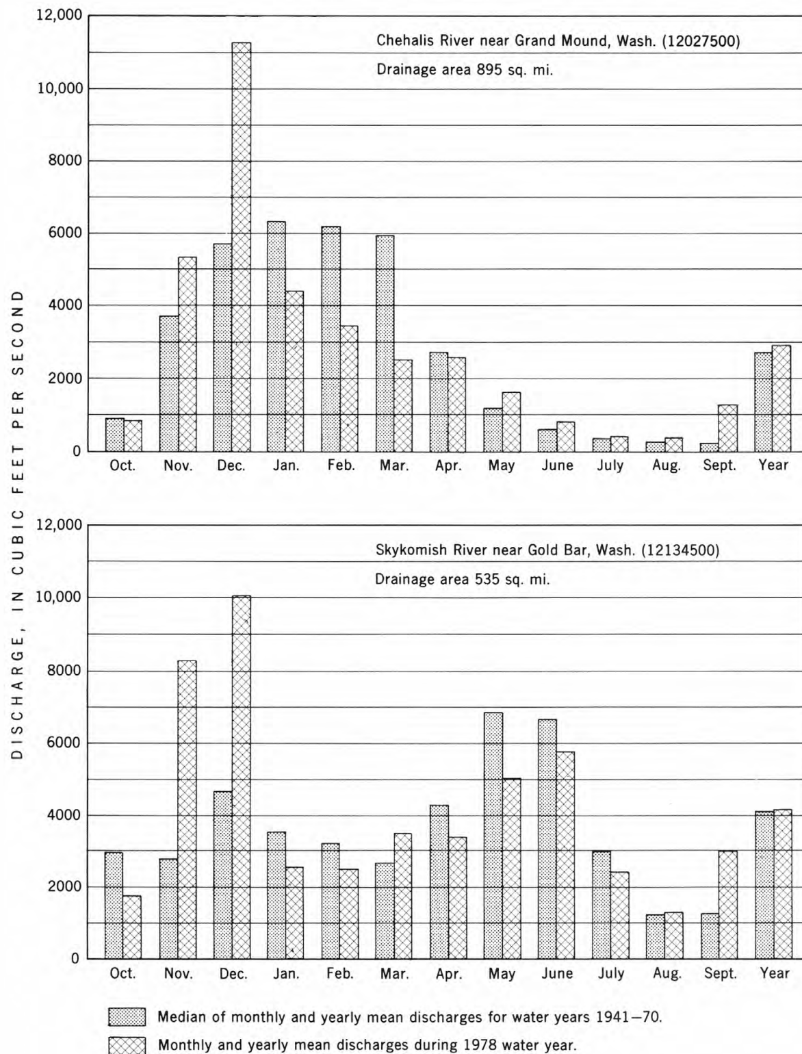
Figure 3. Discharge during 1978 water year compared with median discharge for period 1941-70 for two representative gaging stations.
