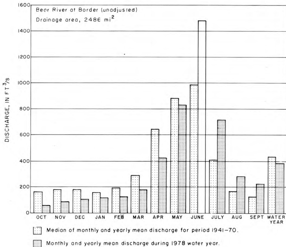
Figure 3.—Discharge during 1978 water year compared with median discharge for period 1941-70 for two representative gaging stations.
