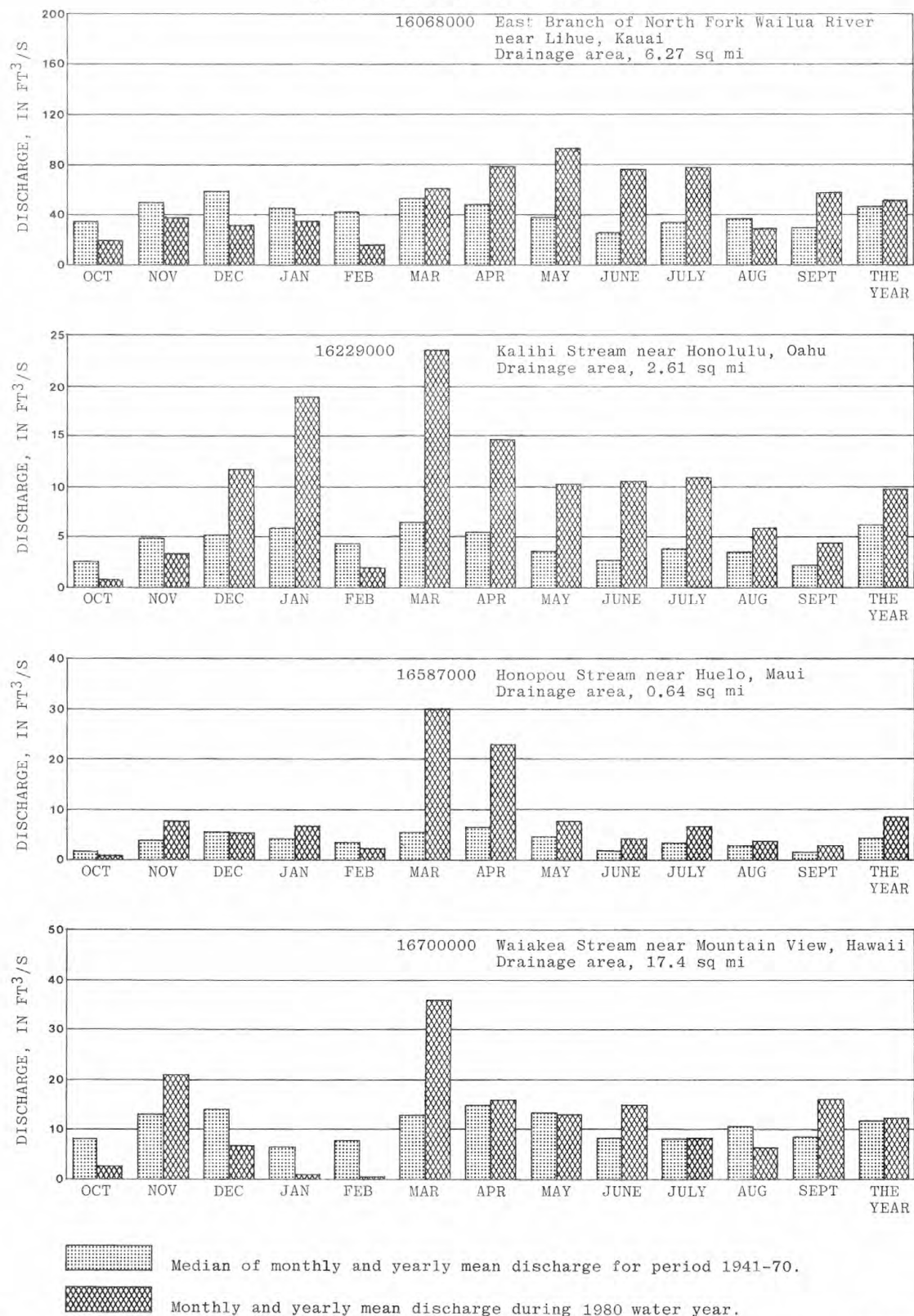
FIGURE 1.--DISCHARGE DURING 1980 WATER YEAR COMPARED WITH MEDIAN DISCHARGE FOR PERIOD 1941-70 FOR FOUR REPRESENTATIVE GAGING STATIONS.
