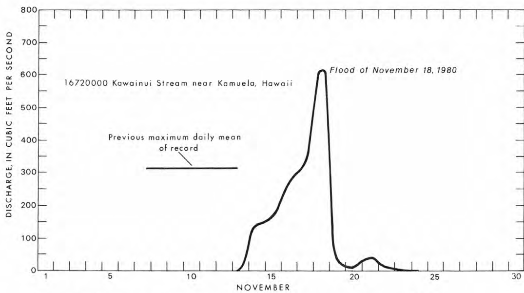
FIGURE 2.--DISCHARGE AT SELECTED GAGING STATIONS, FLOODS OF NOVEMBER 17-18.
