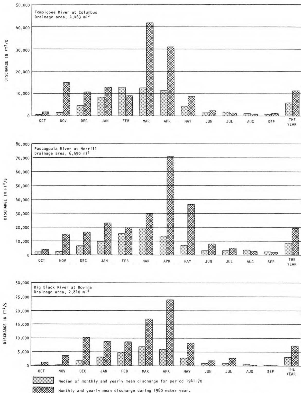
FIGURE 2.--Discharge during 1980 water year compared with median discharge for period 1941-70 for three representative gaging stations.
