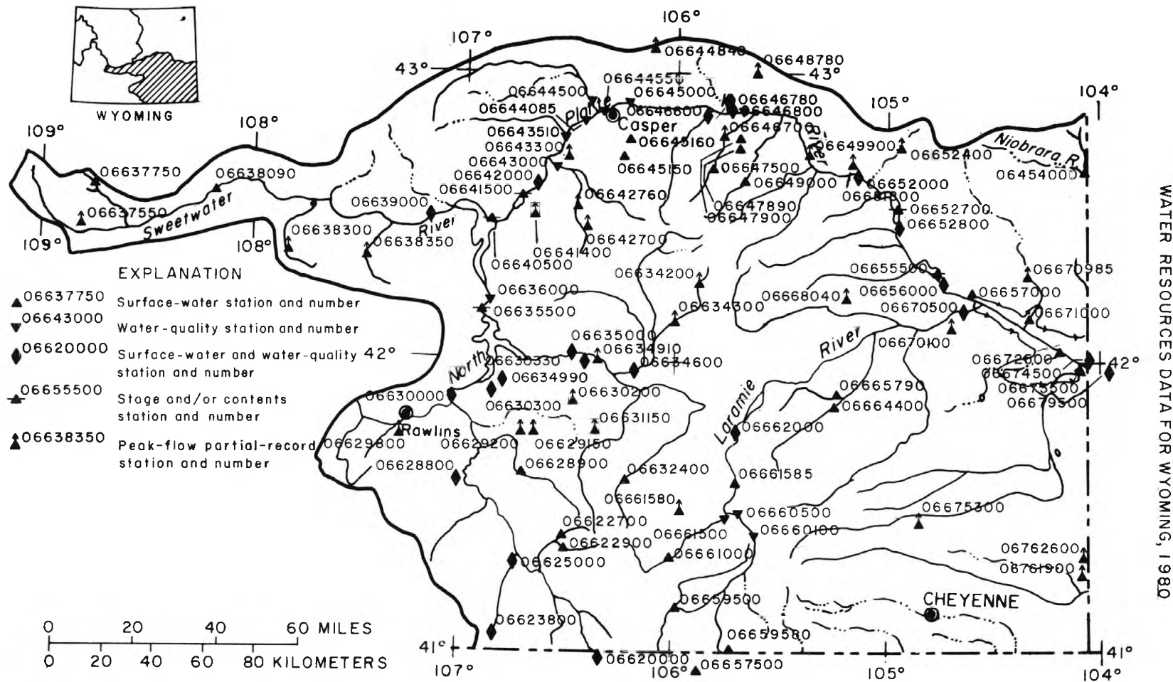
Figure 6.—Location of gaging stations and peak-flow partial-record stations in the Niobrara River and Platte River basins.
