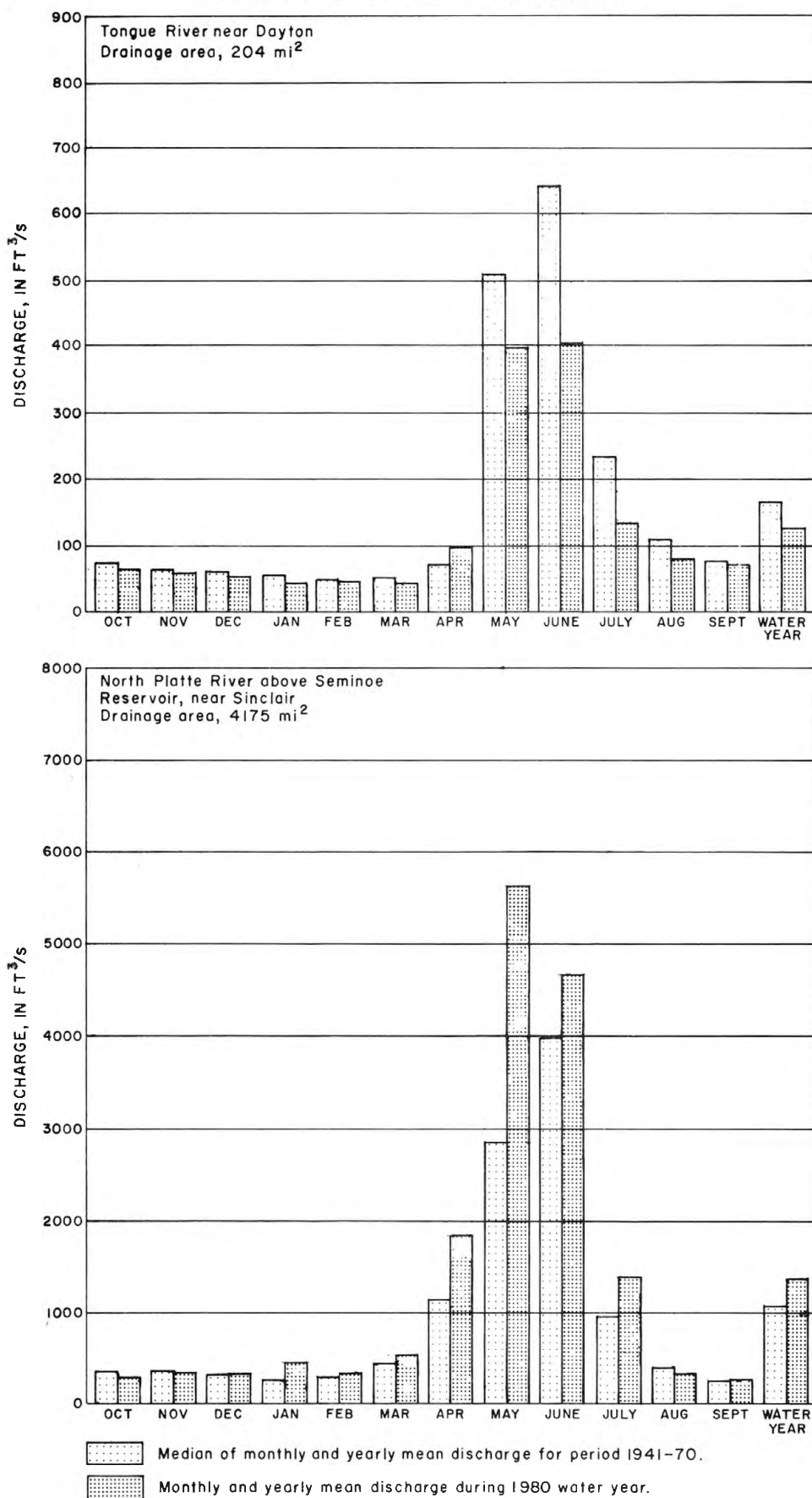
Figure 3.—Discharge during 1980 water year compared with median discharge for period 1941-70 for two representative gaging stations.
